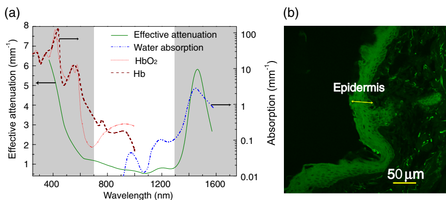
Fig. 2 (a) Optical effective attenuation spectrum of living skin tissue (solid green line) dominated by water ( \text{H}_2\text{O} , blue “- - -” line), hemoglobin (Hb, brown “-” line), oxy-hemoglobin ( \text{HbO}_2 , red solid “-” line), proteins (not shown), with the scattering effect taken into account. Biological tissue transparency window ranges from 700 to 1300 nm, visualized as clear area against the gray-shaded area. Calculated based on the published data. 33 (b) Autofluorescence image of human skin under the excitation at 405 nm. The viable epidermis layer is color-coded green and marked by an arrow, with cell nuclei are visible as dark ovals. Dermis, visualized primarily via collagen and elastin bundles, is adjacent to the epidermis extending to the right.
