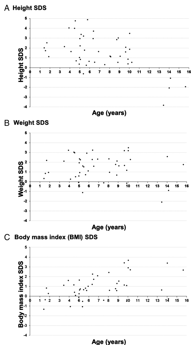
Figure 1 SD scores (SDS) for height and weight at first presentation with congenital adrenal hyperplasia for children over 1 year of age (n=44). (A) Height SDS. (B) Weight SDS. (C) Body mass index (BMI) SDS.
