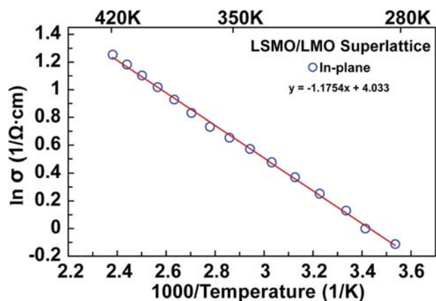
FIG. 9. The in-plane LSMO/LMO superlattices electrical conductivity fitting plot to extract the effective thermal activation energy of 101 \pm 5 meV.
