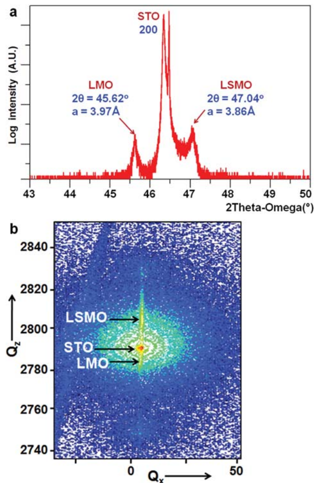
FIG. 2. (a) XRD 2-theta-omega scan of an LSMO/LMO superlattice on a STO (100) substrate confirming c-axis epitaxial behavior with LSMO FWHM ( 0.027^\circ ) and LMO FWHM ( 0.102^\circ ) and (b) 110 RSM of a micron-thick LSMO/LMO superlattice. The LSMO and LMO peaks have a small degree of spread and show a consistent in-plane lattice parameter, confirming the pseudomorphic epitaxial growth of the superlattice film.
