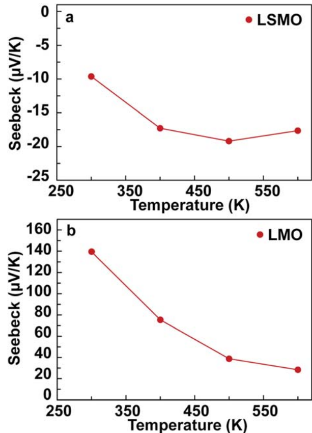
FIG. 6. (a) In-plane Seebeck measurement of LSMO shows Seebeck coefficient consistent with metallic behavior with a magnitude of less than 20 \mu\text{V}/\text{K} and (b) in-plane Seebeck measurement of LMO validating p-type behavior with a room temperature Seebeck coefficient of 140 \pm 3 \mu\text{V}/\text{K} .
