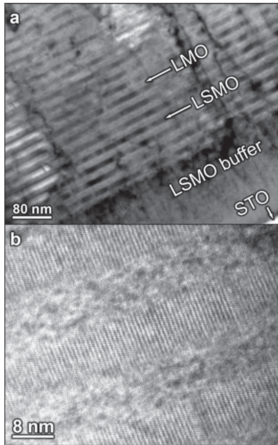
FIG. 3. (a) Low-magnification cross-sectional bright field TEM images of an LSMO (8 nm)/LMO (8 nm) superlattice and (b) high-resolution cross-section TEM confirming epitaxial layer contrast of LSMO/LMO superlattices on a STO (100) substrate were taken using FEI Titan operating at 300 kV. The contrast in (a) along the normal to the growth surface is due to threading dislocations.
