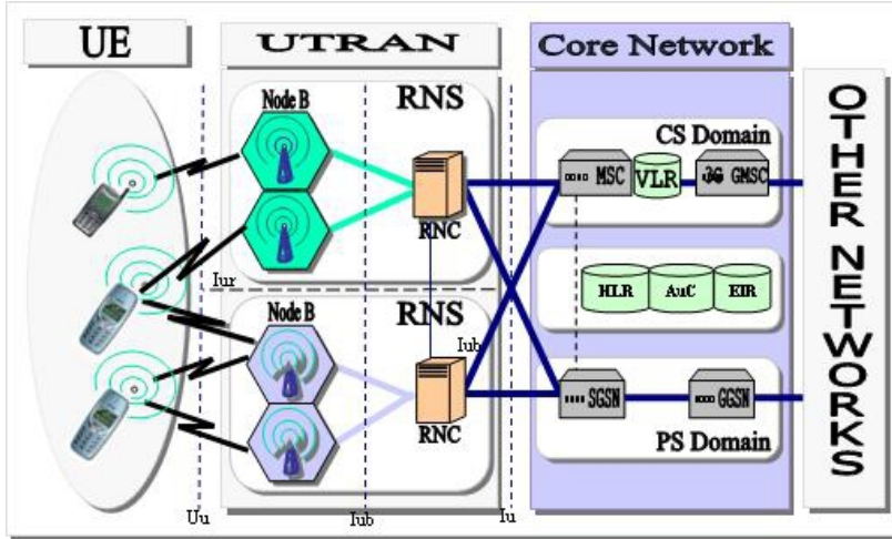
Fig. 2 UMTS Architecture
