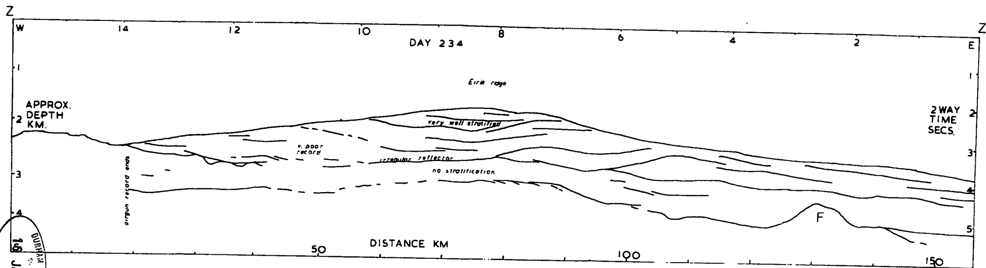
Fig. 5.5 Airgun profile line drawing interpretation across the Eirik ridge, Z-Z' located on fig. 5.3 showing sediment structure. Basement high F is interpreted as a continuation of the Farewell fracture zone.
