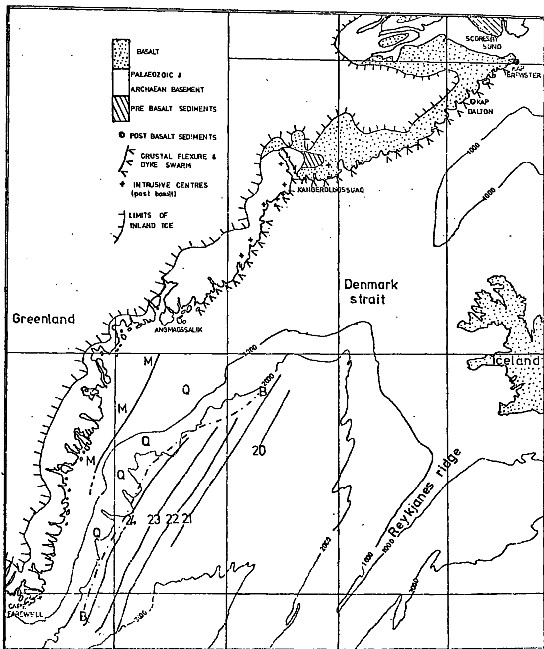
Fig. 4.5 Sketch map showing the relationship of the magnetic anomalies with the extrusives on land, anomalies as in fig. 4.1, geology after Wager (1934) and Escher et al. (1970).
