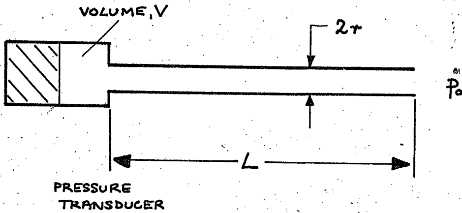
FIGURE 3.17 : IDEALISED PRESSURE MEASURING SYSTEM
