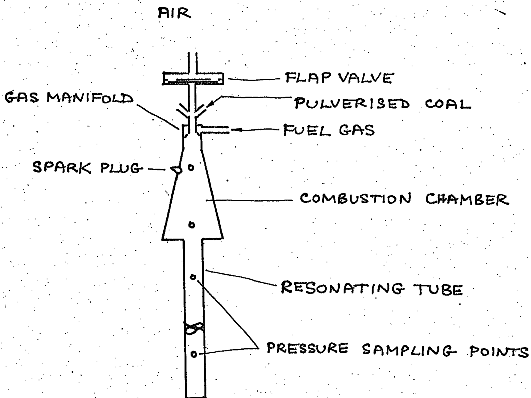
FIGURE 1.16: PULSATING COMBUSTOR OF HANBY & BROWN
