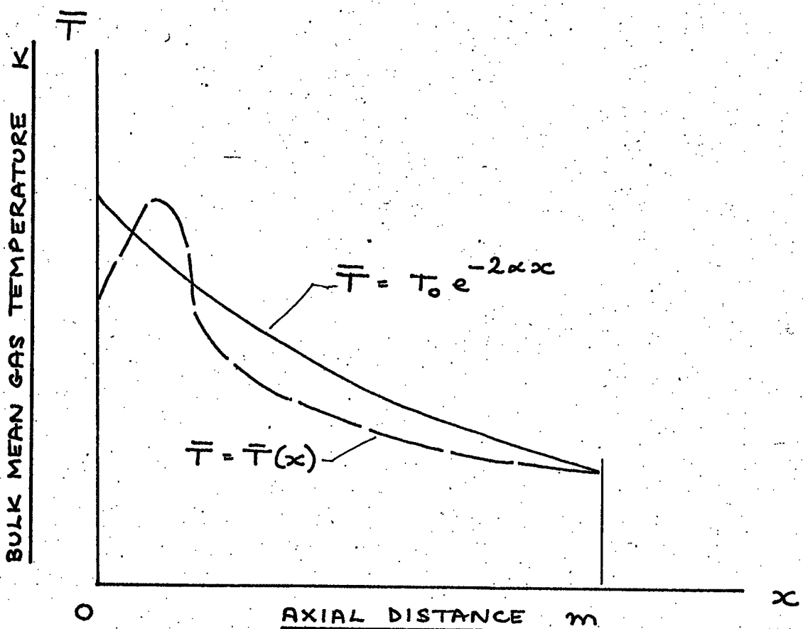
FIGURE 2.2 : EXPONENTIAL AND GENERAL VARIATIONS OF GAS TEMPERATURE ALONG TUBE
