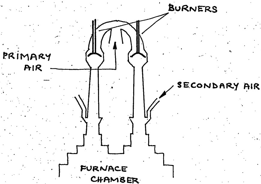
FIGURE 1.14 : COUNTER-PHASE PULSATING COMBUSTOR
