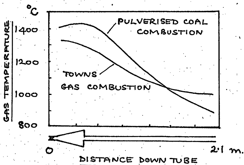
FIGURE 1.17: GAS TEMPERATURE DISTRIBUTION
