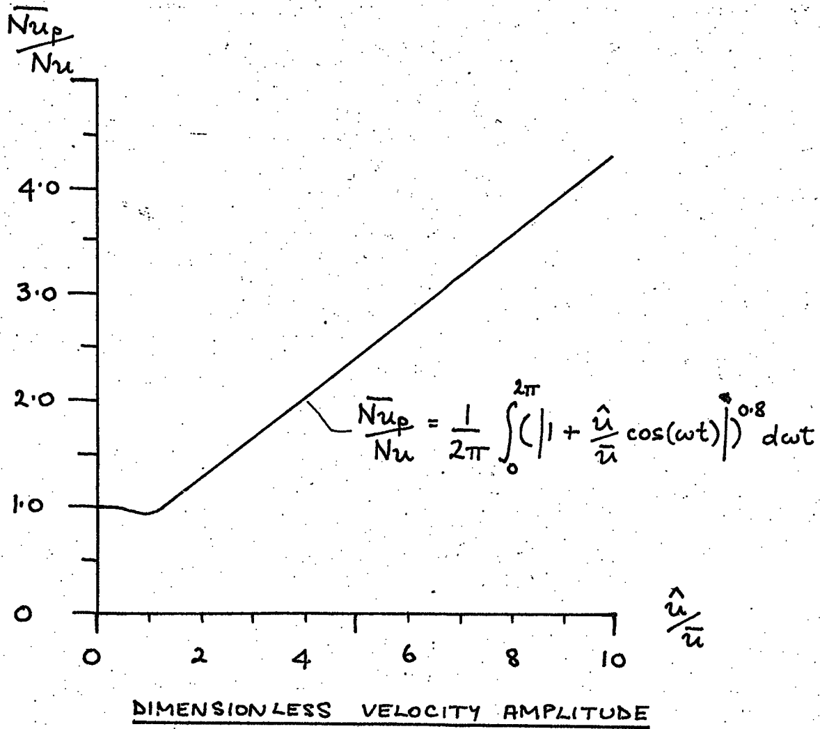
FIGURE 2.6 : QUASI-STEADY STATE THEORY
