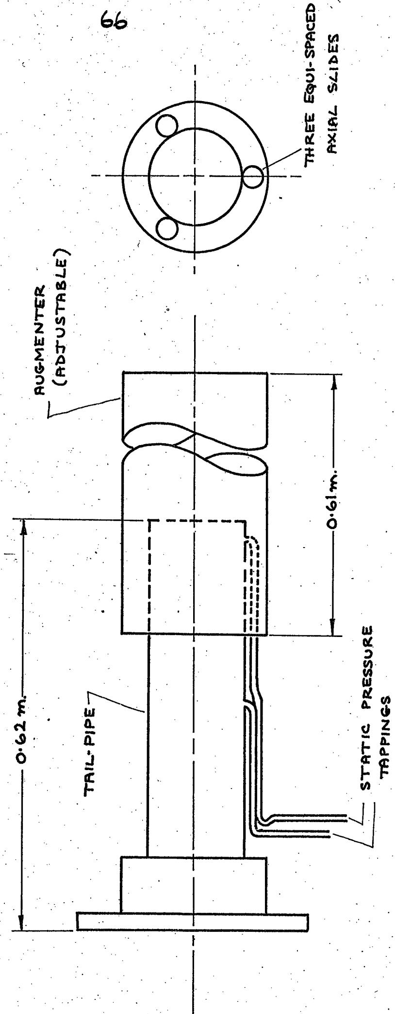
FIGURE 3.6 : TAIL-PIPE AND AUG-MENTER
