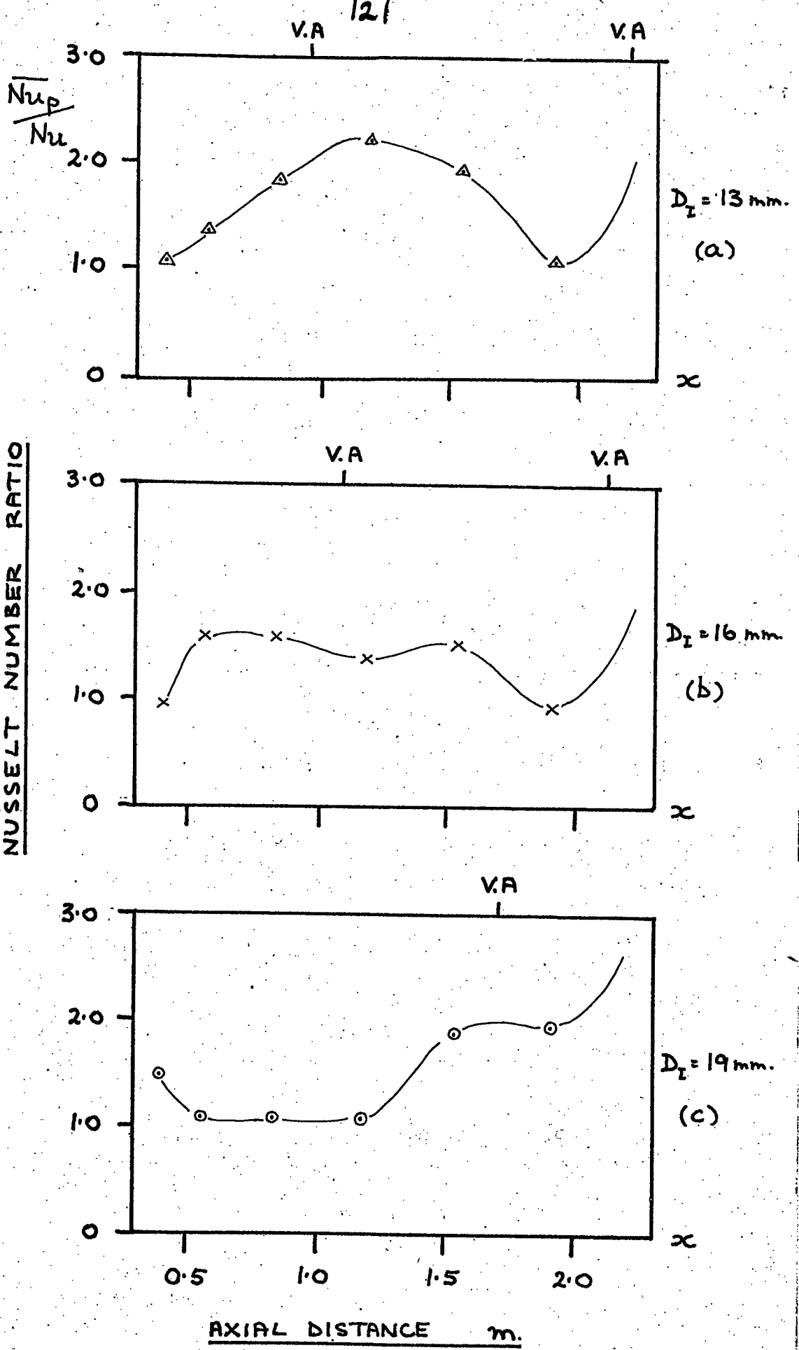
FIGURE 4.24: GRAPHS OF NUSSELT NUMBER RATIO AGAINST DISTANCE IN HEAT EXCHANGER A FOR D_I = 13, 16 + 19 \text{ mm.}
