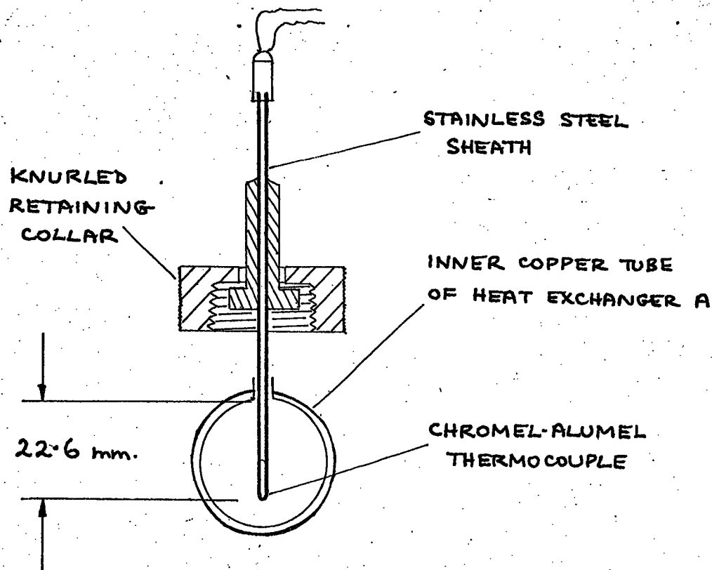
FIGURE 3.11 : GAS TEMPERATURE THERMOCOUPLE - TYPE K
