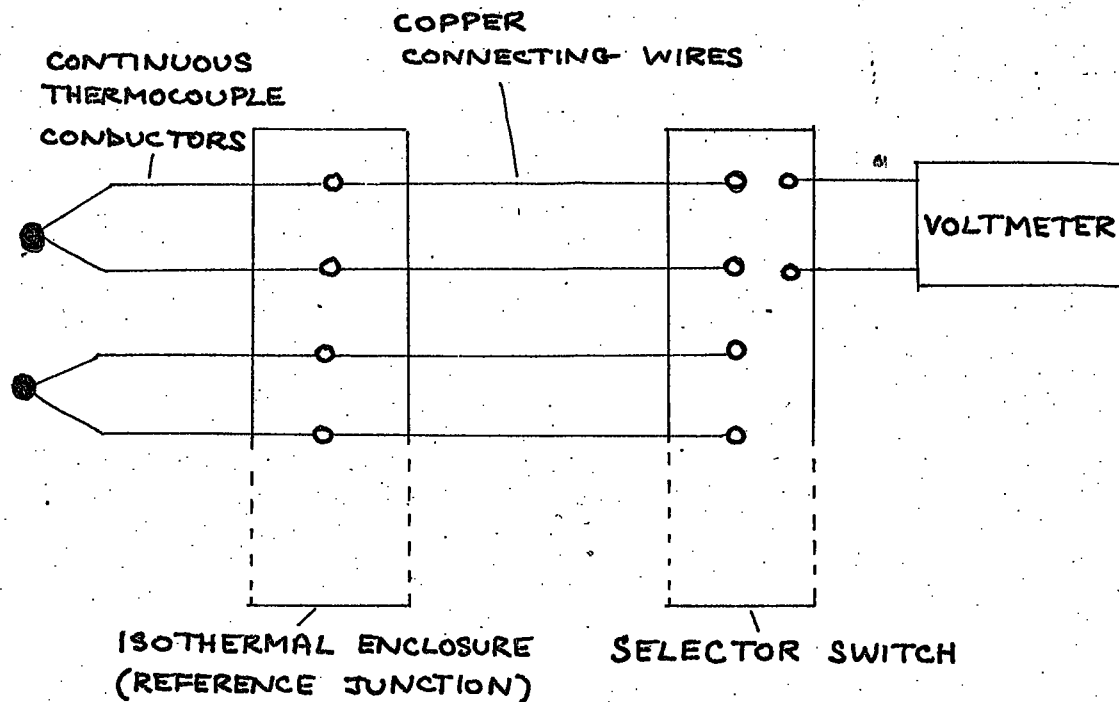
FIGURE 3.10 : THERMOCOUPLE CIRCUIT
