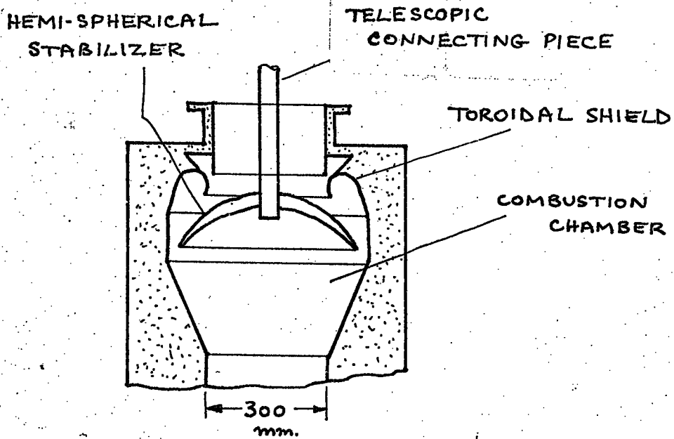
FIGURE 1.13 : AERODYNAMIC VALVE OF BABKIN
