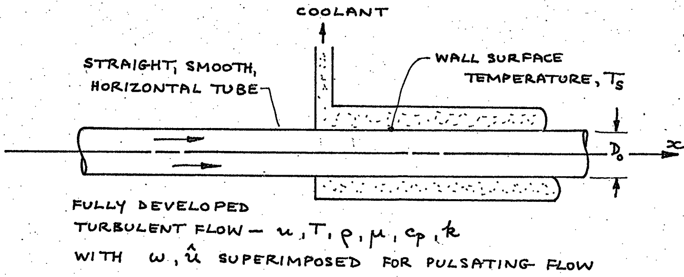
FIGURE 2.5: PARAMETERS OF THE FLOW
