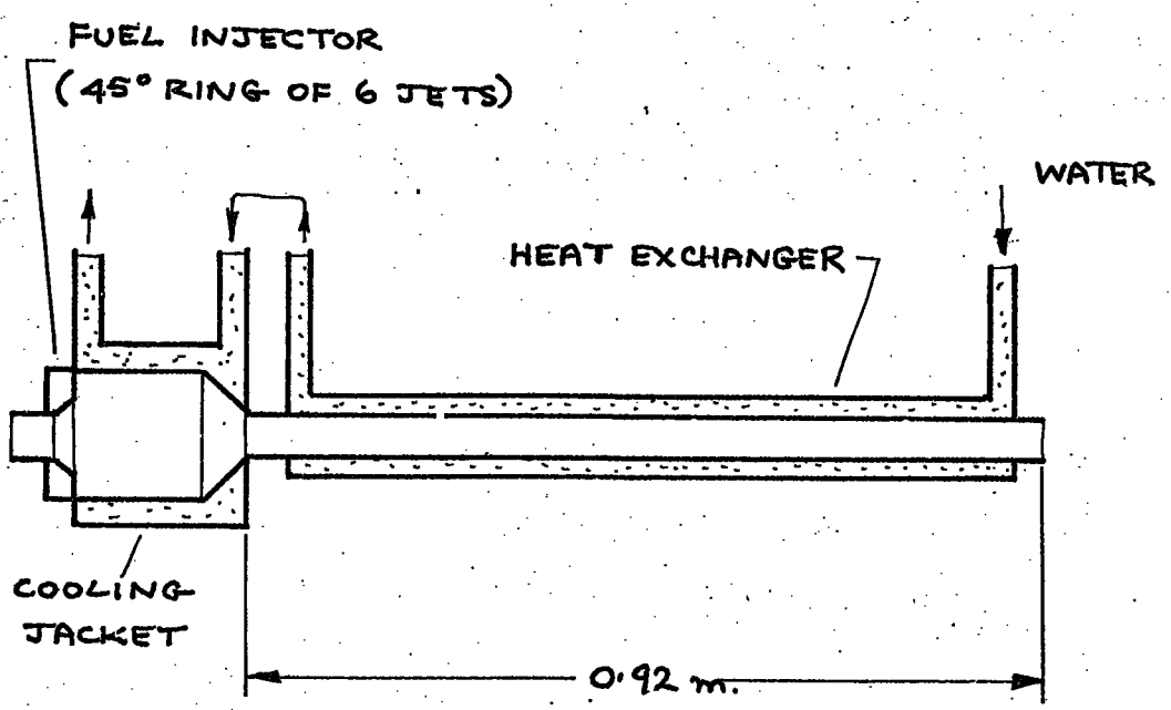
FIGURE B.2 : FIRST COMBUSTION CHAMBER WITH HEAT EXCHANGER, COOLING JACKET AND MODIFIED FUEL INJECTION
