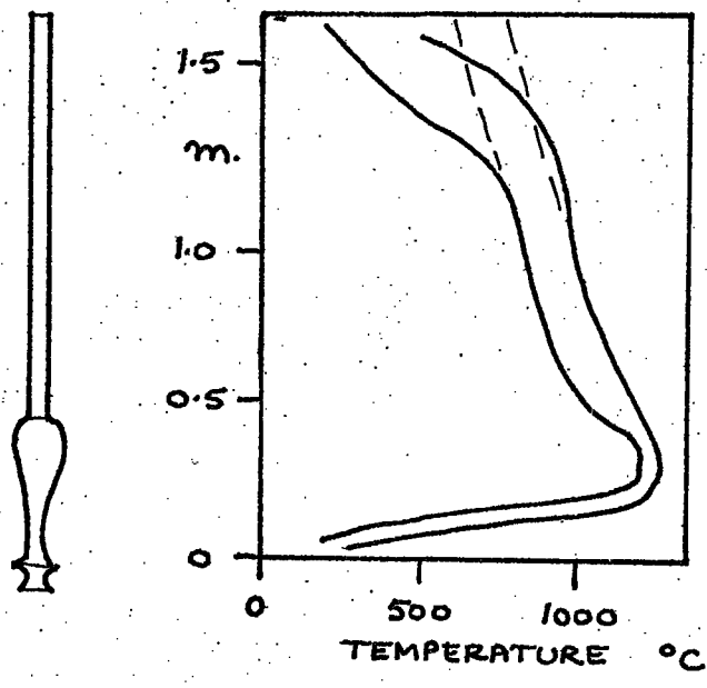
FIGURE 1.9 : GAS TEMPERATURE DISTRIBUTION IN PULSATING COMBUSTOR
