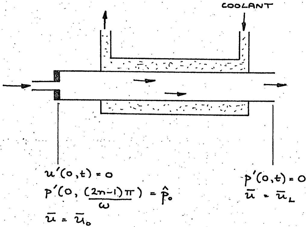
FIGURE 2.3 : OSCILLATING FLOW OF COMPRESSIBLE FLUID THROUGH SIMPLE HEAT EXCHANGER
