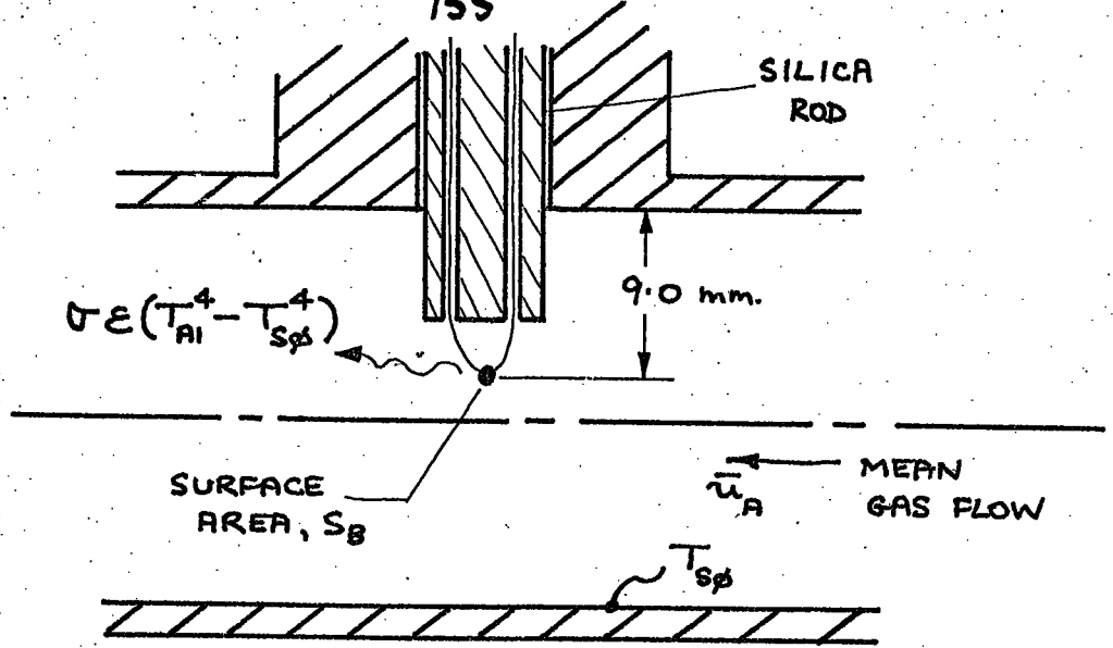
FIGURE C.1: EXAGGERATED T_{AI} INSTALLATION
