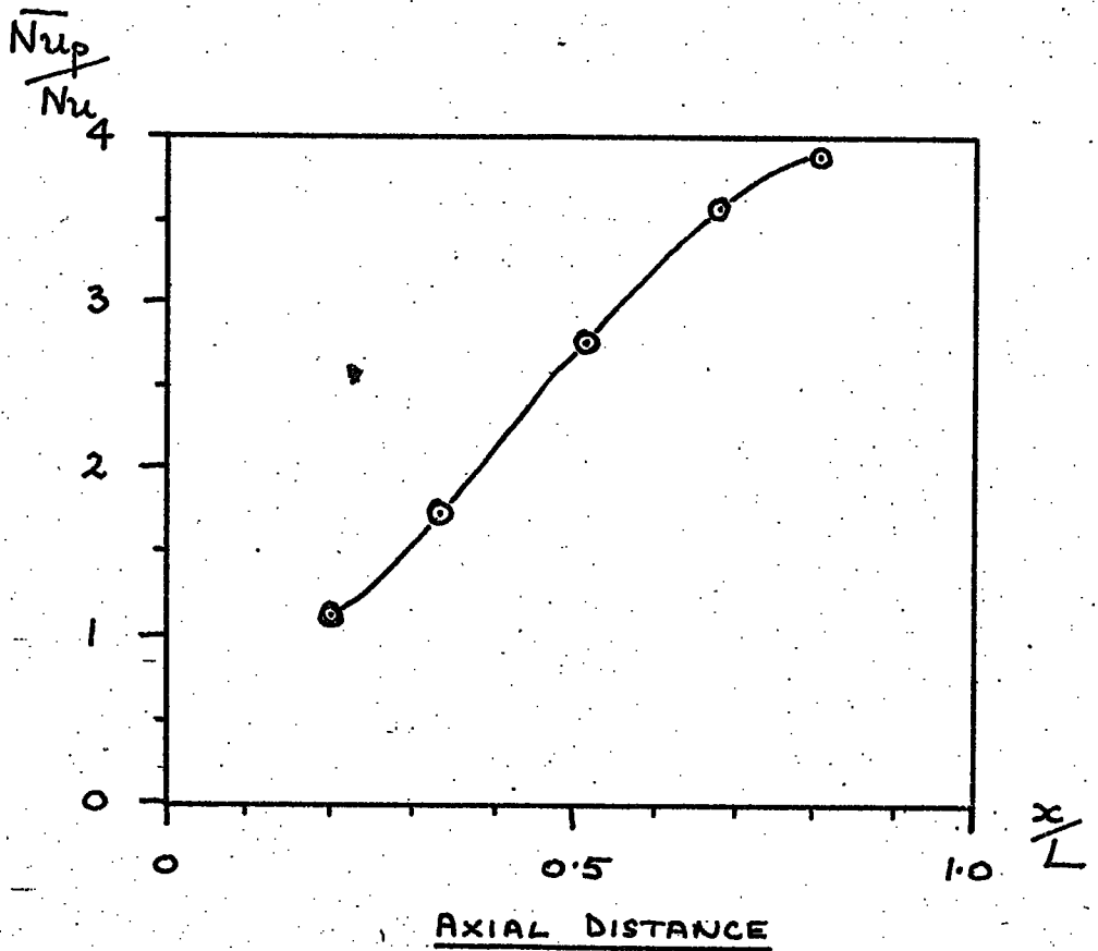
FIGURE 1.22 : GRAPH OF NUSSELT NUMBER RATIO AGAINST DISTANCE FROM HANBY
