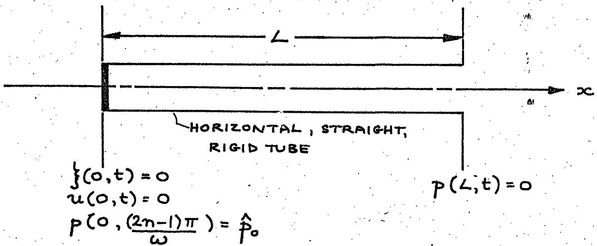
FIGURE 2.1 : BOUNDARY CONDITIONS & CO-ORDINATE SYSTEM FOR ISOTHERMAL FLUID
