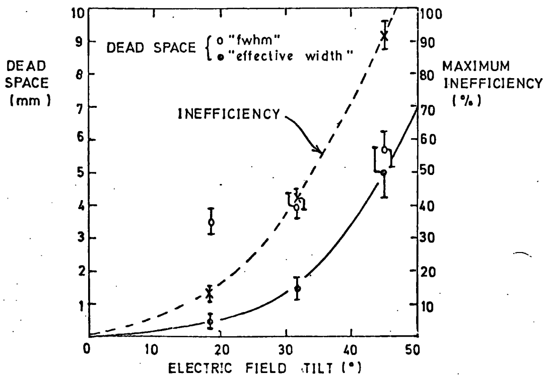
FIG A7: INEFFICIENCIES AND "DEAD SPACES" CAUSED BY TILTED ELECTRIC FIELD CONFIGURATIONS ( B=0 )
