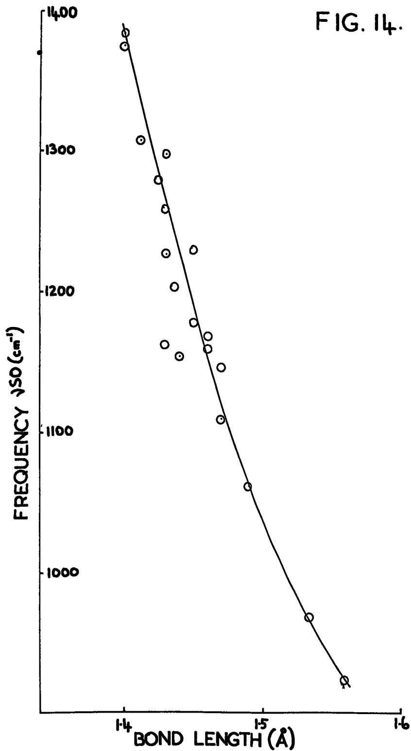
CORRELATION OF S-O STRETCHING FREQUENCY WITH BOND LENGTH 310
