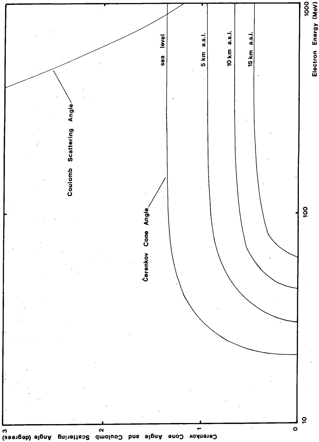
Figure 2.5 Comparison of Cerenkov and Coulomb Effects on Angular Distribution of Light.
