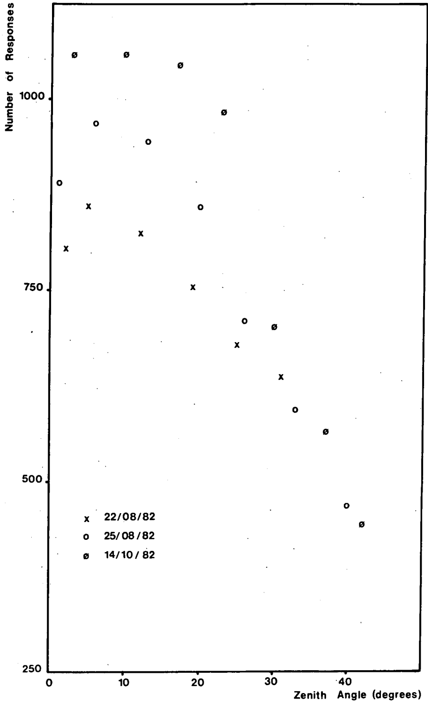
Figure 4.8 Zenith Angle Dependence of Array Response.
