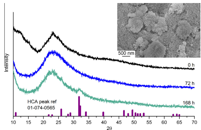
Fig. 9. XRD diffraction pattern for immersion in SBF solution for 0, 72 and 168 h. (Inset) SEM image at 50,000 \times magnification after 2 weeks in SBF for a hybrid of 40 wt.% 60 kDa \gamma CaPGA.
