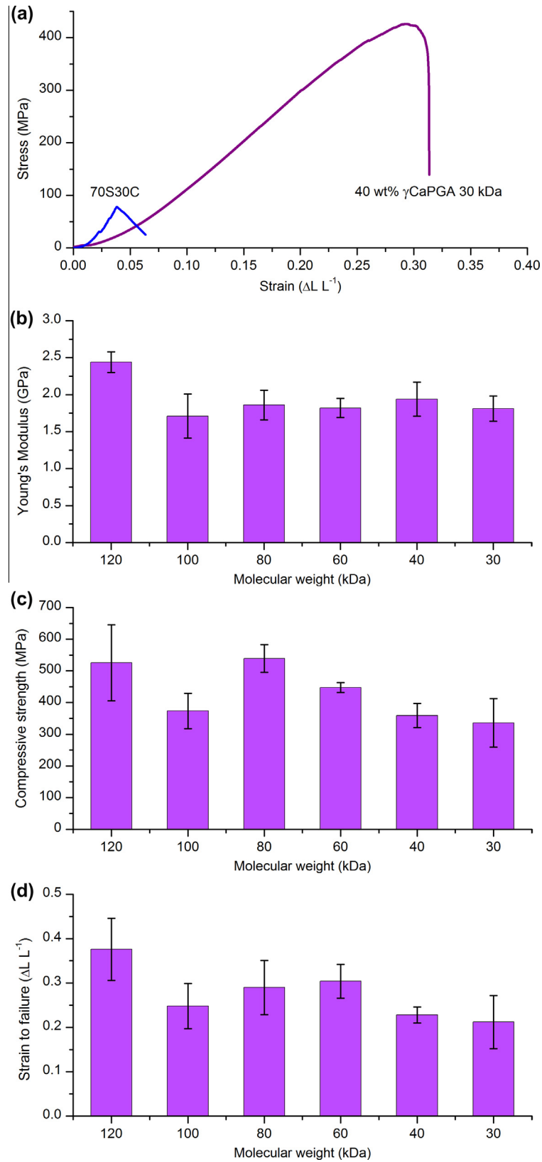
Fig. 10. Compression testing for hybrids of 40 wt.% \gamma CaPGA of varying M_w . (a) Sample stress–strain curve for 30 kDa \gamma PGA hybrid and a sample stress–strain curve for a 70 mol.% SiO_2 , 30 mol.% CaO glass (70S30C). (b) Young's modulus, (c) maximum compressive strength and (d) strain to failure.
