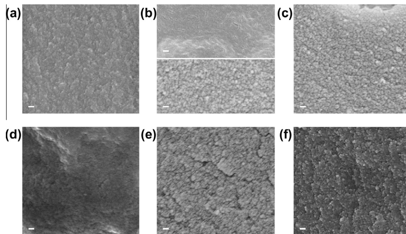
Fig. 7. SEM images of 40 wt.% 120 kDa \gamma\text{CaPGA} hybrid (a) before immersion, (b) after 3 days (2 regions) and (c) 2 weeks immersion in Tris buffer solution. SEM images of 40 wt.% 60 kDa \gamma\text{CaPGA} hybrid (d) before immersion and (e) after 2 weeks immersion in Tris buffer solution. (f) 70S30C glass dried at 40 °C. Scale bar 100 nm.
