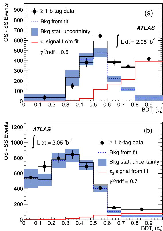
Fig. 2. BDT_j (OS-SS) distributions of \ell + \tau in the \geq 1 b -tag sample; (a) \tau_1 , (b) \tau_3 . The normalisation of each template is derived from a fit to the data. The fitted contributions are shown as the light/red (signal), dashed/blue (background derived from 0 b -tag after applying MC corrections) and dark/black (total) lines. Shaded/blue bands are the statistical uncertainty of the background template.
