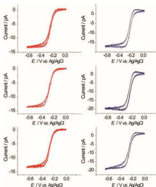
Figure 4. Typical CVs of 5 mM Ru(NH 3 ) 6 3+ reduction in 50 mM KCl at a scan rate of 100 mV s -1 . Red lines indicate forest sidewalls, blue lines, forest closed ends.
