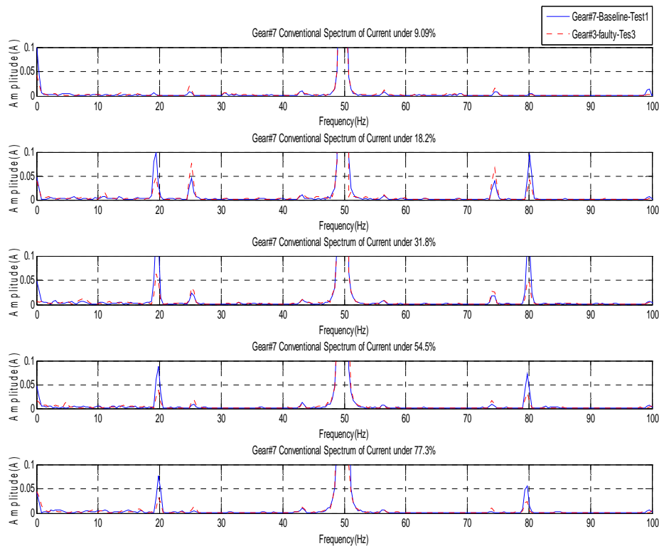
Figure 4 Motor current signals in non-slip compensation mode
