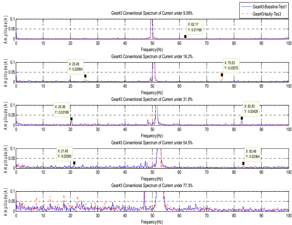
Figure 5 Motor current signals in slip compensation mode
