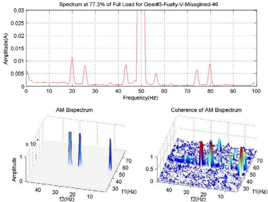
Figure 8 Spectrum and bispectrum at 77.3% of full load for gear with broken tooth and 0.46mm misalignment
