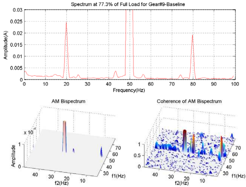
Figure 6 Spectrum and bispectrum at 77.3% of full load for healthy gear
