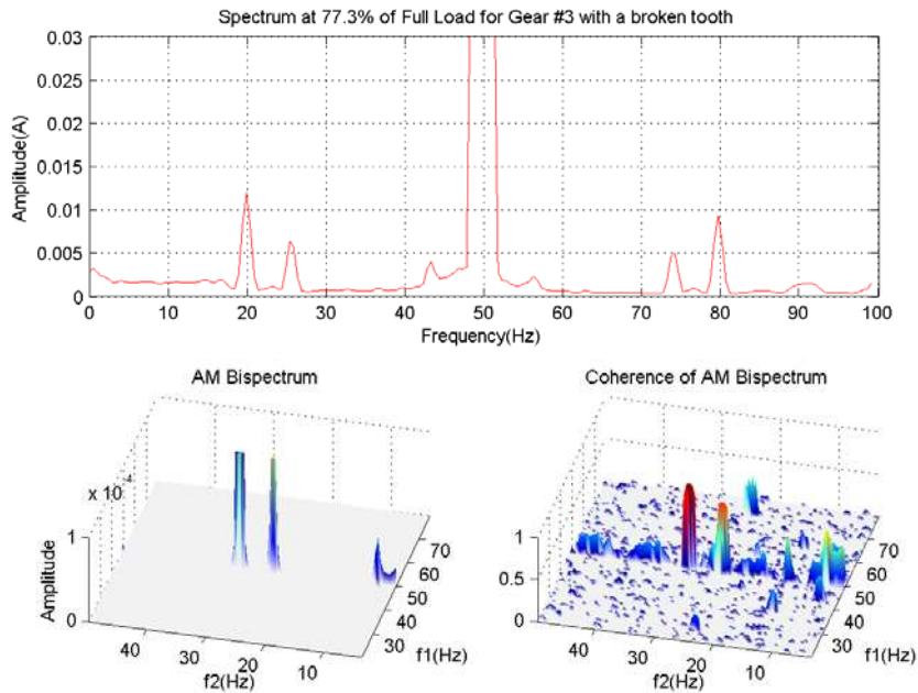
Figure 7 Spectrum and bispectrum at 77.3% of full load for gear with broken tooth
