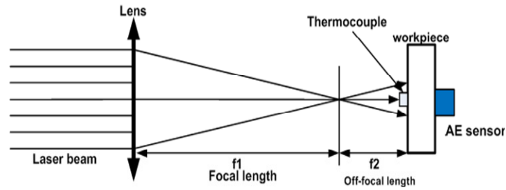
Figure 1: Schematic diagram of laser irradiation optical arrangement.
