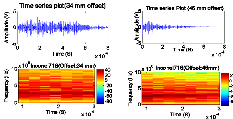
Figure 3: AE signal from laser irradiation, Top: time series data, and down: STFT.
