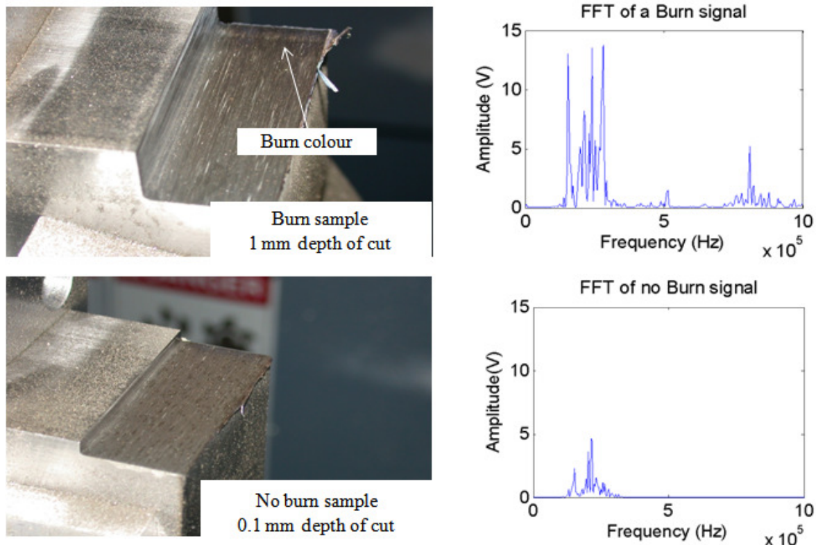
Figure 4 : Grinding burn and no burn phenomena related to 1.0mm and 0.1mm depth of cuts.
