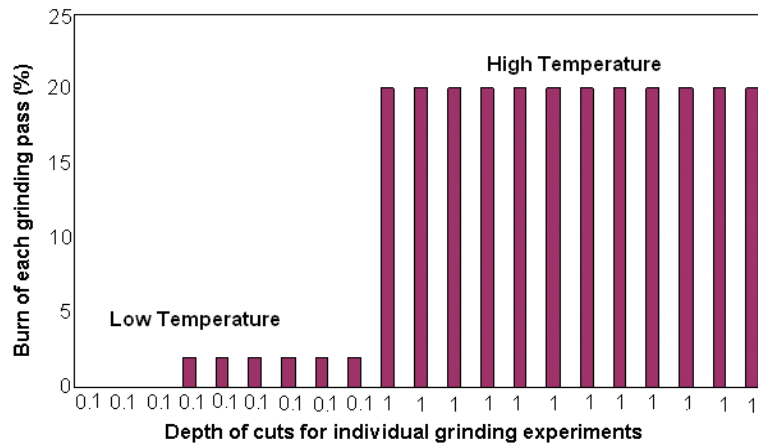
Figure 5: Grinding burn (%) from each grinding pass in relation to 0.1 mm and 1mm depth of cuts (Inconel718).
