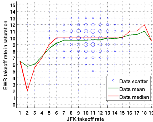
(c) EWR departure capacity as a function of JFK departures for 11,22L|22R EWR configuration.
