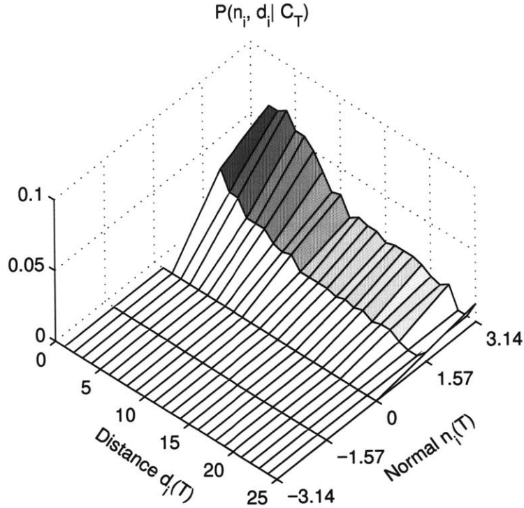
Figure 4-13: Empirical estimate of the joint density for normals and distances for tibial cartilage.
