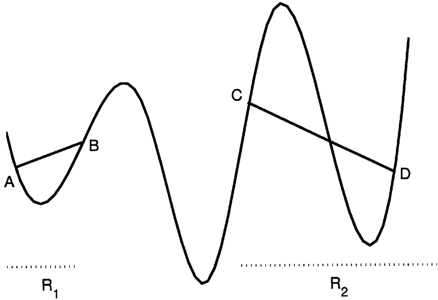
Figure 2-5: A function is strictly convex over a given region if the segment joining any two points in that region lies completely above the function. The above function is convex over the region R_1 and non-convex over R_2 .
