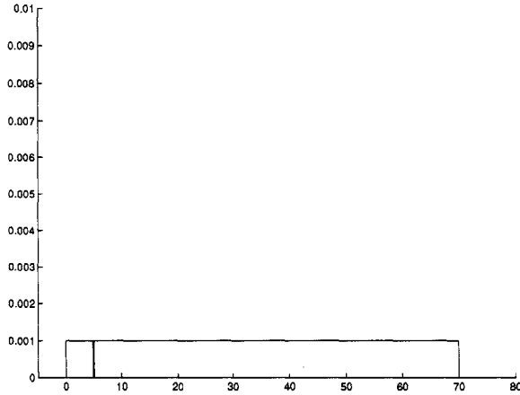
Figure 3-6: The estimated class conditional density function for \bar{l} . Note that it is uniform on the intervals [0, 5) and (5, 70] and is zero at \rho_{s,l'} = 5 .
