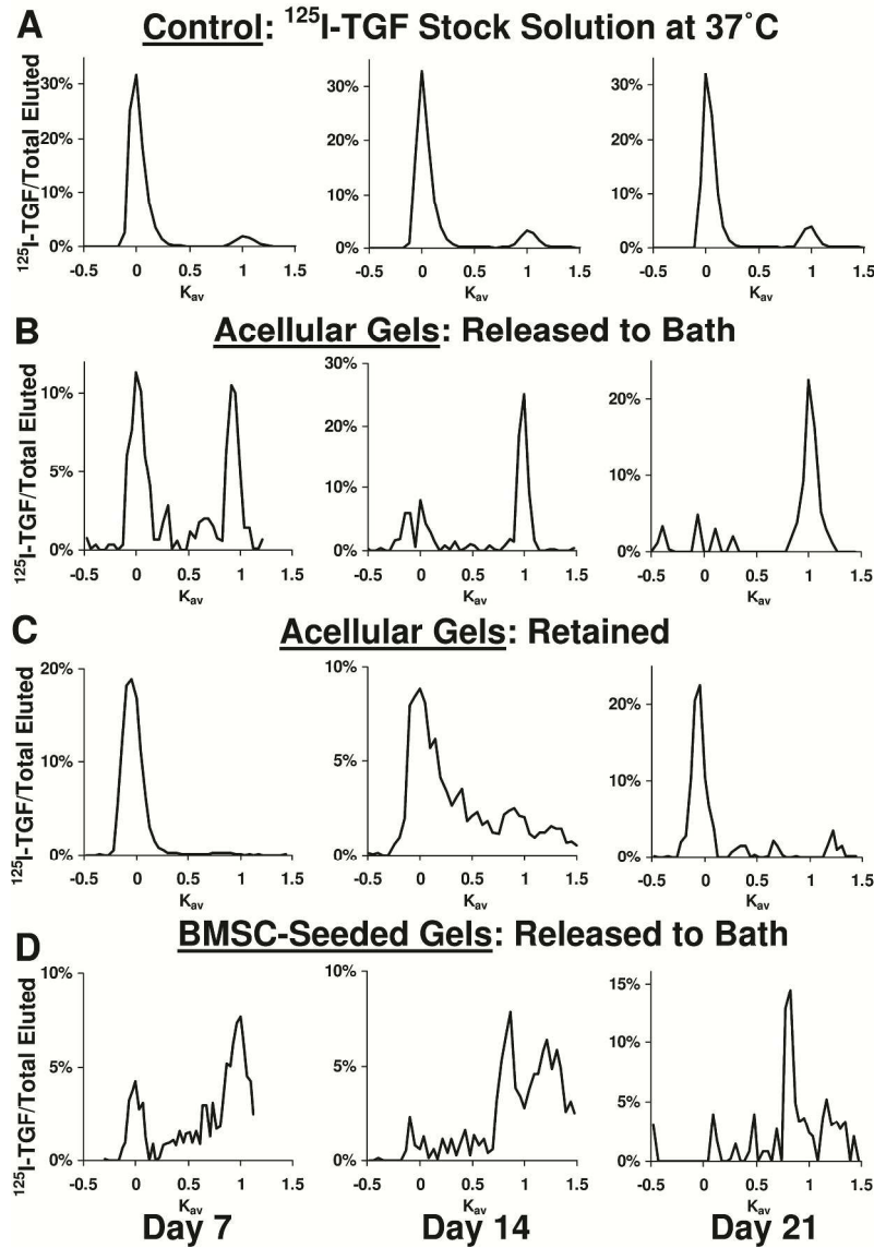
Figure 4. Size exclusion chromatography of ^{125}\text{I} -labeled species by Sephadex G25. (A) Control samples of ^{125}\text{I} -TGF- \beta 1 stock solution after 7, 14, & 21 days of incubation at 37°C. (B-D) ^{125}\text{I} -TGF- \beta 1 (1.4 ng/mL) plus unlabeled TGF- \beta 1 (100 ng/mL) was adsorbed to KLD peptide hydrogels. (B) ^{125}\text{I} -TGF- \beta 1 released to the bath from acellular peptide hydrogels. (C) ^{125}\text{I} -TGF- \beta 1 retained in acellular peptide hydrogels. (D) ^{125}\text{I} -TGF- \beta 1 released to the bath from bovine BMSC-seeded peptide hydrogels. 122x175mm (600 x 600 DPI)
