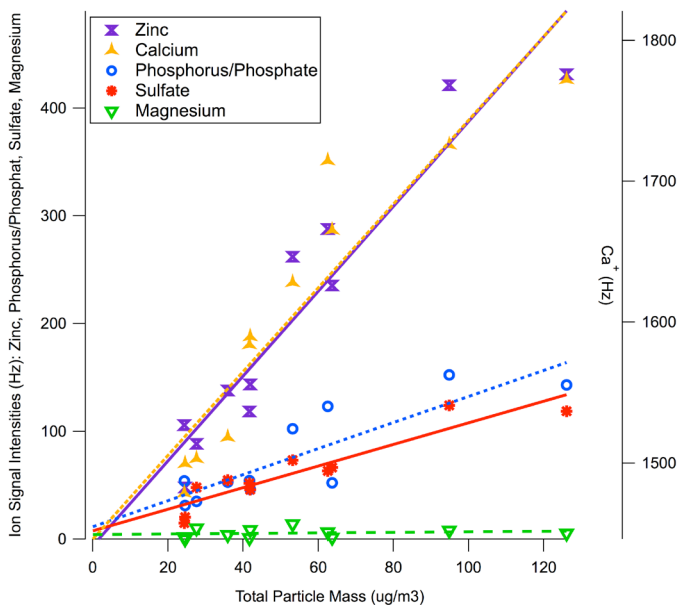
Figure 6. Ion response for calcium, zinc, phosphorus and sulfate species as a function of total particle mass measured with the SMPS.
