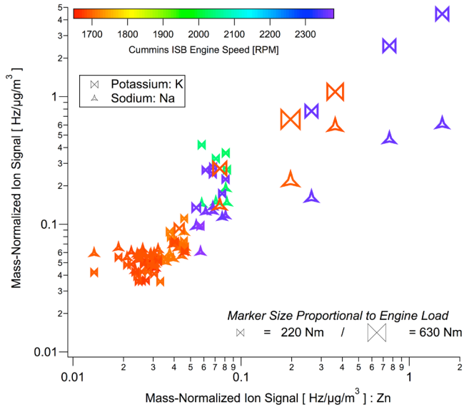
Figure 10. SP-AMS measurements of potassium and sodium as a function of zinc across all engine speed and load conditions studied. All ion signals are normalized to the SMPS measured mass concentration. Marker color and size indicate engine speed and load respectively.
