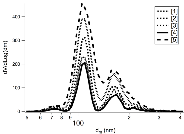
Figure 5. SMPS volume distributions obtained by varying the sheath flow rate in the size-selecting DMA to systematically control the total mass concentration of particles sampled with the SP-AMS. The bi-modal distribution results from doubly charged particles (with equivalent mobility to singly charge 100 nm particles) being transmitted through the size-selecting DMA.
