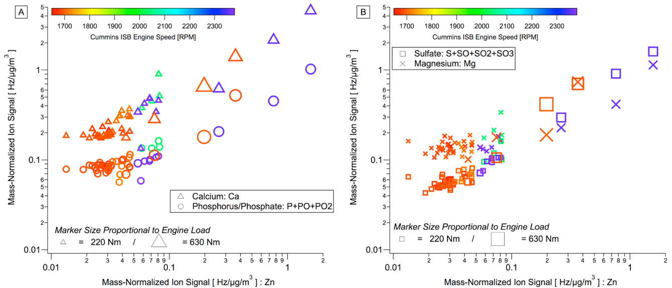
Figure 8. (a) SP-AMS measured calcium and phosphorus/phosphate and (b) sulfate and magnesium as a function of zinc. All ion signals are normalized to the SMPS measured mass concentration. Marker color and size indicate engine speed and load respectively.
