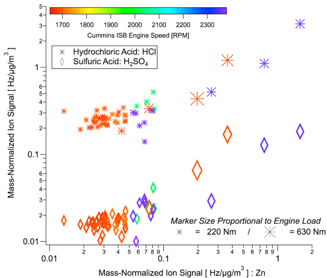
Figure 12. SP-AMS measurements of hydrochloric acid and sulfuric acid as a function of zinc across all engine speed and load conditions studied. All ion signals are normalized to the SMPS measured mass concentration. Marker color and size indicate engine speed and load respectively.
