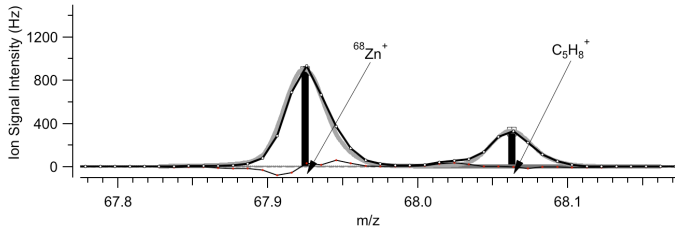
Figure 1. Ion signal intensities measured at nominal m/z = 68 showing a peak corresponding to the Zn_{68}^+ isotope at 67.9248 amu and a hydrocarbon fragment C_5H_8^+ at 68.0626 amu. The residual between the peak fit and raw data is also plotted in the figure.
