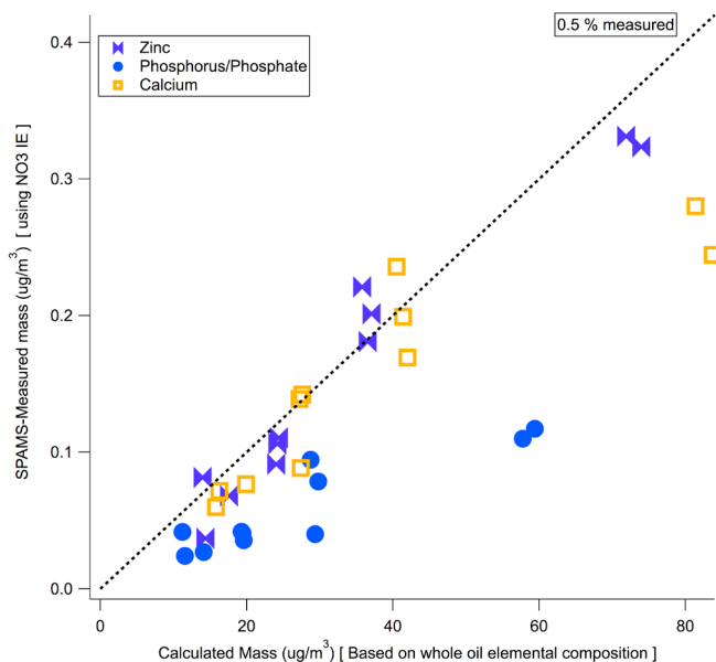
Figure 7. SP-AMS measured mass concentrations for zinc, calcium and phosphorus/phosphate as a function of calculated mass concentrations for each component based on elemental analysis of CJ-4.
