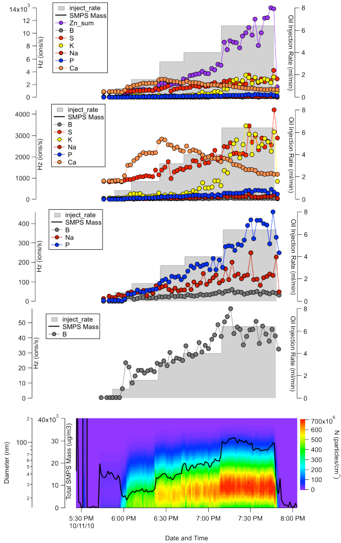
Figure 4. Specific lubricant-derived ash species ion signal intensities as a function of increasing CJ-4 oil injection rate. SMPS-measured size distribution is displayed as an image plot colored by the number concentration in the lower panel of the plot.
