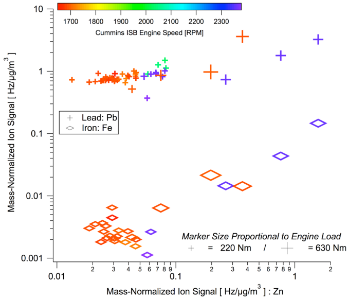
Figure 11. SP-AMS measurements of lead and iron as a function of zinc across all engine speed and load conditions studied. All ion signals are normalized to the SMPS measured mass concentration. Marker color and size indicate engine speed and load respectively.
