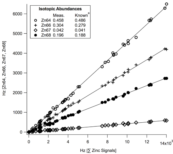
Figure 2. Empirical measurement of the isotopic abundance for each major isotope of zinc.
