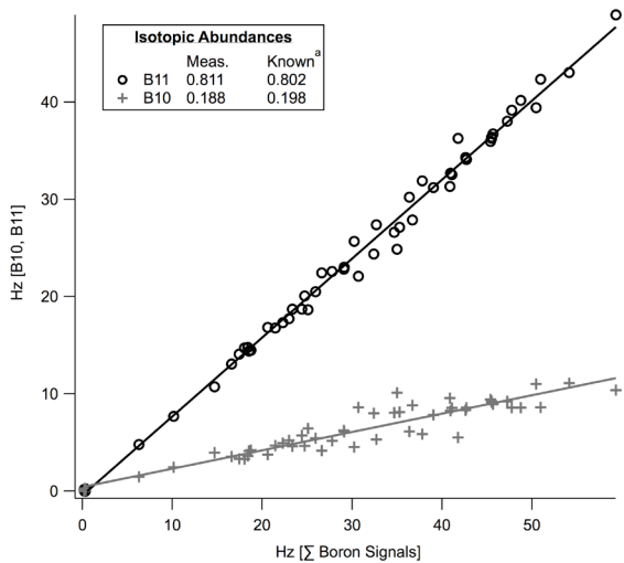
Figure 3. Empirical measurement of isotopic abundance for boron.
