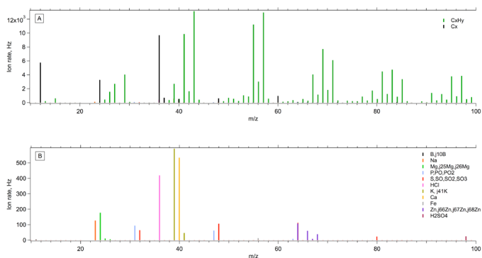
Figure 9. Average mass spectrum measured during high speed/high load engine operation. The upper panel (a) plots all ion signals and is dominated by hydrocarbon fragments (C x H y , green) and black carbon (C x , black). The lower panel (b) displays ion fragments associated with trace elements from the CJ-4, fuel, and engine wear.
