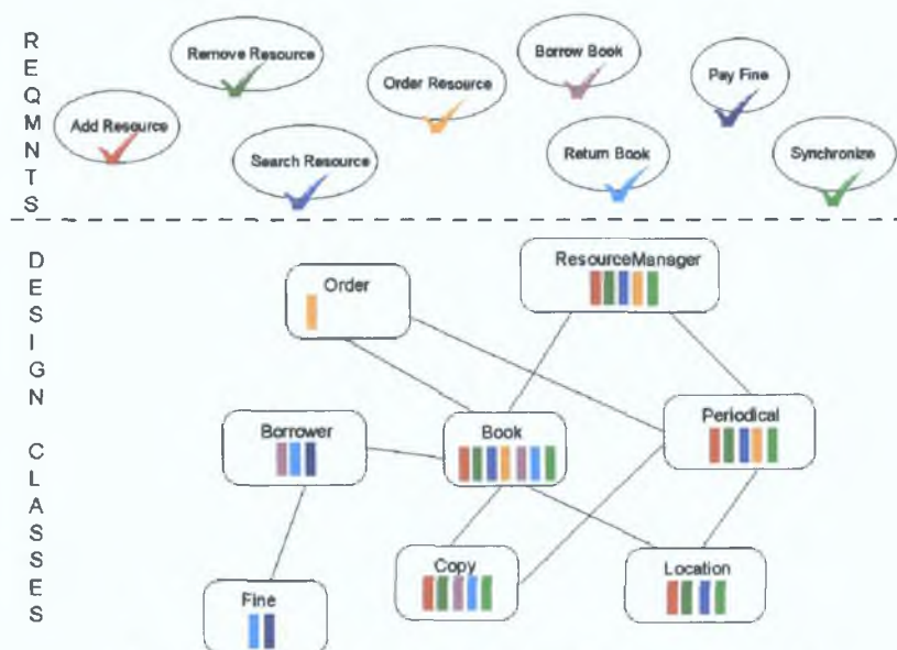
Figure 114: Initial Assessment of Project Classes and Tasks
