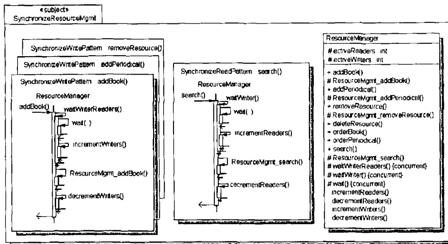
Figure 135 Output of Composition with Synchronization
