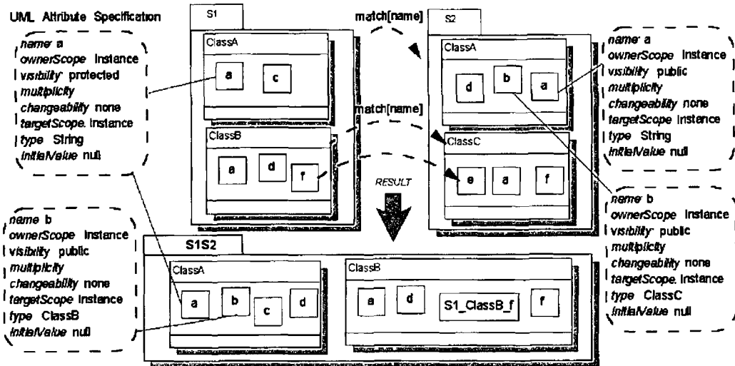
Figure 48 Impact of Override on Attribute Specifications
