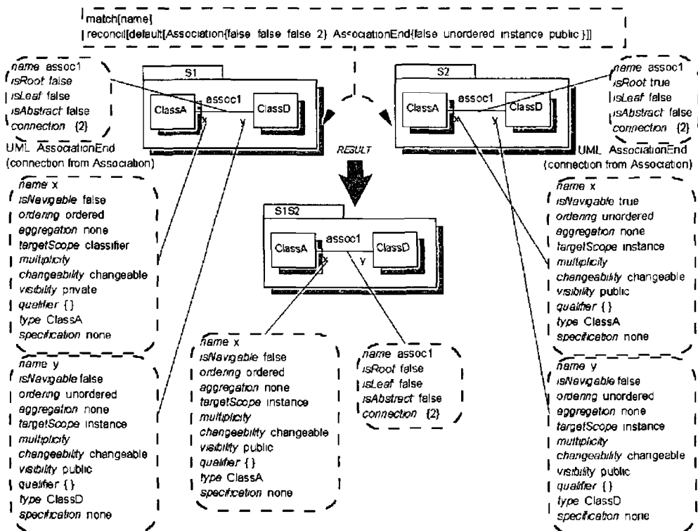
Figure 82 Example 2 Using Defaults to Reconcile Conflicts in Associations
