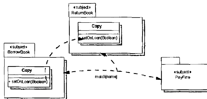
Figure 132 Specify Composition of Borrowing Subjects
