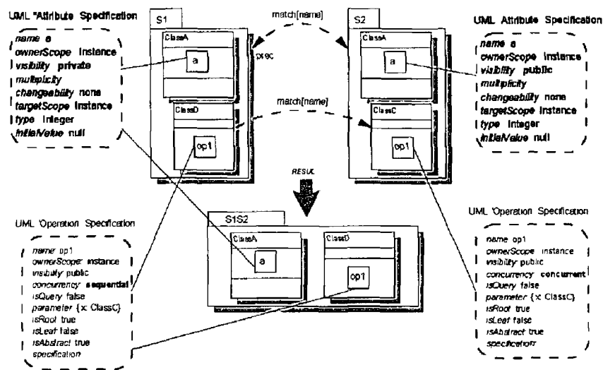
Figure 34 Loss of (some) Constraints in Input Subjects
