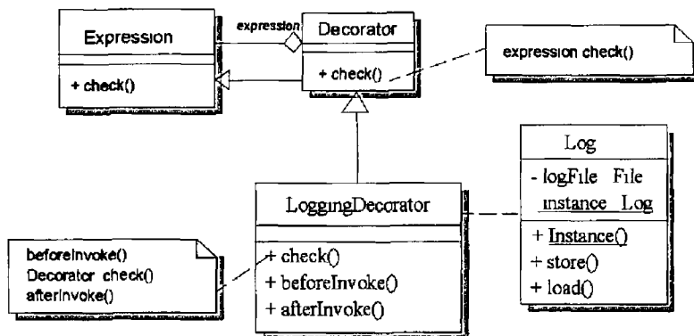
Figure 12 Using Decorator for Logging
