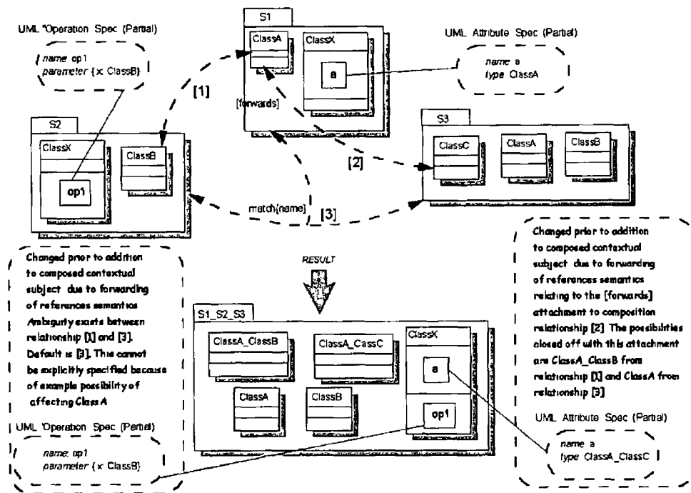
Figure 42 Forwarding to Implicit Composition Output as Default
