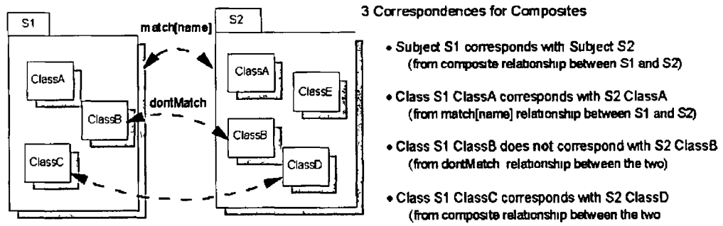
Figure 39 Correspondences between Composites
