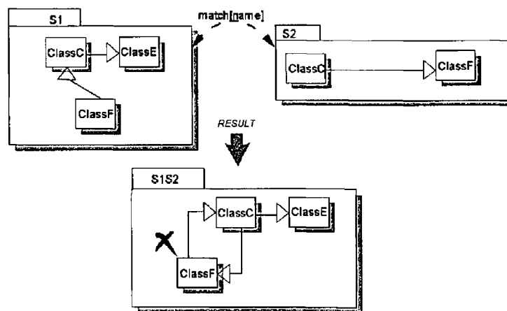
Figure 85 Example 2 Impact of Merge on Generalizations
