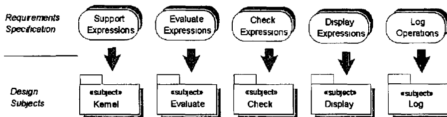
Figure 13 Matching SEE Requirements with Design Models
