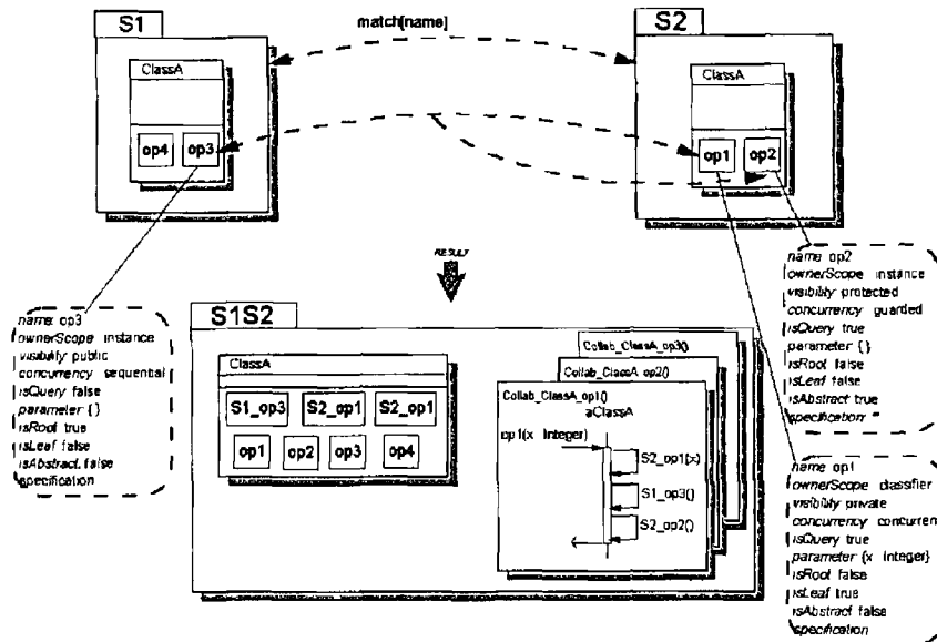
Figure 35 Composing Incompatible Operations
