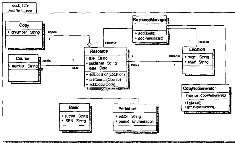
Figure 116 Add Resource Class Diagram
