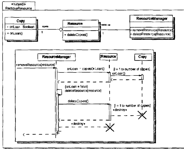
Figure 118 Remove Resource Class Diagram and Interactions
