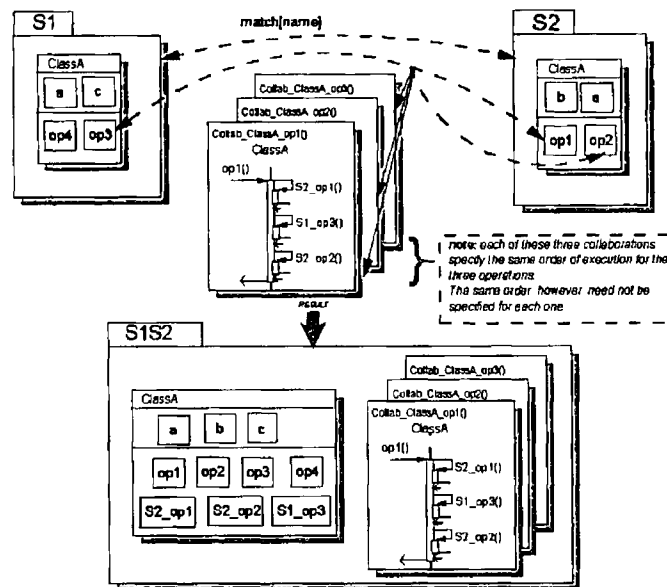
Figure 30 Merge Integration with Interaction Specification
