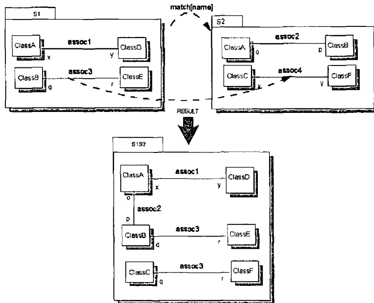
Figure 53 Example 4 Result of Override on Associations
