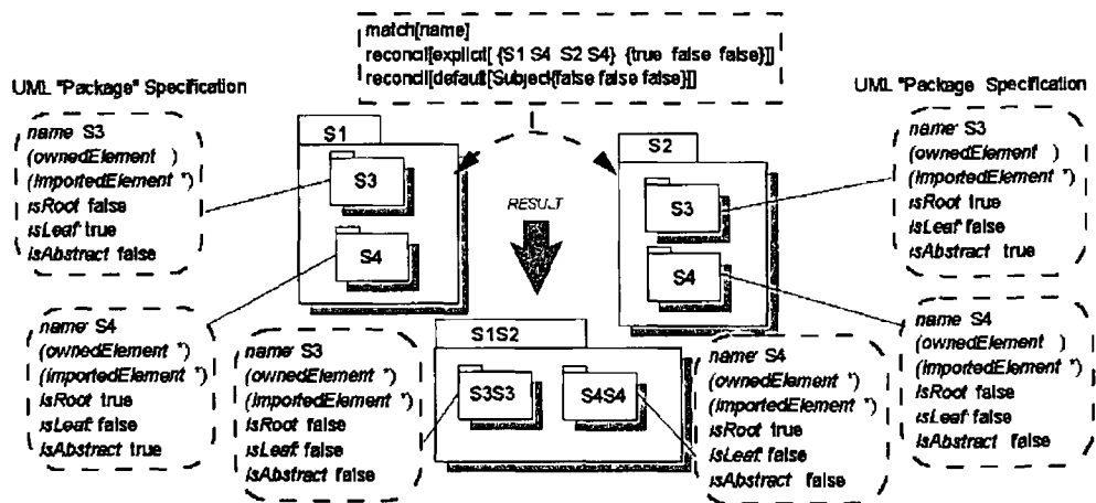
Figure 75 Reconciling Conflicts in Subject Specifications
