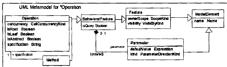
Figure 145 Partial UML Metamodel for Operations
