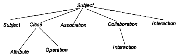
Figure 17 A Subject as a Tree Structure
