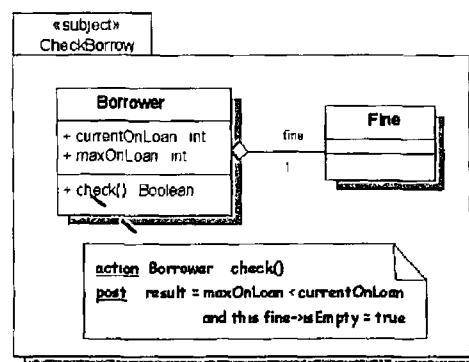
Figure 136 Updating rules for borrowing
