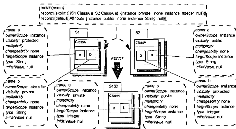
Figure 80 Reconciling Conflicts in Attribute Specifications
