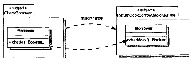
Figure 138 Specify Composition of Borrow Checking Update
