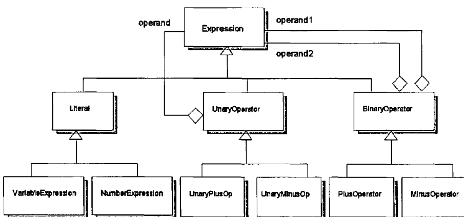
Figure 3 Composite Pattern for AST
