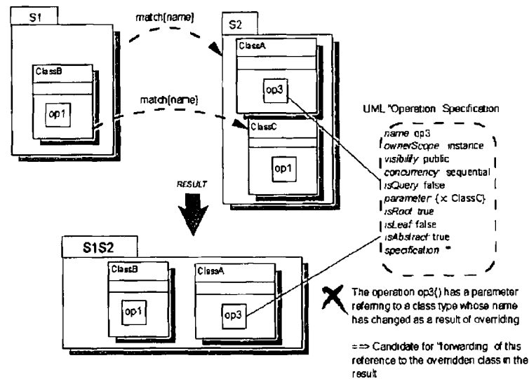
Figure 31 Forwarding References to Composed Elements
