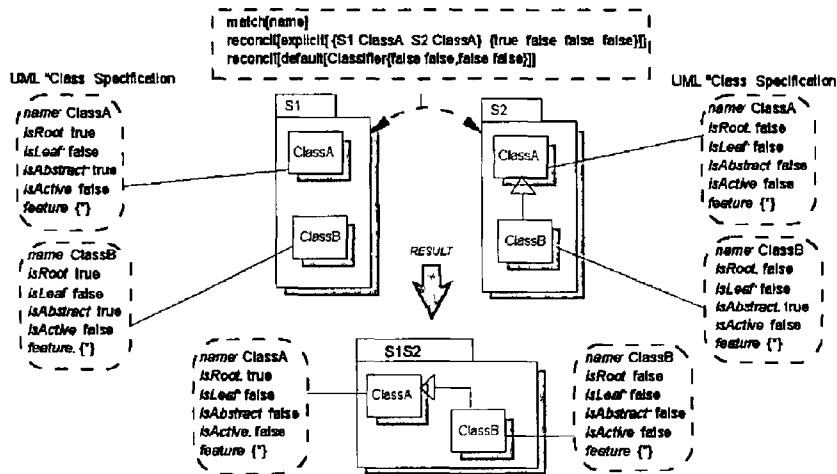
Figure 78 Reconciling Conflicts in Classes
