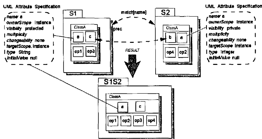
Figure 67 Reconciliation with Subject Precedence
