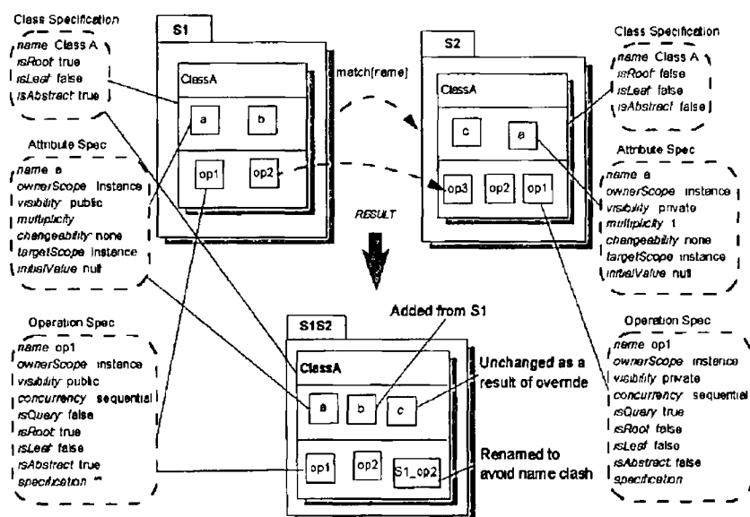
Figure 28 General Override Semantics
