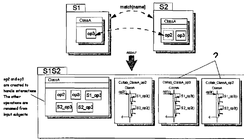
Figure 91 Operations involved in Multiple Compositions
