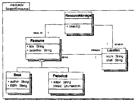
Figure 121 Search Resource Class Diagram
