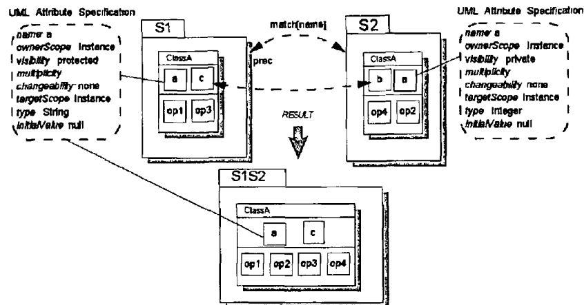
Figure 29 Merge Integration with Reconciliation Specification
