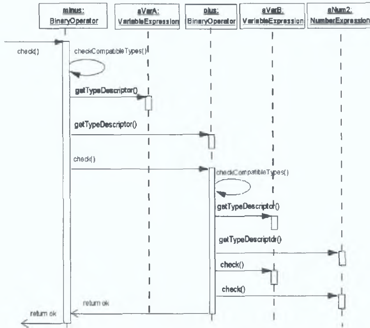
Figure 5: Sequence Diagram for Checking the Syntax of an Expression: A-B+2
