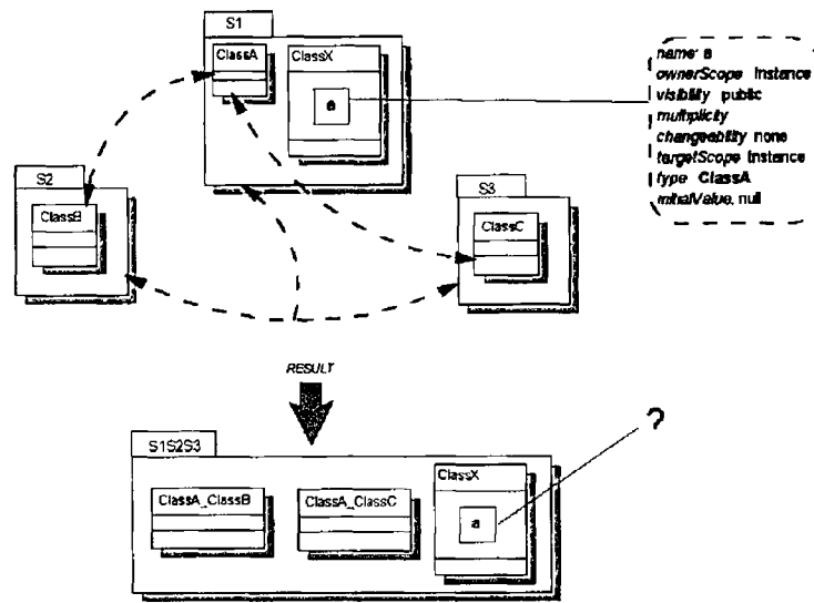
Figure 32 Ambiguities with Forwarding of References
