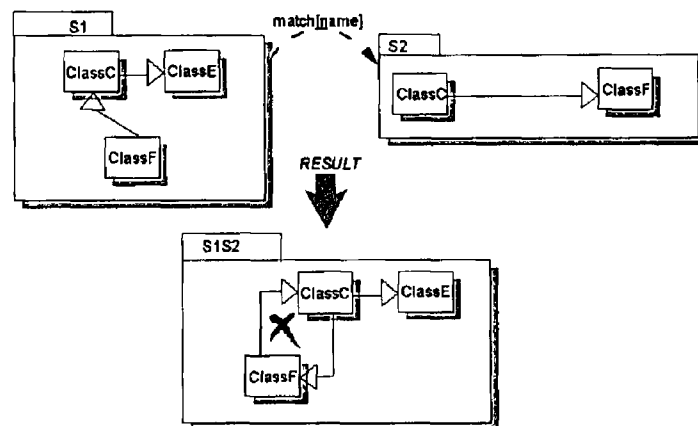
Figure 55 Example 2 Impact of Override on Generalizations
