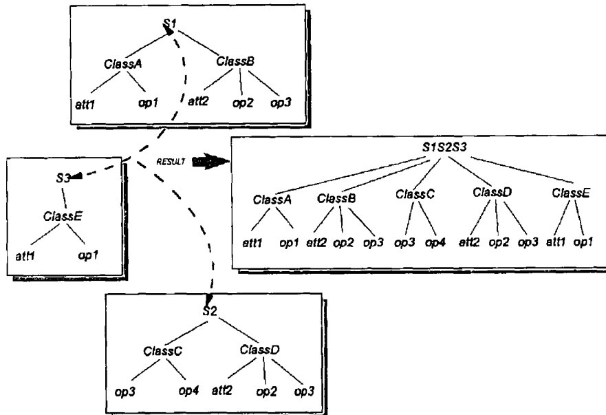
Figure 18 Composing Design Subjects to New Result
