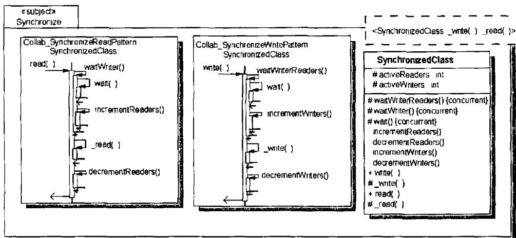
Figure 127 Synchronize Pattern Classes and Interactions
