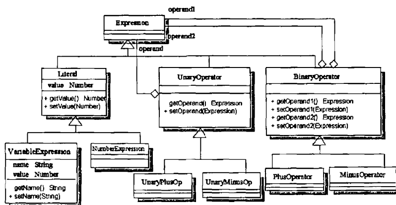
Figure 4 Core Expression Design in UML
