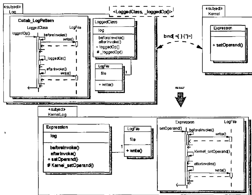
Figure 112 Applying Composition Pattern for Logging
