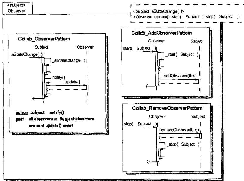
Figure 99 Specifying Patterns of Cross-Cutting Behaviour
