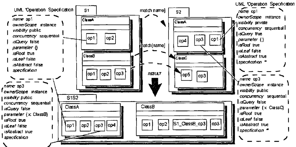
Figure 49 Impact of Override on Operation Specifications
