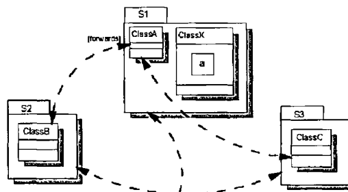
Figure 33 Resolving Ambiguities with Forwarding of References
