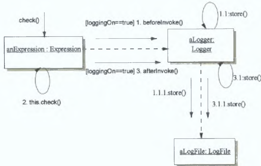
Figure 8: Collaboration Diagram for Logging Utility: Example - Check ()
