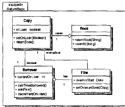
Figure 124 Return Book Class Diagram
