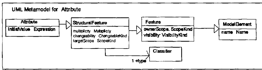
Figure 144 Partial UML Metamodel for Attributes
