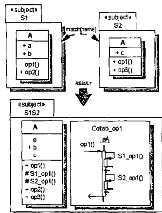
Figure 97 Merge Integration Example
