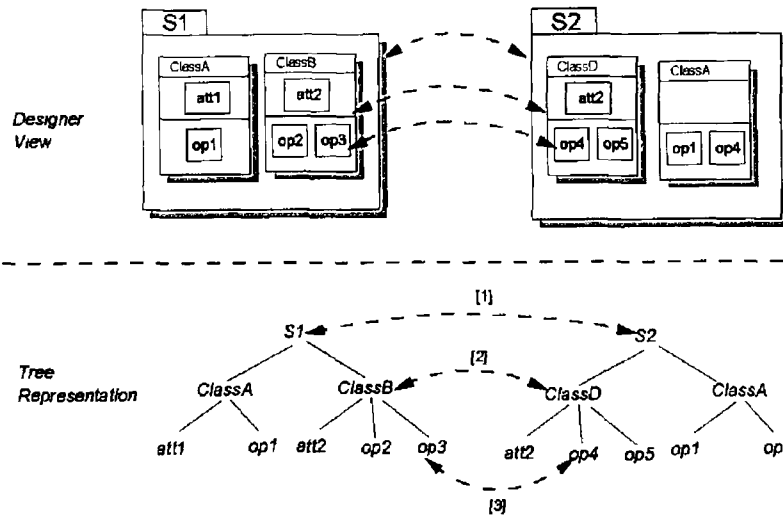
Figure 24 Multiple Composition Relationships
