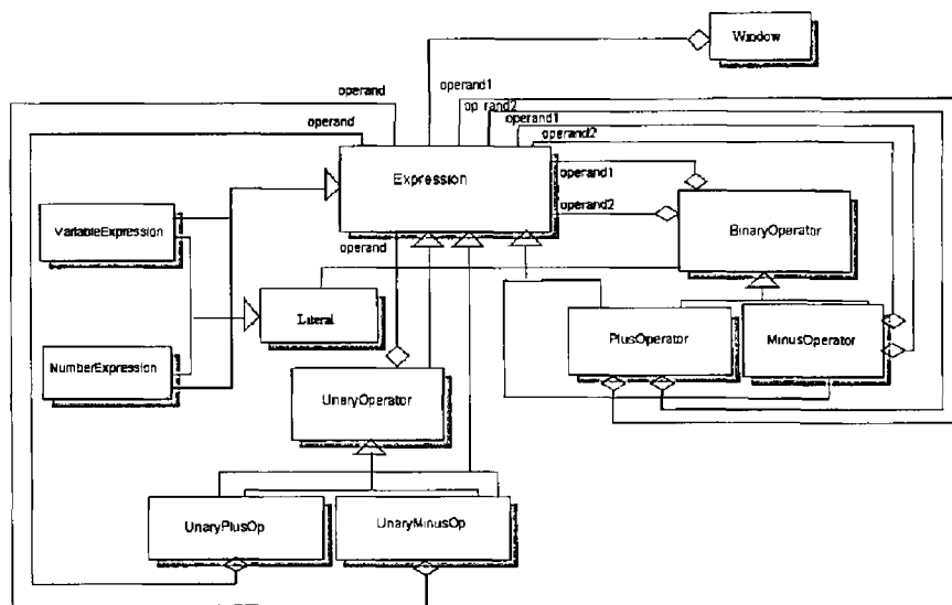
Figure 111 Composed SEE Design with Relationships
