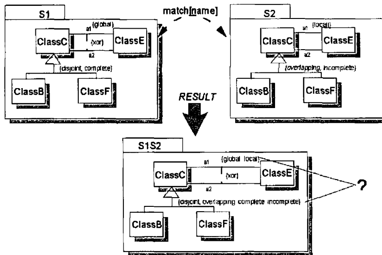
Figure 89 Example 3 Impact of Merge on Constraints
