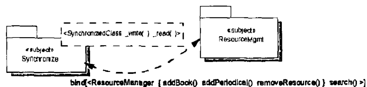
Figure 134 Specify Composition with Synchronization
