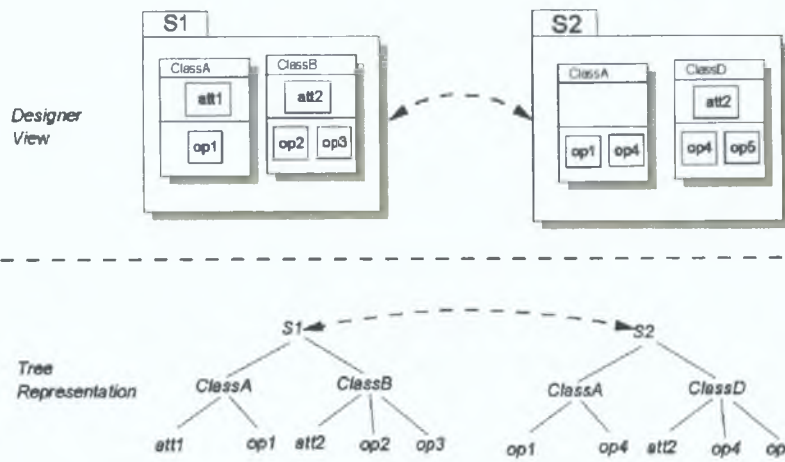
Figure 20: Subject-Level Inputs to Composition
