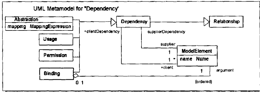
Figure 147 Partial UML Metamodel for Dependency
