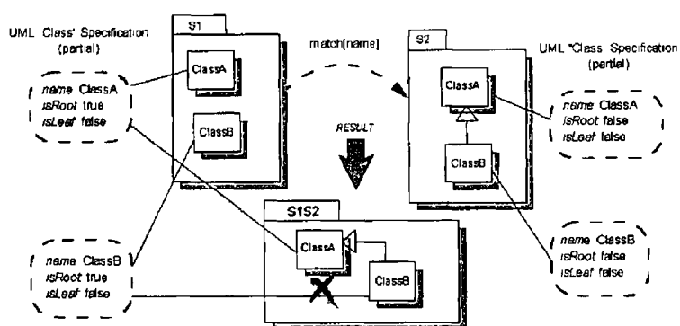
Figure 47 Breaking Well-Formedness Rules for Classifiers
