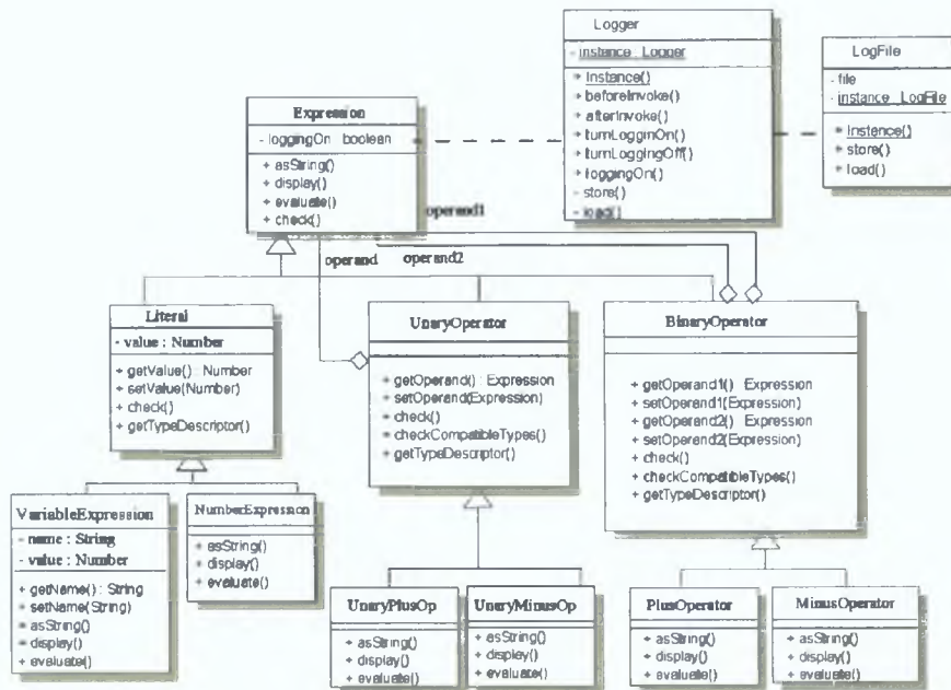
Figure 9: UML Class Diagram for SEE, Version 1.0
