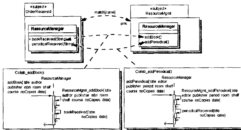
Figure 140 Specify Composition with Receiving Orders
