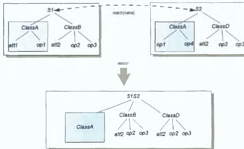
Figure 19: Composing Design Subjects with Overlap
