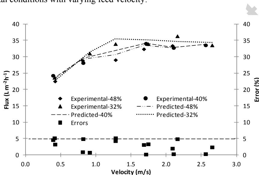
Figure 7 Comparison of predicted flux with initial experimental flux at different feed velocities and different packing densities
