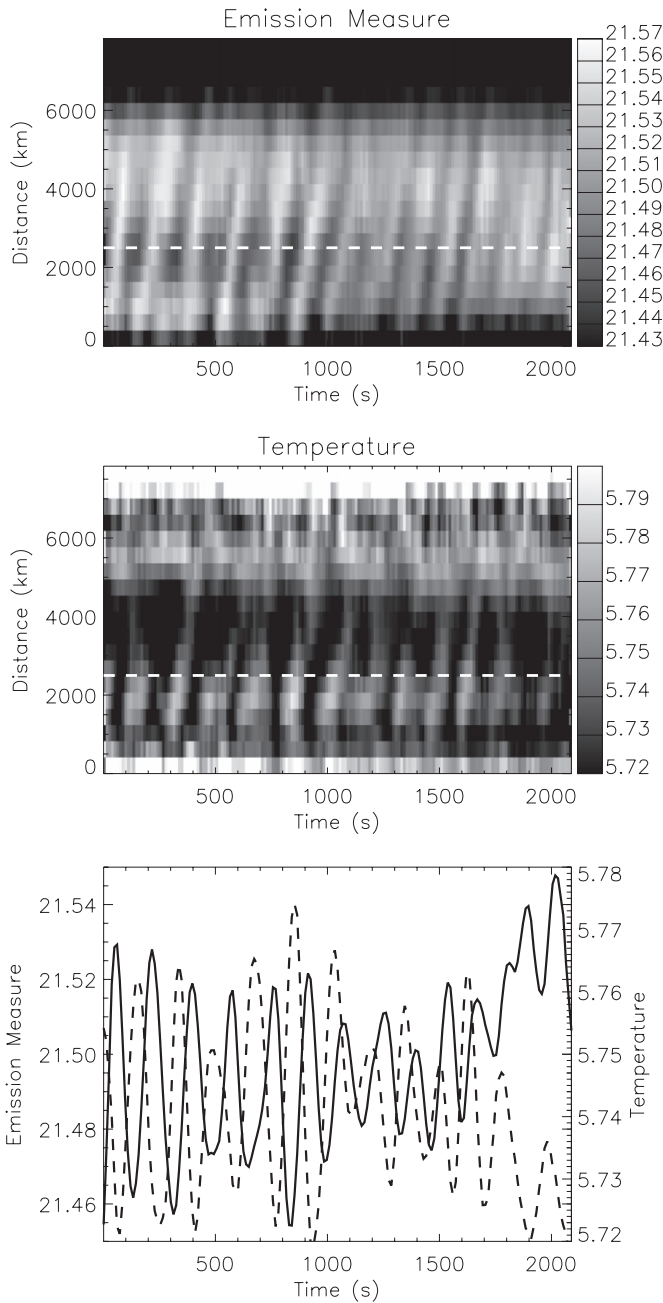
Figure 8. Time–distance diagrams of the emission measure (in units of \text{cm}^{-5} \text{K}^{-1} ; top) and temperature (in units of \log(T_e) ; middle), derived for the fan structure where propagating wave phenomenon in EUV intensity images was detected. The dashed white lines highlight the spatial position along the slice (2500 km from the underlying umbra) where EM and T_e time series were created. These values are displayed in the lower panel, where the solid line represents the emission measure, and the dashed line traces the temperature. Both time series are displayed in their native units, as used in the top and middle panels. A clear anti-correlation between the EM and T_e time series is readily apparent.
