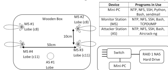
Figure 1: Data Capture System Layout (Milliken & Marshall, 2012).
