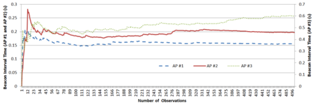
Figure 3: Beacon Interval Average Trace for each AP Monitored at MS#2.
