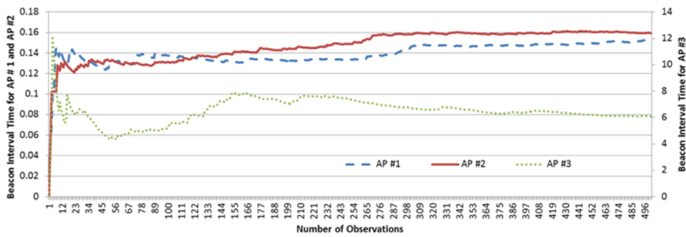
Figure 1: Beacon Interval Average (s) Trace for each AP Monitored at MS#1.
