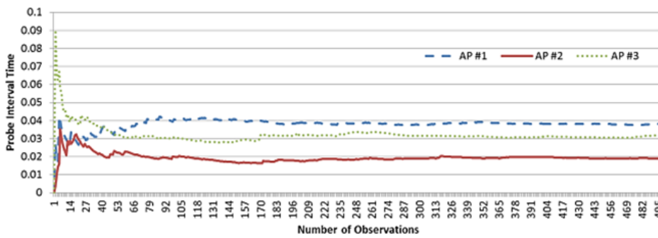
Figure 2: Probe Exchange Interval Average (s) Trace for each AP Monitored at MS#1.
