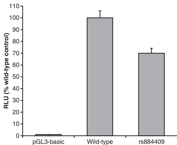
Fig 1. Promoter activity without (wild-type) and with rs884409 SNP. Wild-type or mutant rs884409 SNP luciferase reporter constructs were transiently transfected into Caco-2 cells and relative luciferase activity (RLU) was measured 48 h later. rs884409 SNP is localized to nucleotide -326 relative to the TSS-1 and had a significant negative association with basal promoter activity ( P = 0.0043 ). Data are representative of two independent experiments measured in triplicate, presented as means \pm standard deviation and analysed using 1-way analysis of variance and Tukey's post hoc test. Data is presented as % of Wild-type promoter activity set as 100.
