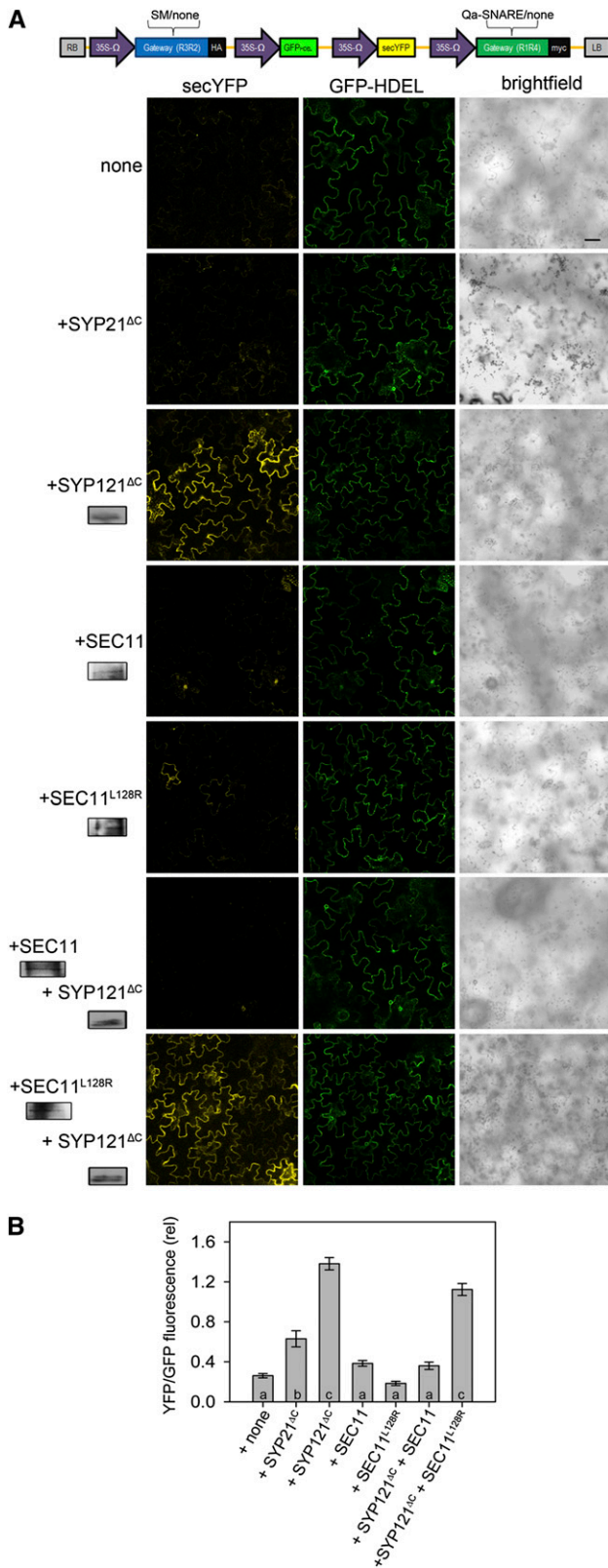
Figure 7. Secretory Traffic Block in Vivo by SYP121 \Delta C Is Rescued by SEC11, but Not by SEC11 L128R .
