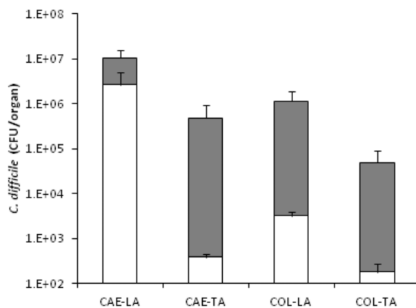
Figure 3. Colonisation kinetics of C. difficile CD1342 in hamsters. To monitor colonisation throughout the infection process hamsters were culled at 1- (A), 3- (B) and 11 (C) days post challenge. C. difficile was recovered from the caecum (CAE) and the colon (COL) either associated with the lumen (LA) and the tissue (TA). Filled bars represent vegetative bacteria whilst empty bars indicate bacteria in
