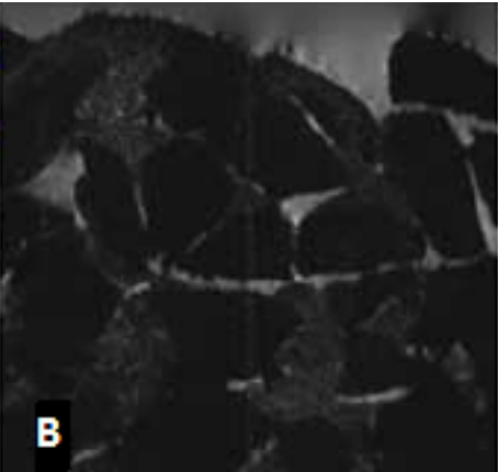
Figure 3a: Grey-scale (un-thresholded) MRI data slices (2D) of fine infiltration into a gravel framework following water-working. Image (A) shows sealing, where coarse sand deposits confined to the upper layers of the bed. Image (B) shows siltation by fine sand throughout the sample depth with isolated and interconnected voids present on the underside of gravel particles. Image adapted from Haynes et al. (2009).
