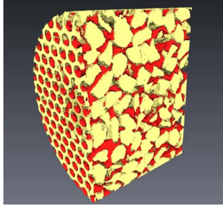
Figure 3b: Post-processed MRI data (3D volume) indicating kaolin deposition (red) within a 10mm gravel framework (yellow). Remaining pore spaces are shaded grey. This follows 10 days of clogging at 50ml/min and average sedimentation rates of 0.54g/hour. Pipe diameter was ~100mm with flow entering via a perforated plate (left of image). Images generated using Avizo software, courtesy of J. Minto, University of Glasgow.
