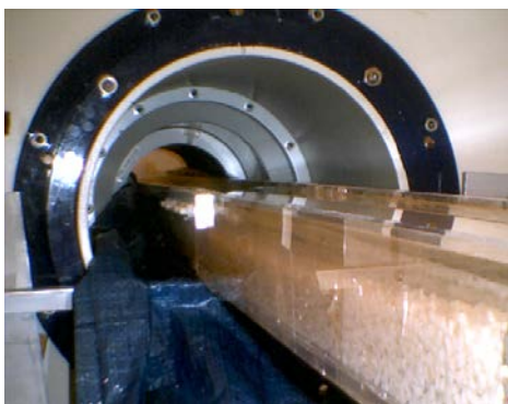
Figure 5: Trials of a bespoke MR-compatible open-channel flume (100mm rectangular cross-section) within the bore of the 7T MRI system at Glasgow's Experimental MRI Centre. All flume components and fixings within the MRI room are Perspex, made water-tight via rubber seals. The flow-recirculation pump is
