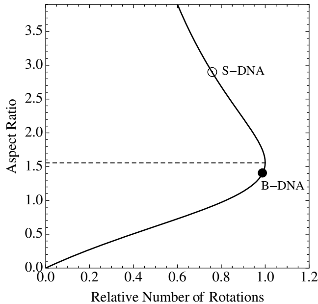
Figure 4. Aspect ratio of DNA versus number of rotations on the double helix (solid line). At the turning point the aspect ratio is A^* = 1.56 (dashed line), separating two regimes with low and high aspect ratio, respectively. The circle at A = 2.90 is the aspect ratio of an example of a stretched DNA, so-called S-DNA from [31].
