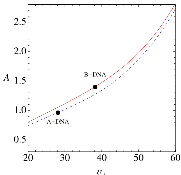
Figure 5. Aspect ratio A versus pitch angle \nu_{\perp} plotted for double helix with minor groove (solid, red curve) and symmetric double helix (dashed, blue curve). The solid circles are for A-DNA and B-DNA using [1].
