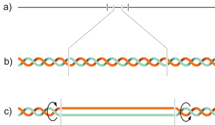
Figure 2. Transcription on (A) a long string of DNA; (B) a subsection of double-stranded DNA before melting takes place and (C) with strand separation having appeared. Also shown by arrows are the many rotations the DNA must be able to absorb.
