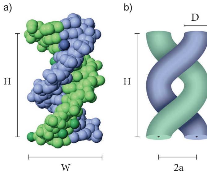
Figure 1. (A) B-DNA structure plotted using MATLAB R2011b (MathWorks) from crystallographic data deposited in PDB (The Protein Data Bank, see [2]). The entry id 425D was used, for additional information on the specific molecule, see [3]. Indicated in the figure is the pitch height, H , and the helix-packing diameter, W . The aspect ratio is A = H/W . (B) Sketch of tube model of DNA molecule discussed in section 2.
