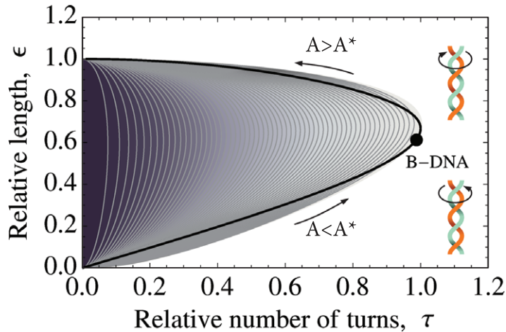
Figure 3. Relative length, \epsilon , of double helix as a function of the relative number of turns, \tau , on the strand. The solid curve is the configurations where the two strands are in contact. The aspect ratio increases along the curve from zero at the lower left corner, to 1.56 at the turning point, and approaching infinity at the upper left endpoint. In the present paper B-DNA is found to have an aspect ratio of 1.40 corresponding to the point below the turning point. The contour lines have constant volume fraction, along the outer contour its value is 0.597 corresponding to B-DNA.
