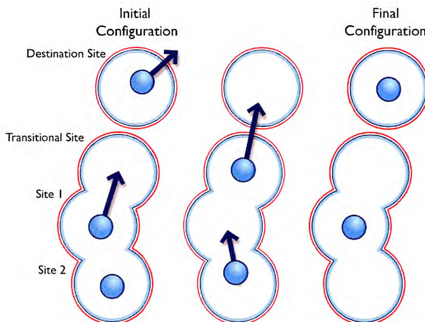
Figure 3.19: Alkali migration occurs by a concerted hopping mechanism (after [112]).
