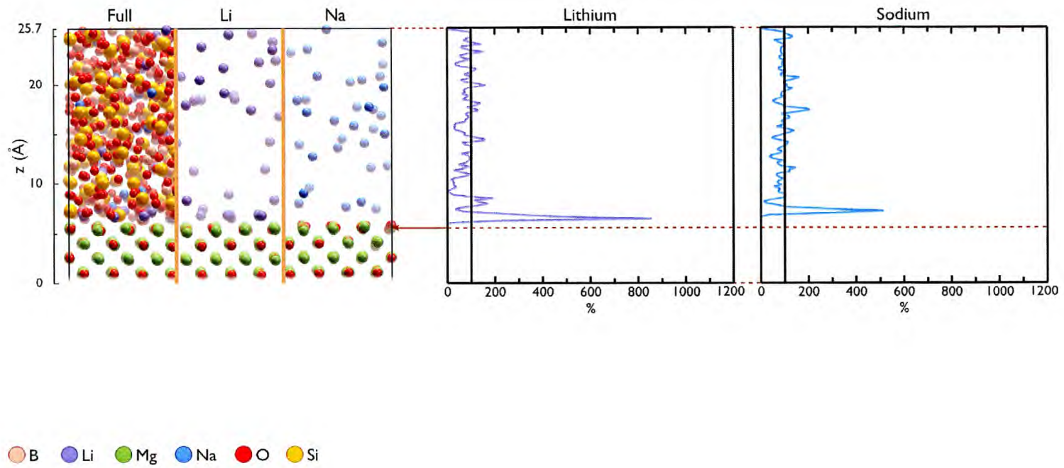
Figure 4.21: Alkali Concentration Profile: MW glass MgO-(110).
