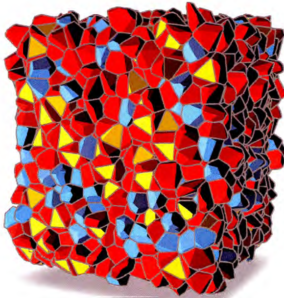
Figure 3.9: Voronoi diagram for a random set of points.
