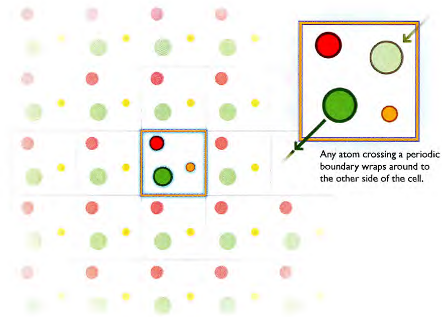
Figure 2.1: Illustration of periodic boundary conditions in two dimensions. The central simulation cell is surrounded by images of itself tessellated in space.
