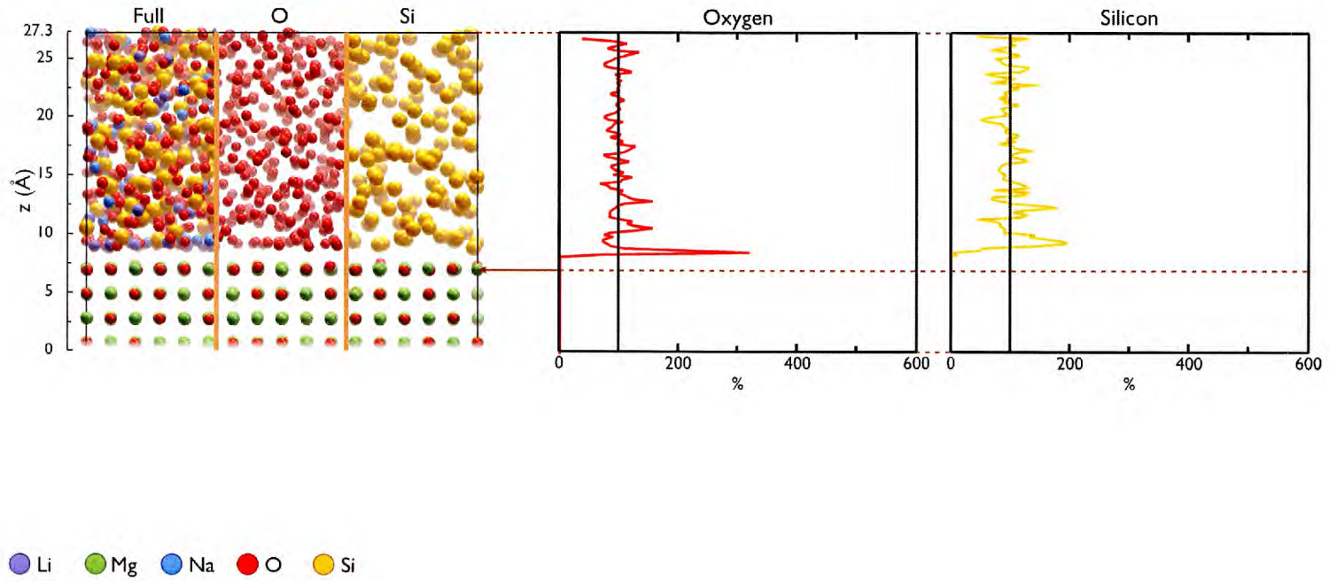
Figure 5.3: Network Former Concentration Profile: \text{SiO}_2+\text{Na}+\text{Li MgO}-(100) .
