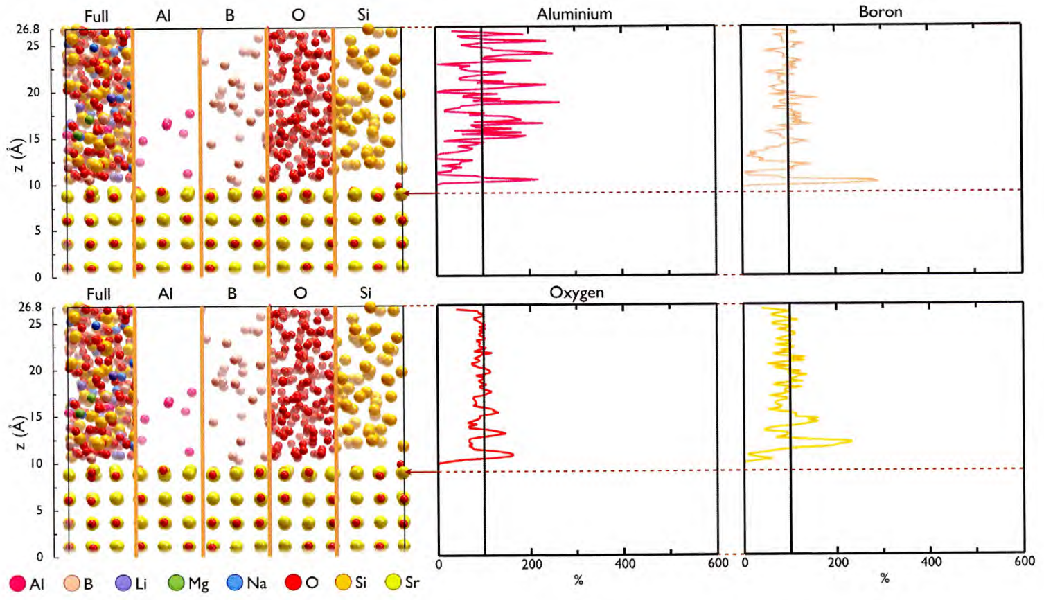
Figure 5.14: Network Former Concentration Profile: MW+Al+Mg glass SrO-(100).
