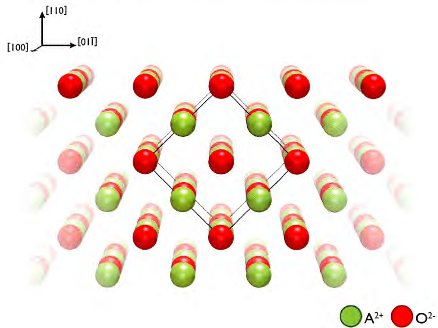
Figure 2.4: The (110) surface of the rock-salt structure. The rock-salt unit cell is highlighted. Crystallographic directions given relative to rock-salt unit cell (figure 2.3).
