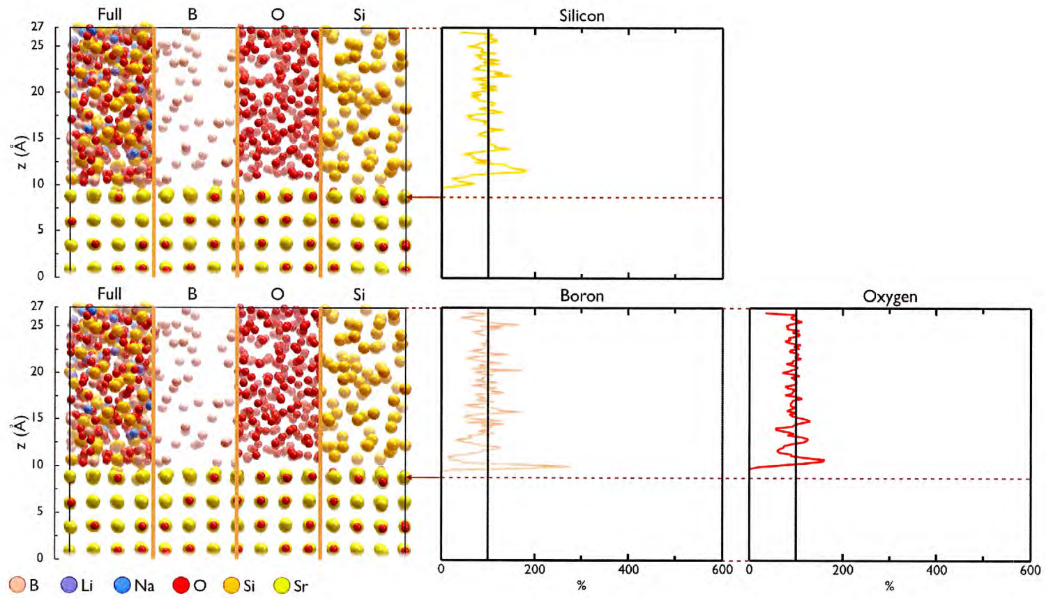
Figure 5.6: Network Former Concentration Profile: MW glass SrO-(100).
