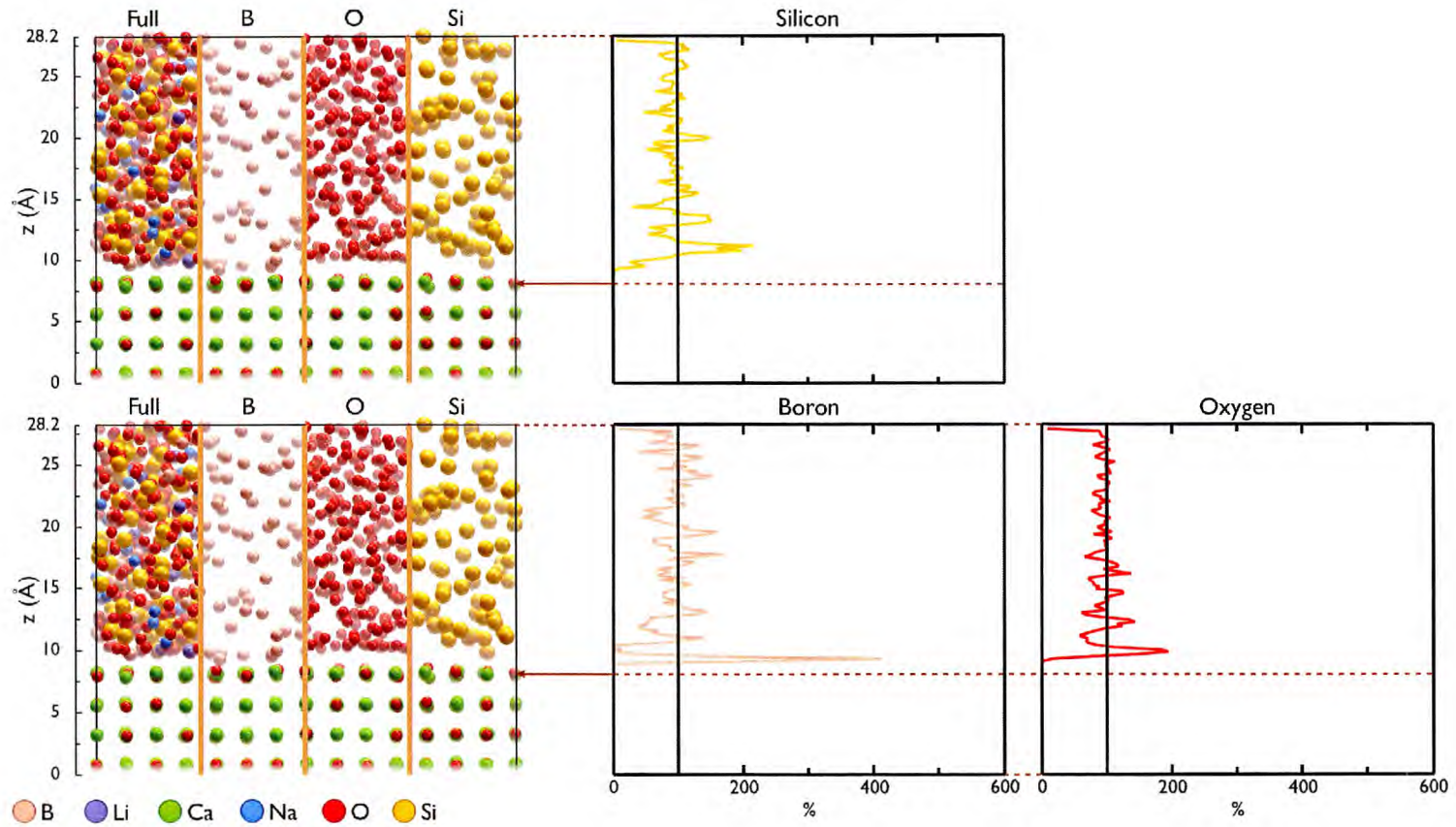
Figure 5.5: Network Former Concentration Profile: MW glass CaO-(100).
