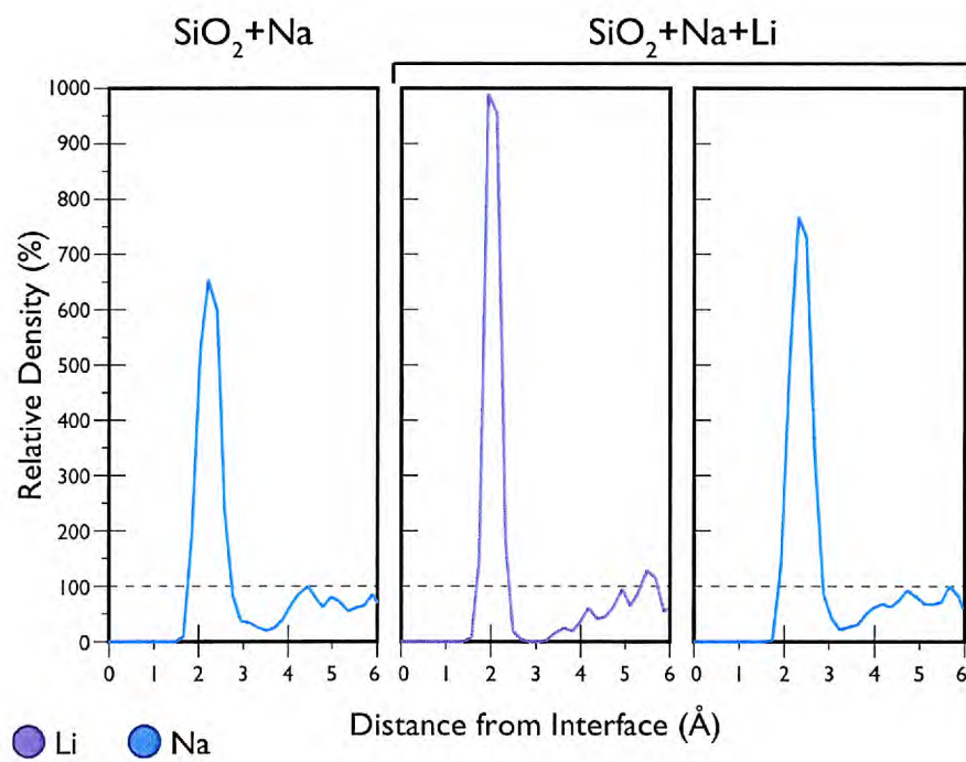
Figure 4.38: Alkali distribution close to the interfaces of \text{SiO}_2+\text{Na} and \text{SiO}_2+\text{Na}+\text{Li} with \text{MgO} -(100). Behind the initial peak a region of low alkali concentration existed.
