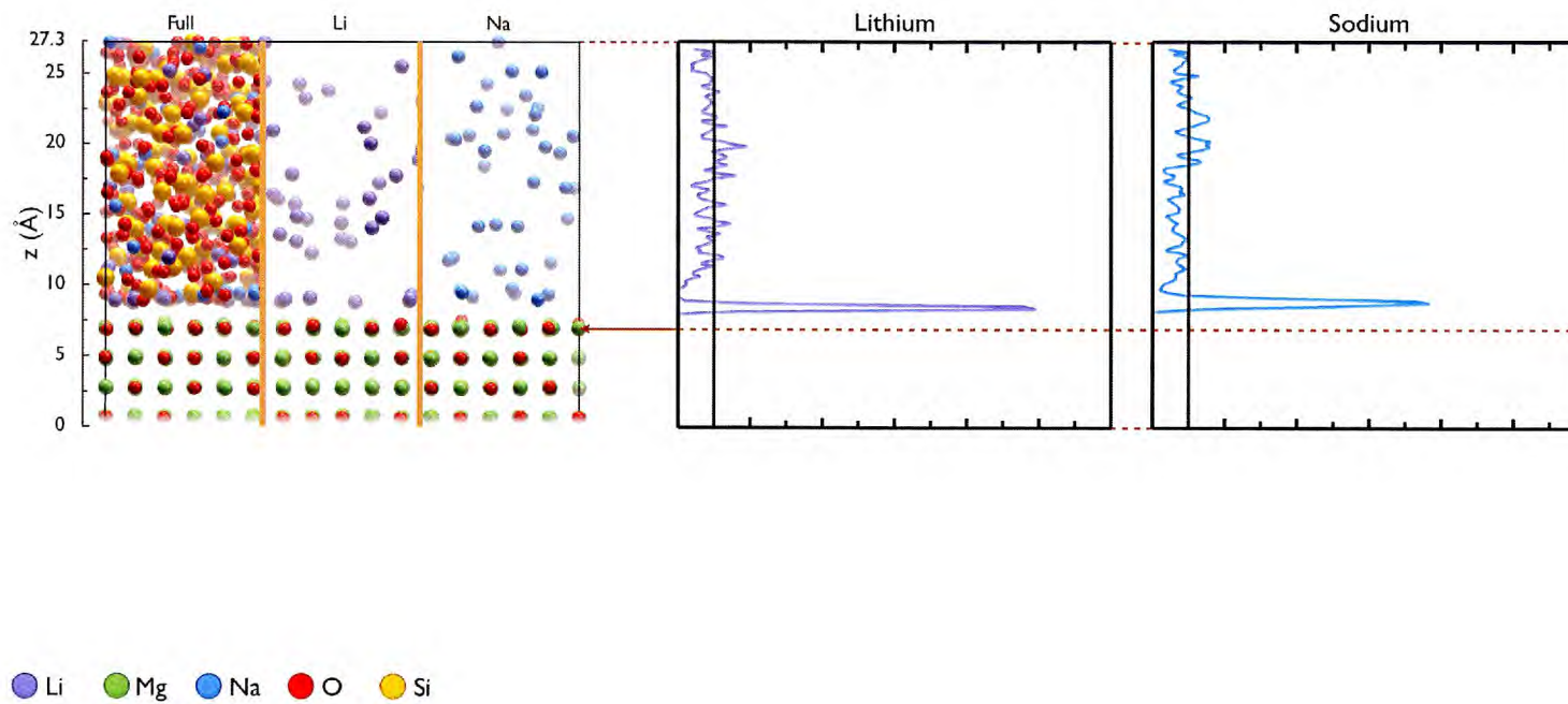
Figure 4.16: Alkali Concentration Profile: \text{SiO}_2+\text{Na}+\text{Li MgO}-(100) .
