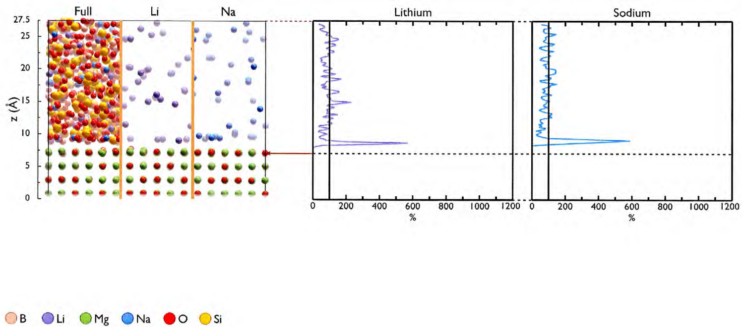
Figure 4.17: Alkali Concentration Profile: MW MgO-(100).
