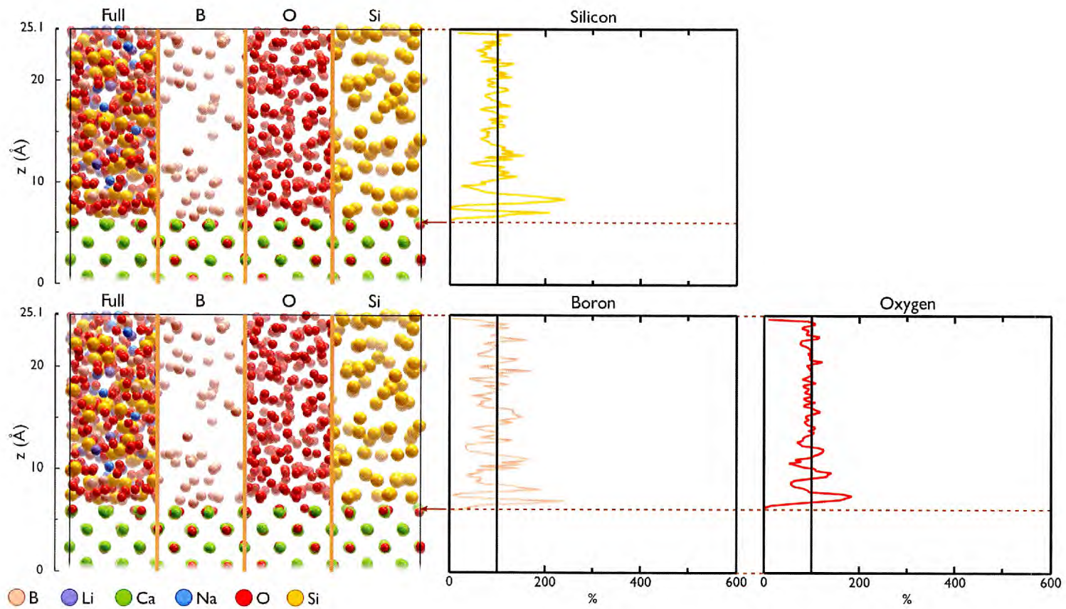
Figure 5.9: Network Former Concentration Profile: MW glass CaO-(110).
