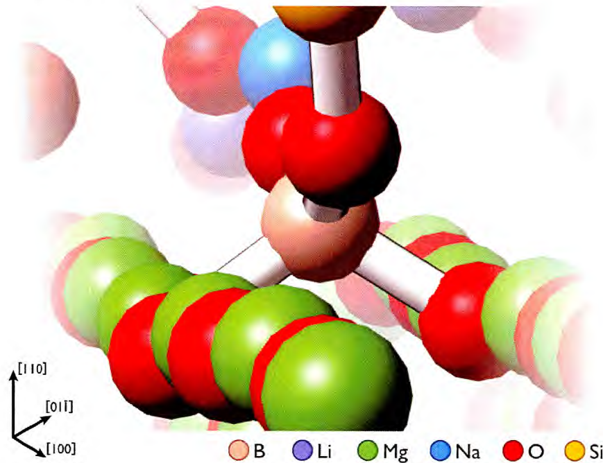
Figure 4.13: A borate unit spanning a furrow in at the MW glass MgO-(110) interface.
