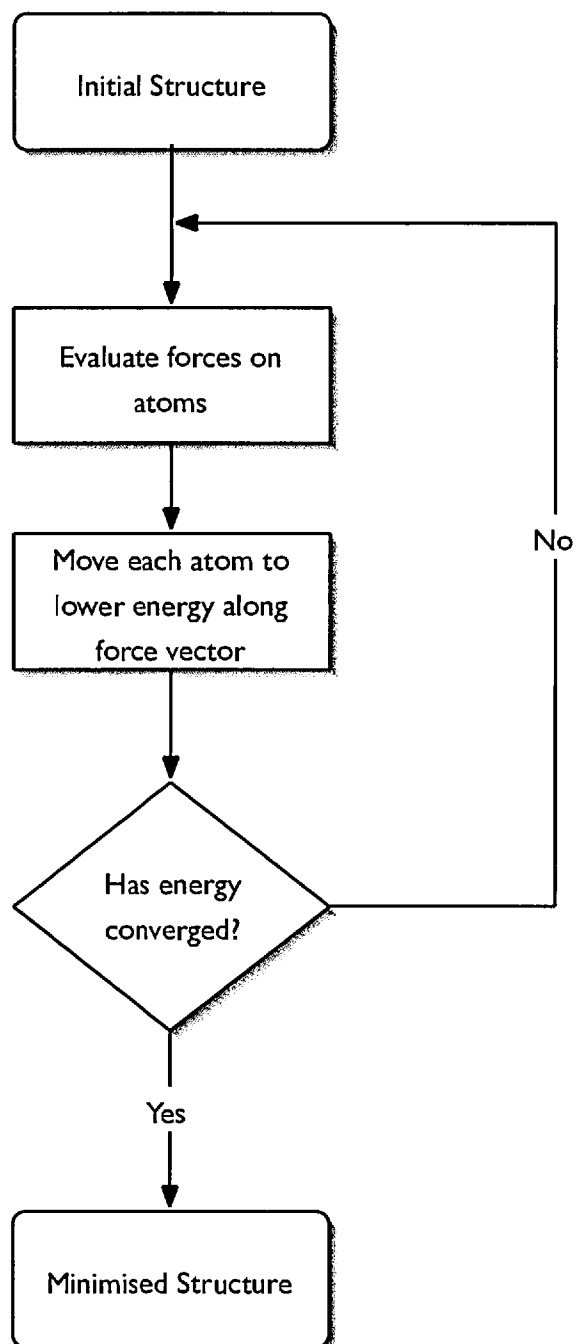
Figure 2.9: The basic energy minimisation algorithm.
