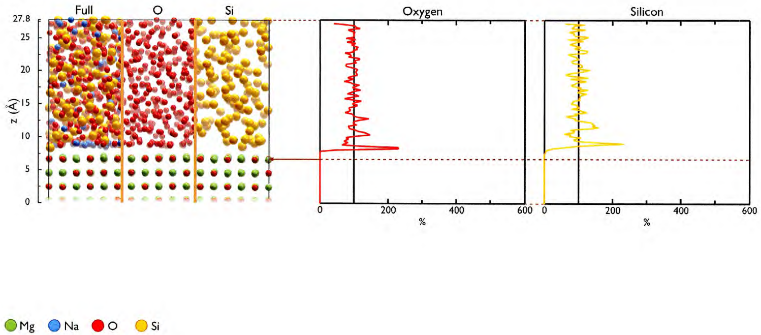
Figure 5.2: Network Former Concentration Profile: \text{SiO}_2+\text{Na MgO}-(100) .
