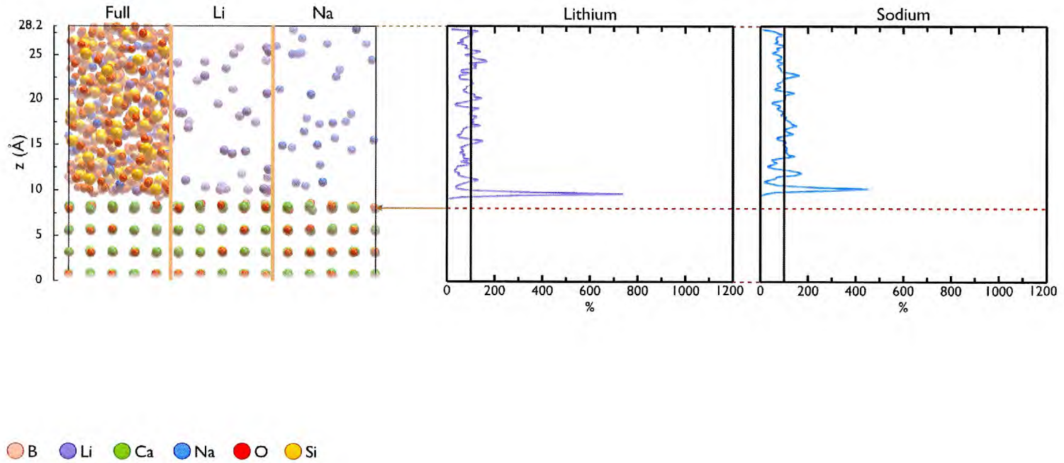
Figure 4.18: Alkali Concentration Profile: MW glass CaO-(100).
