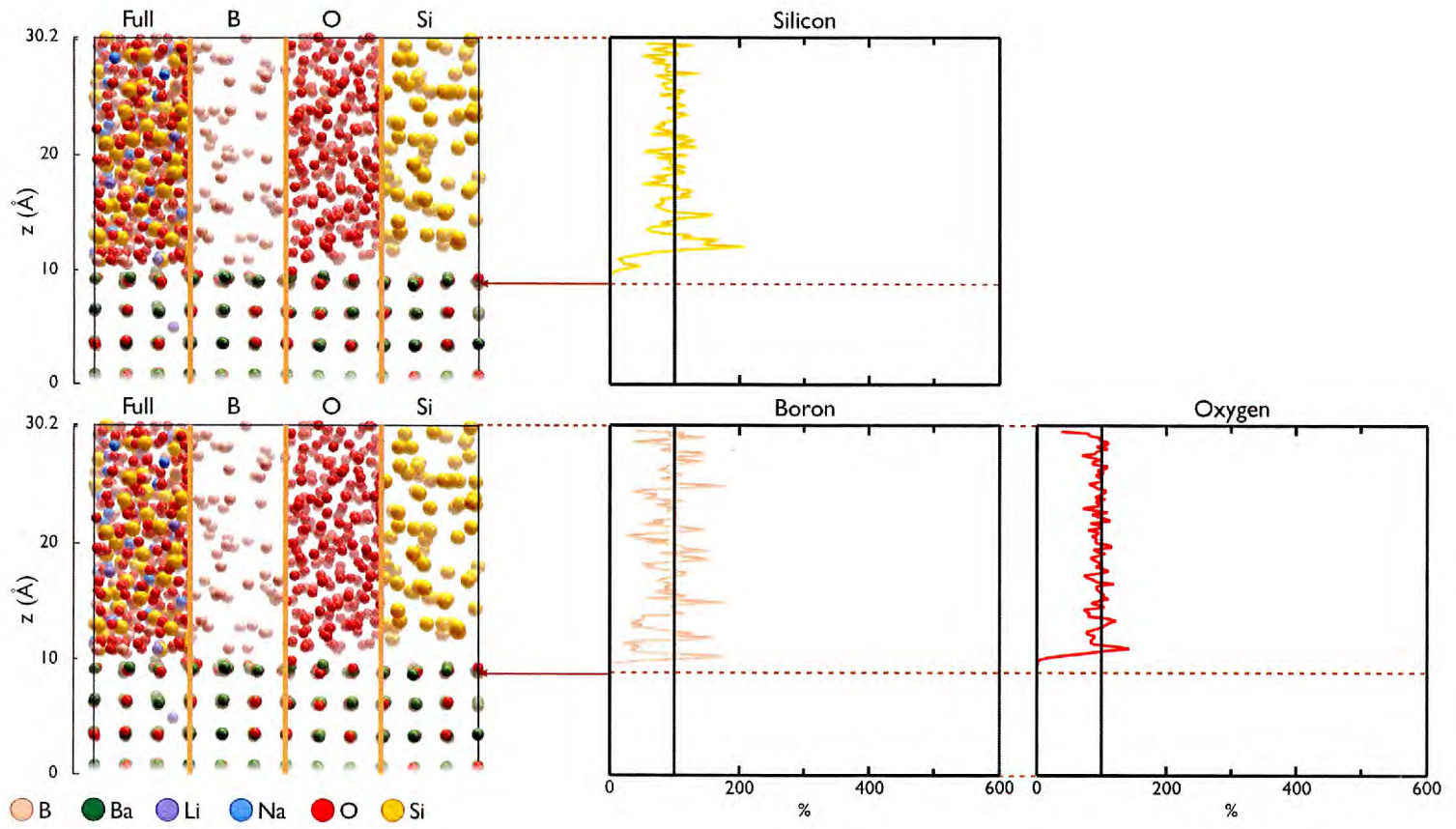
Figure 5.7: Network Former Concentration Profile: MW glass BaO-(100).
