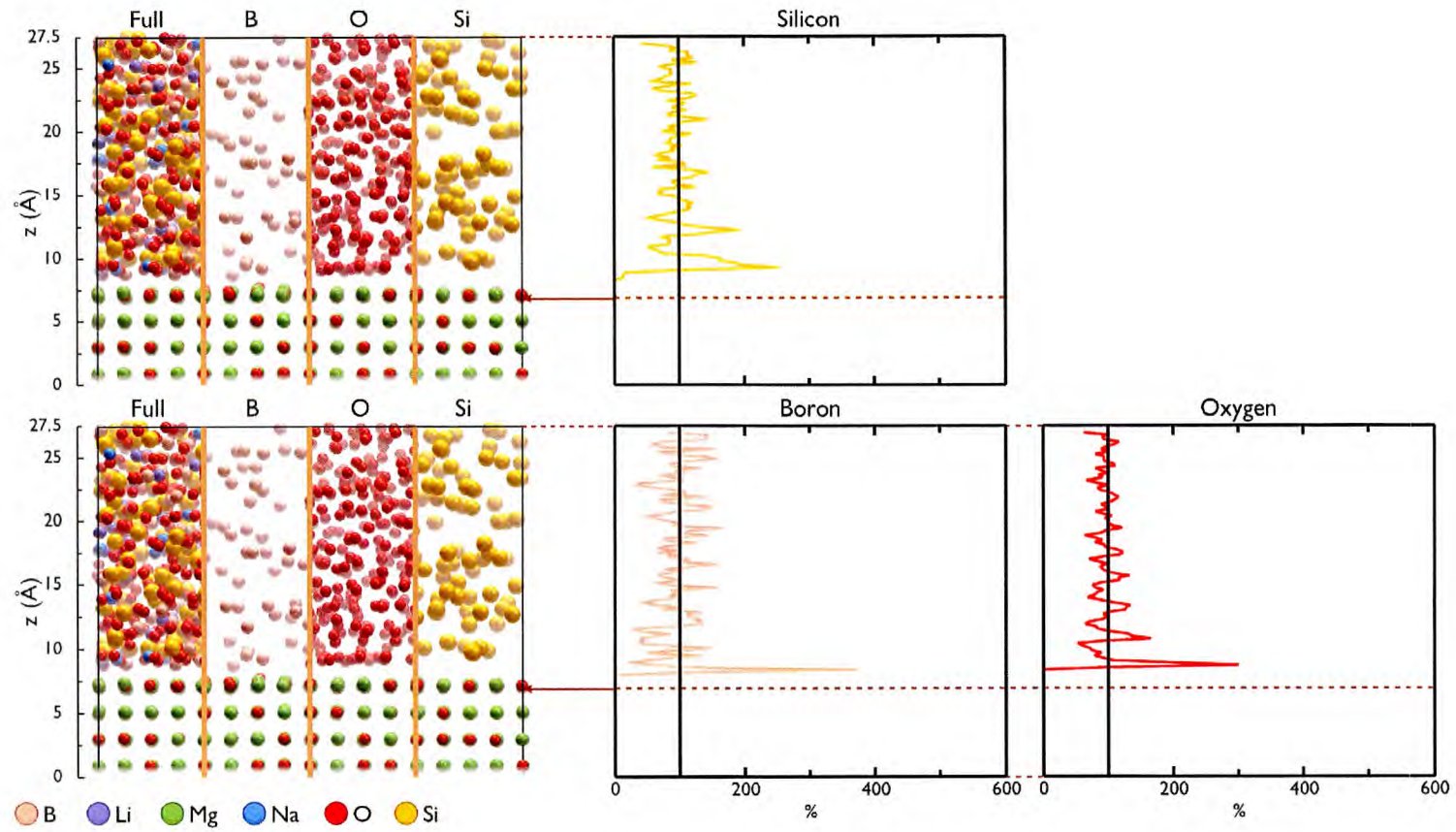
Figure 5.4: Network Former Concentration Profile: MW glass MgO-(100).
