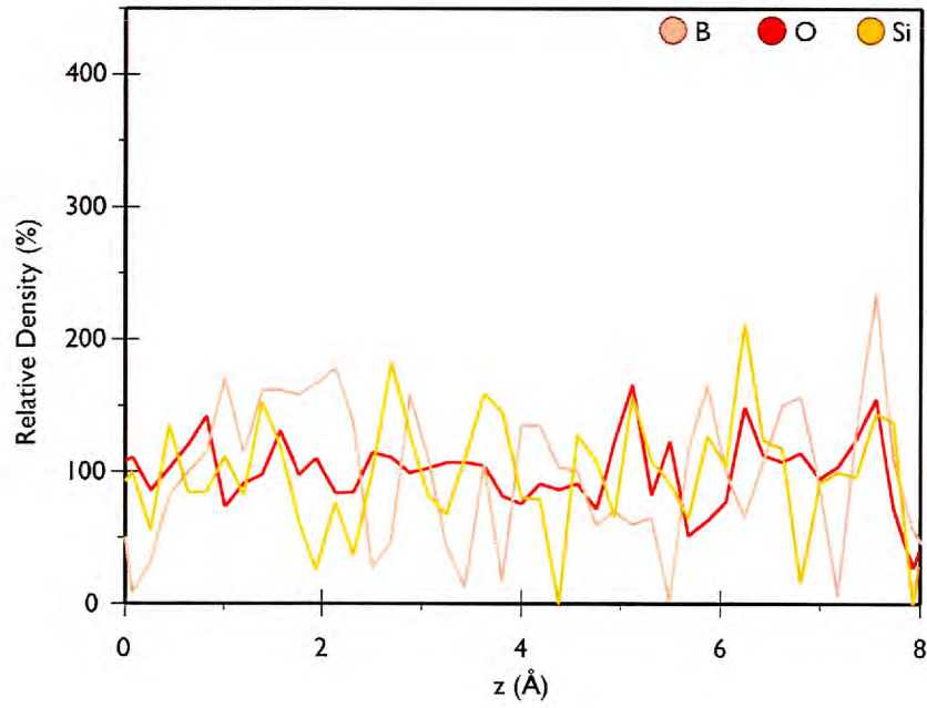
Figure 5.20: Network former density profiles taken along z -axis of MW glass. From this it can be seen that, in the bulk glass, density peaks were randomly distributed and the B, O and Si curves appeared uncorrelated.
