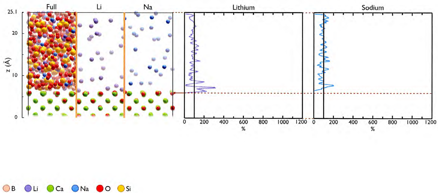
Figure 4.22: Alkali Concentration Profile: MW glass CaO-(110).
