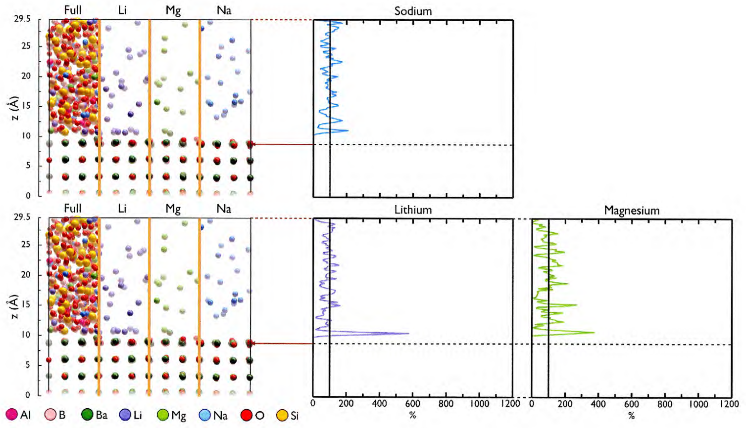
Figure 4.28: Alkali Concentration Profile: MW+Al+Mg glass BaO-(100).
