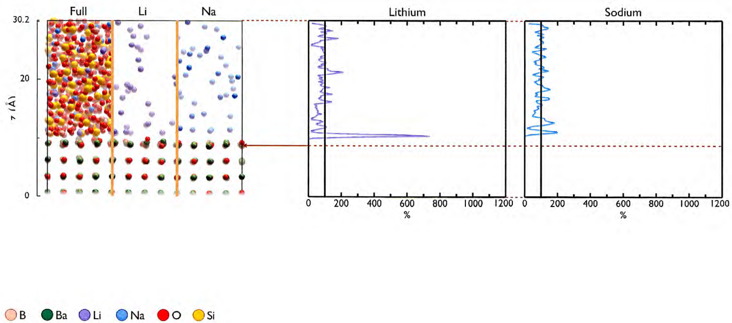
Figure 4.20: Alkali Concentration Profile: MW glass BaO-(100).
