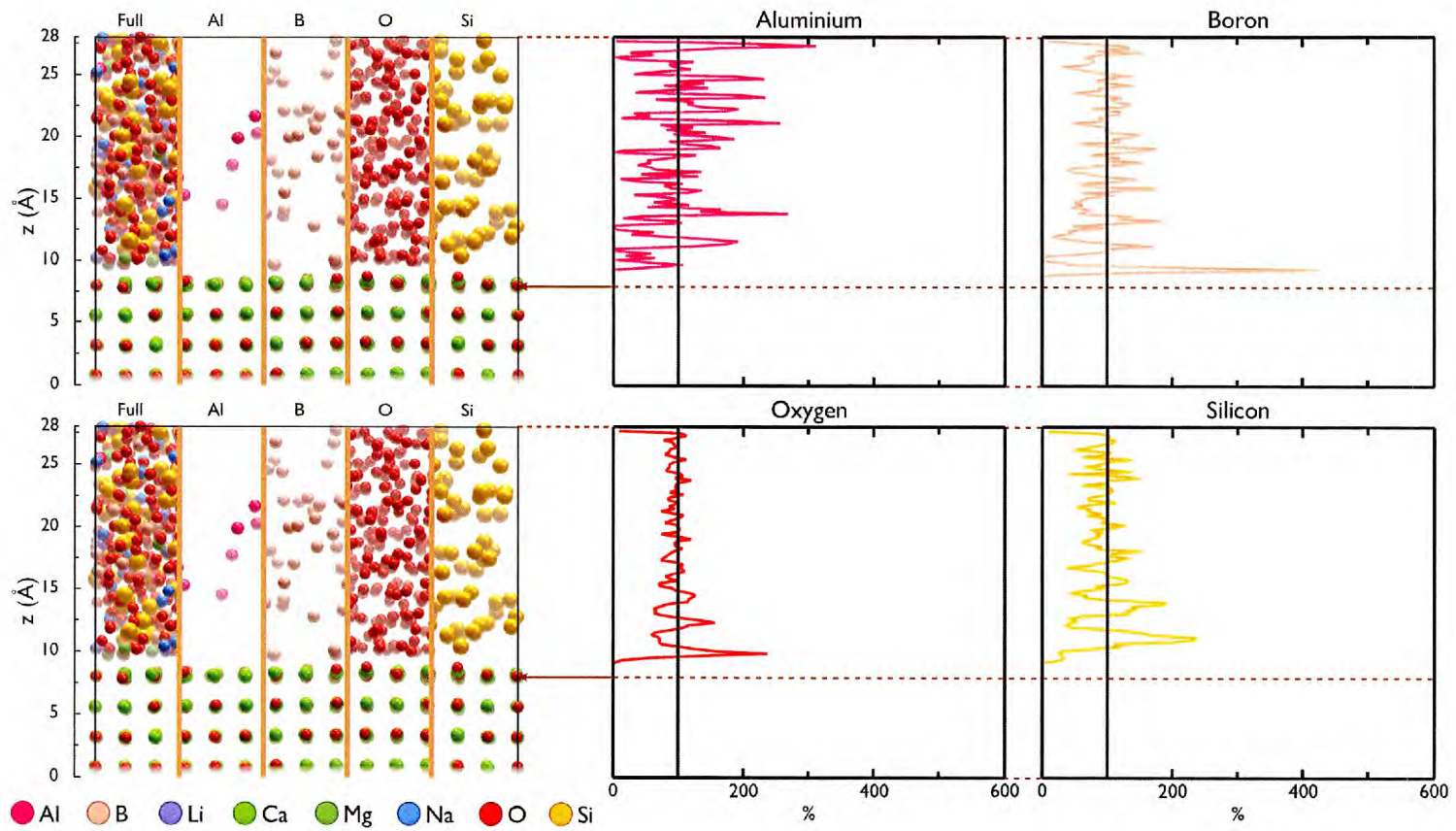
Figure 5.13: Network Former Concentration Profile: MW+Al+Mg glass CaO-(100).
