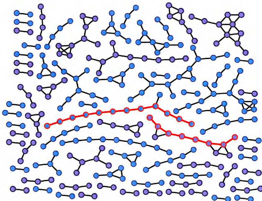
Figure 3.22: Graph showing topography of MW glass alkali network, longest paths, containing most inter-site hops, are highlighted in red for each alkali species (Li-●,Na-●).
