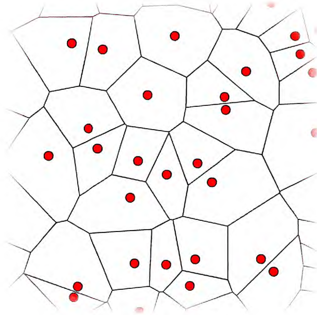
Figure 3.9: Voronoi diagram for a random set of points.
