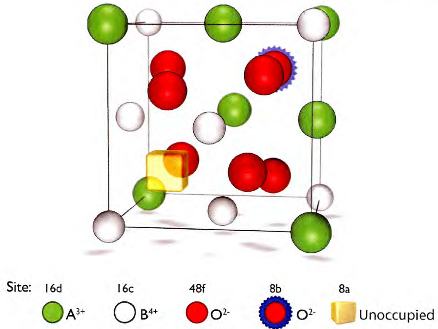
Figure 6.3: One eighth of the full pyrochlore unit cell, showing relaxation of anions towards unoccupied 8a site.
