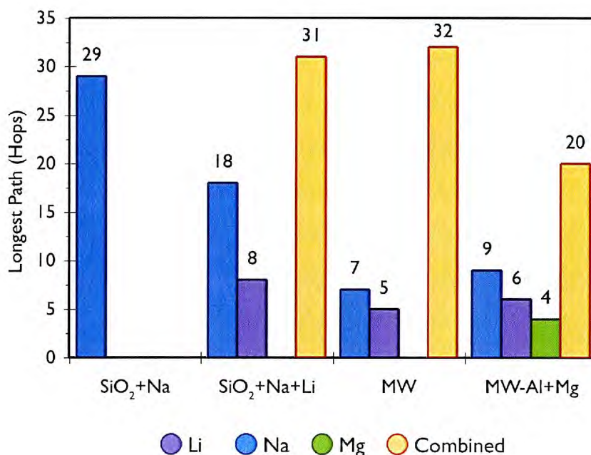
Figure 3.24: Longest paths measured in hops.
