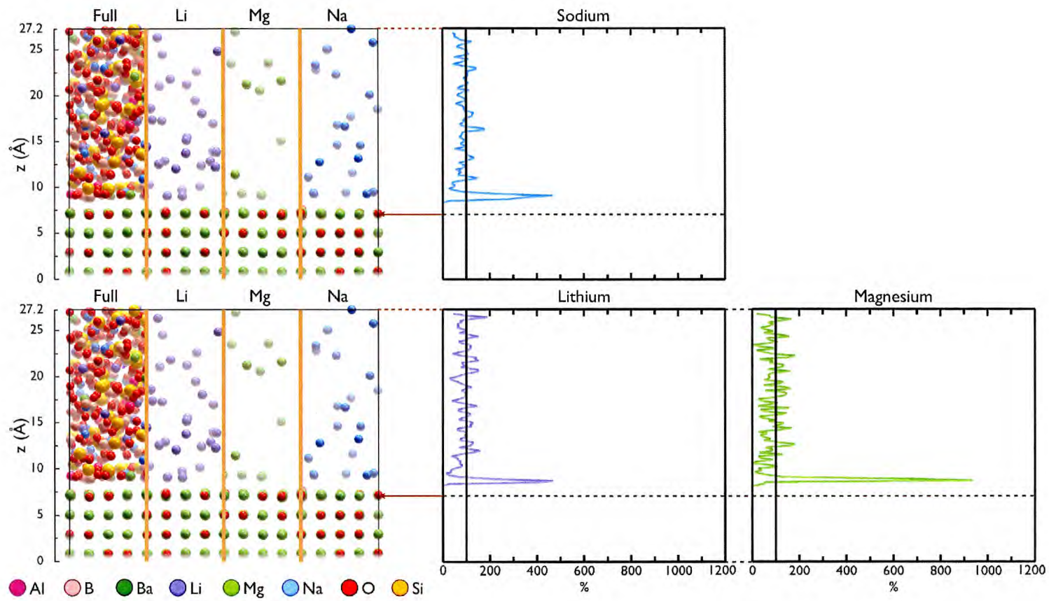
Figure 4.25: Alkali Concentration Profile: MW+Al+Mg glass MgO-(100).
