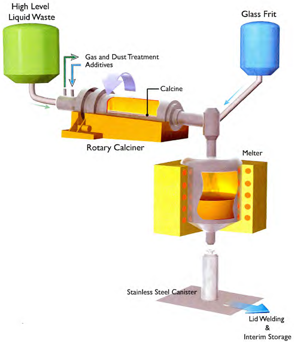
Figure 1.1: Schematic diagram of a typical rig used to immobilise high level nuclear waste.
