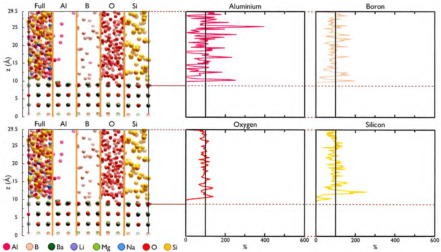
Figure 5.15: Network Former Concentration Profile: MW+Al+Mg glass BaO-(100).
