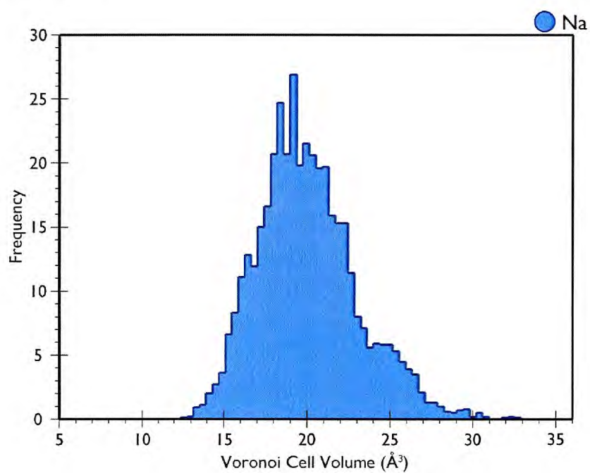
Figure 3.12: Histogram of Voronoi cell volumes for alkali species in \text{SiO}_2+\text{Na} glass.
