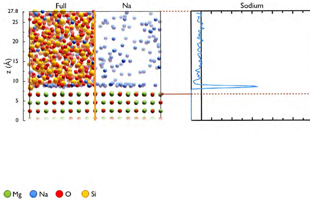
Figure 4.15: Alkali Concentration Profile: \text{SiO}_2+\text{Na MgO} -(100).
