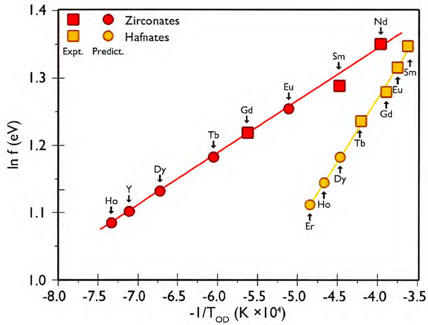
Figure 6.9: Plot of \ln(f) vs. -\frac{1}{T} (hafnate data taken from [168]).
