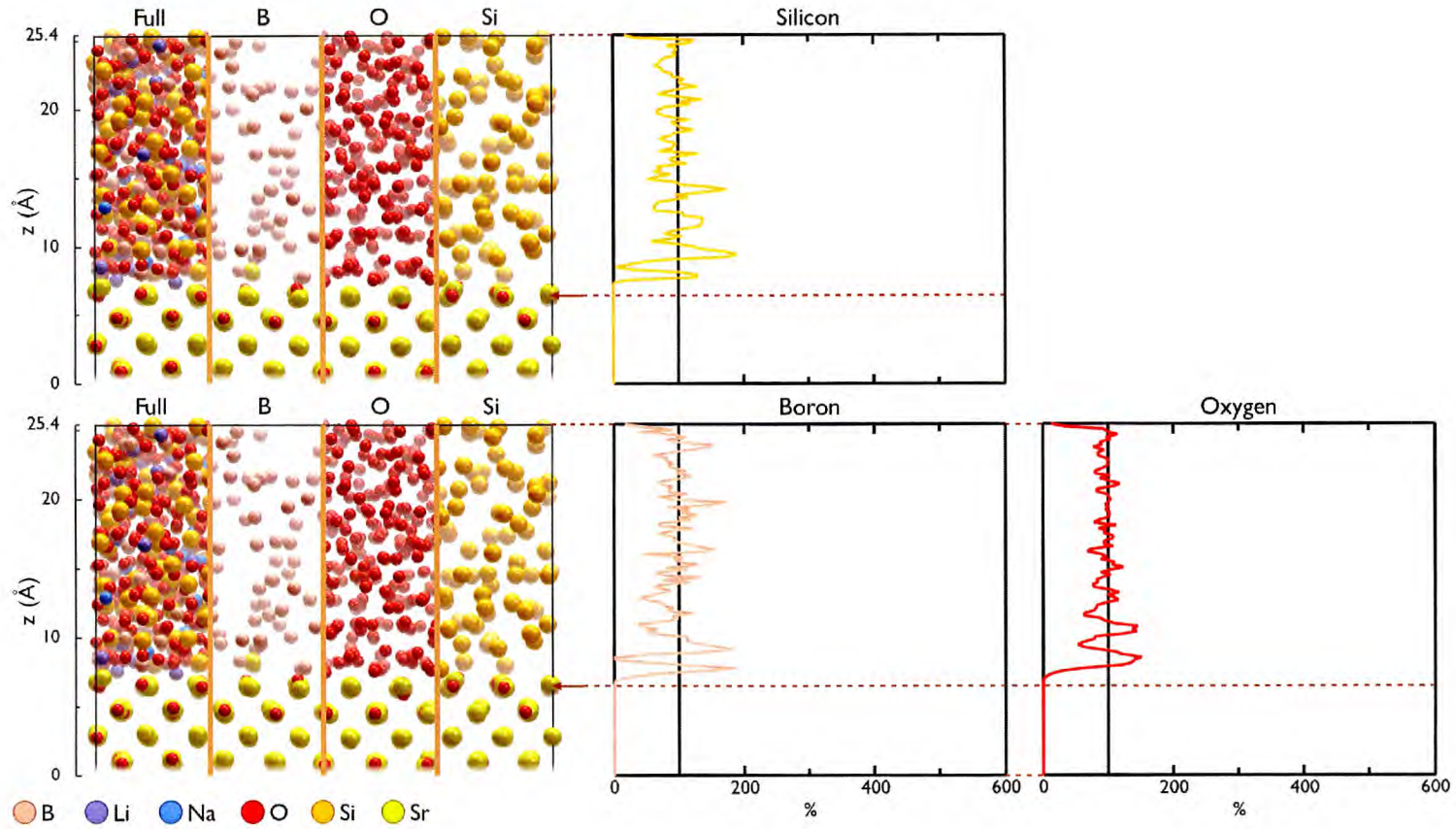
Figure 5.10: Network Former Concentration Profile: MW glass SrO-(110).
