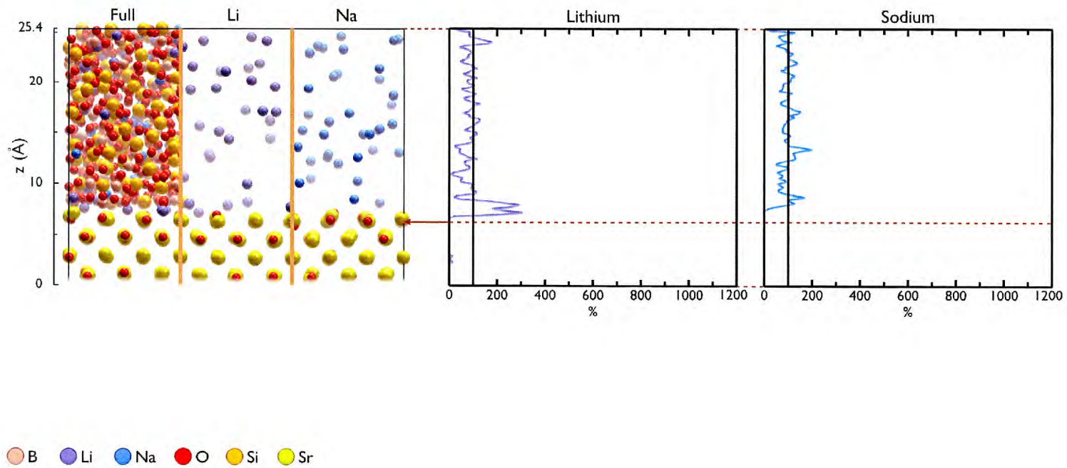
Figure 4.23: Alkali Concentration Profile: MW glass SrO-(110).
