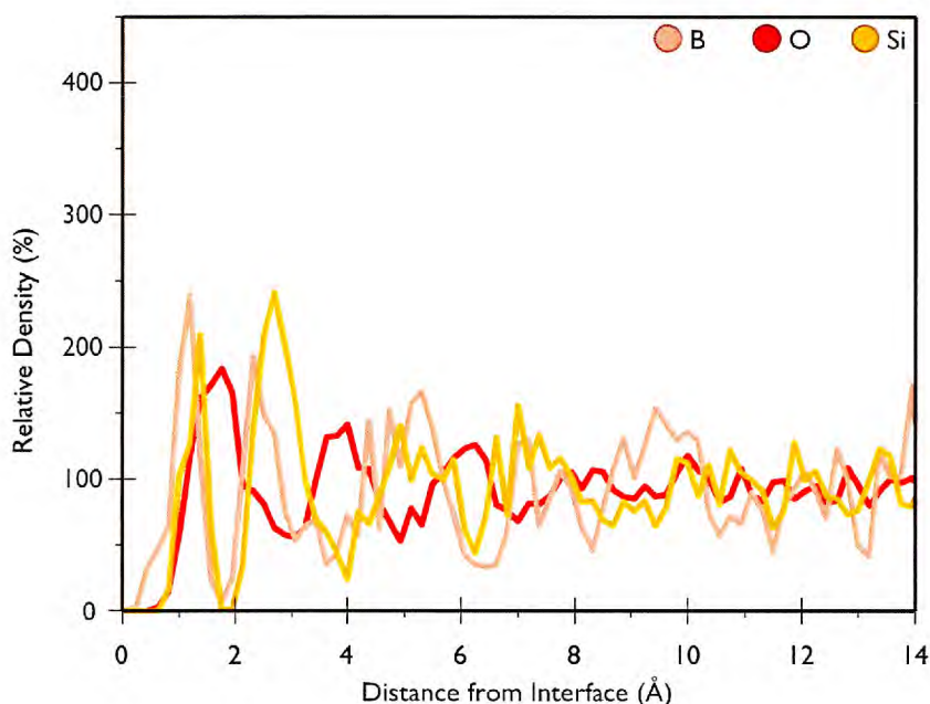
Figure 5.22: Density profile for network formers at interface between MW-glass and (110) surface of CaO.
