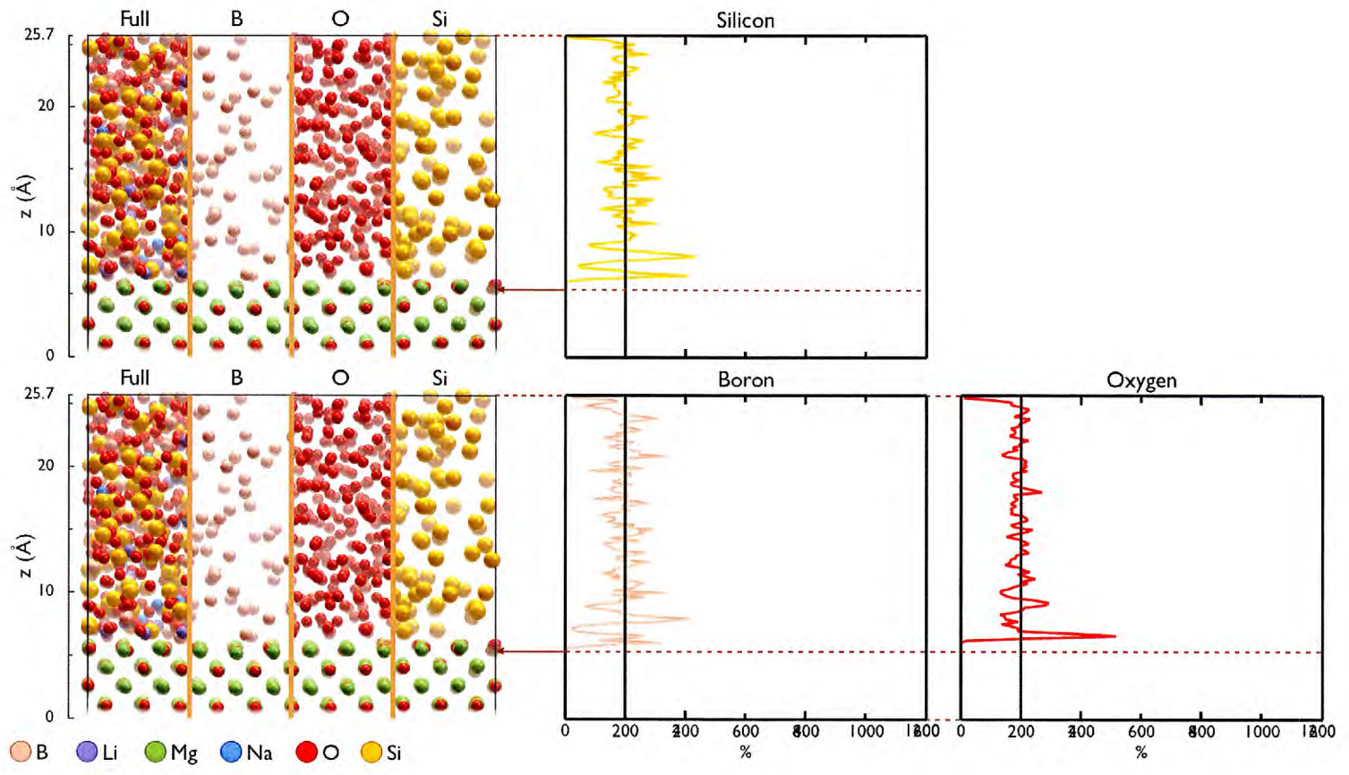
Figure 5.8: Network Former Concentration Profile: MW glass MgO-(110).
