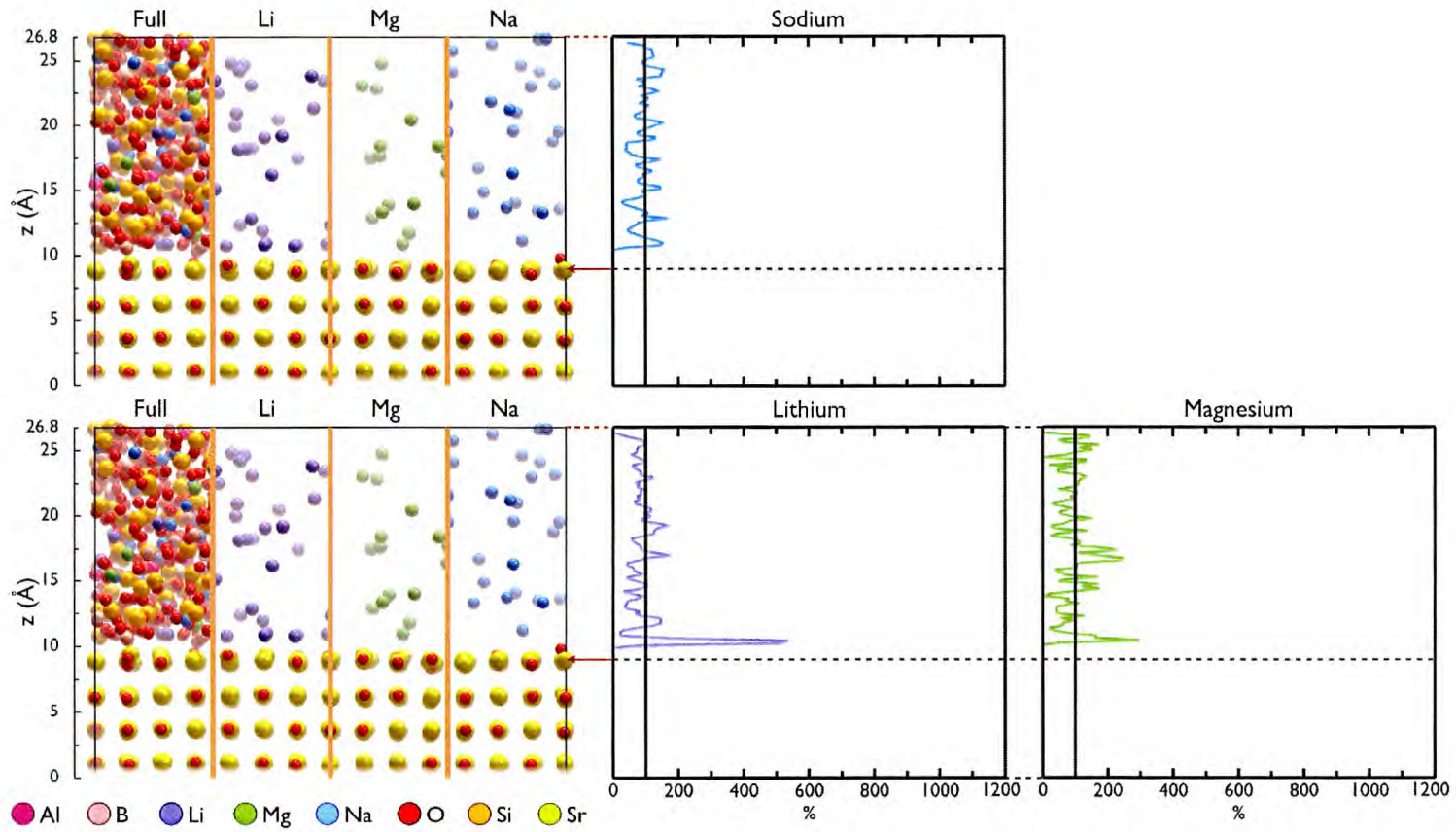
Figure 4.27: Alkali Concentration Profile: MW+Al+Mg glass SrO-(100).
