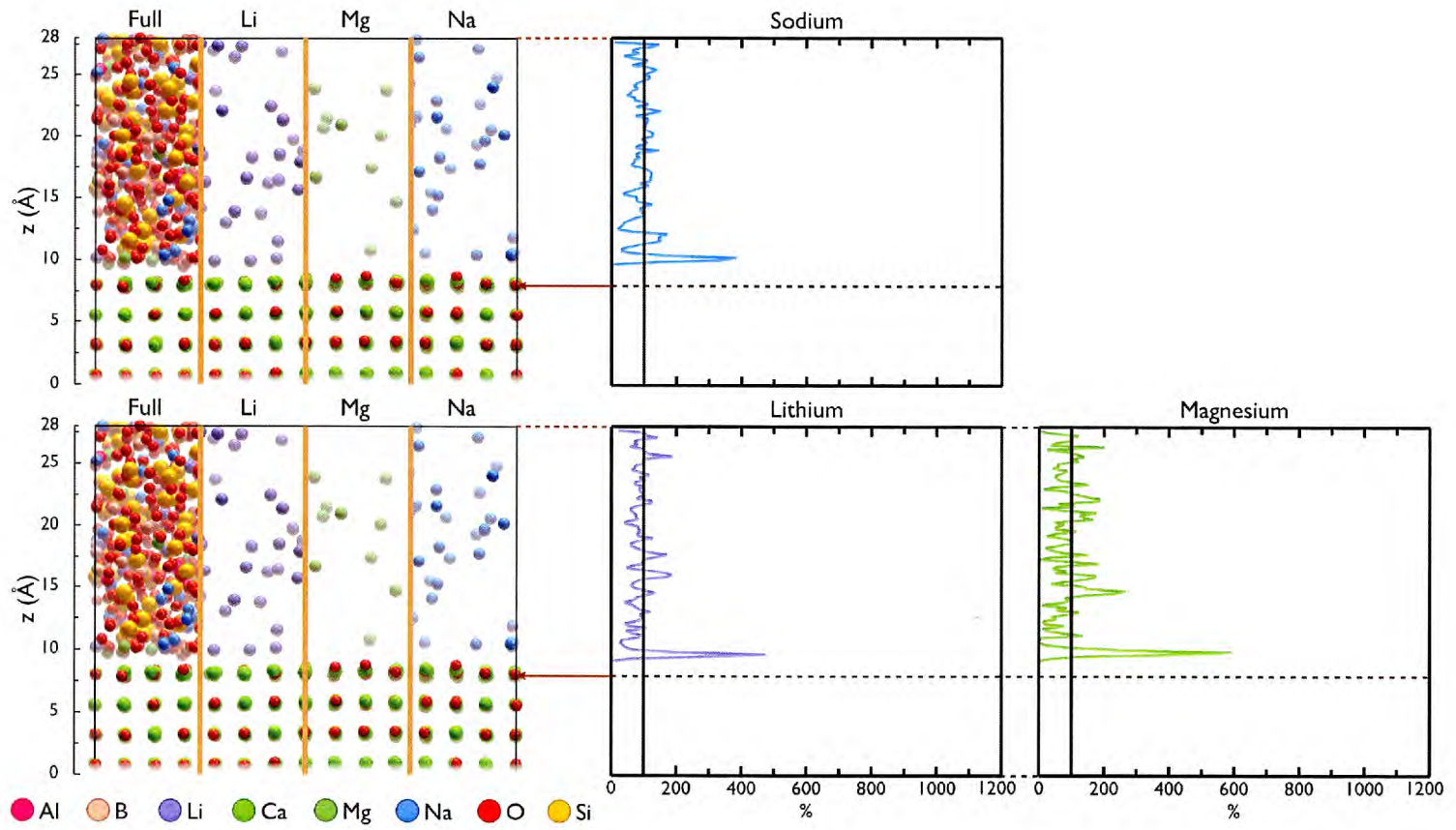
Figure 4.26: Alkali Concentration Profile: MW+Al+Mg glass CaO-(100).
