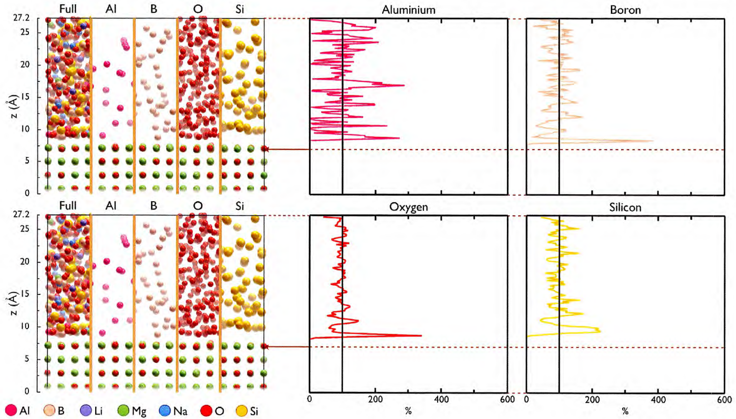
Figure 5.12: Network Former Concentration Profile: MW+Al+Mg glass MgO-(100).
