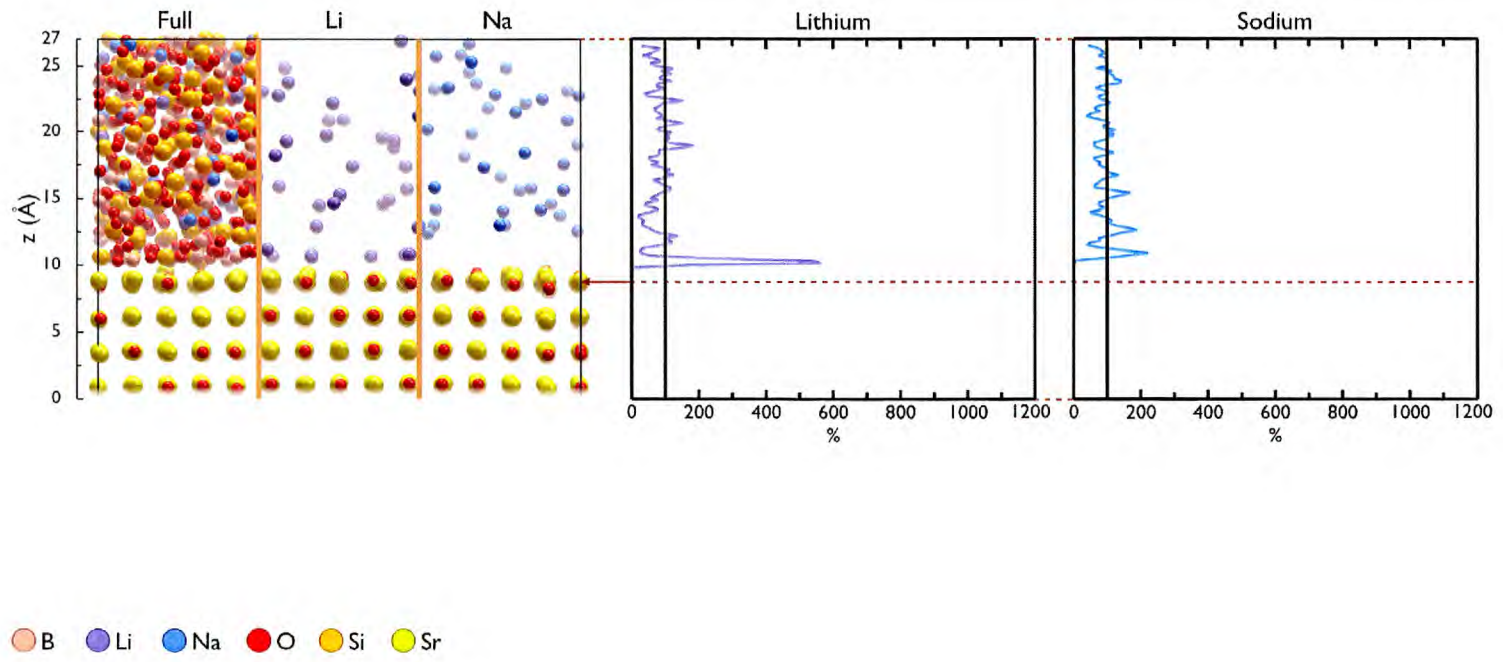
Figure 4.19: Alkali Concentration Profile: MW glass SrO-(100).
