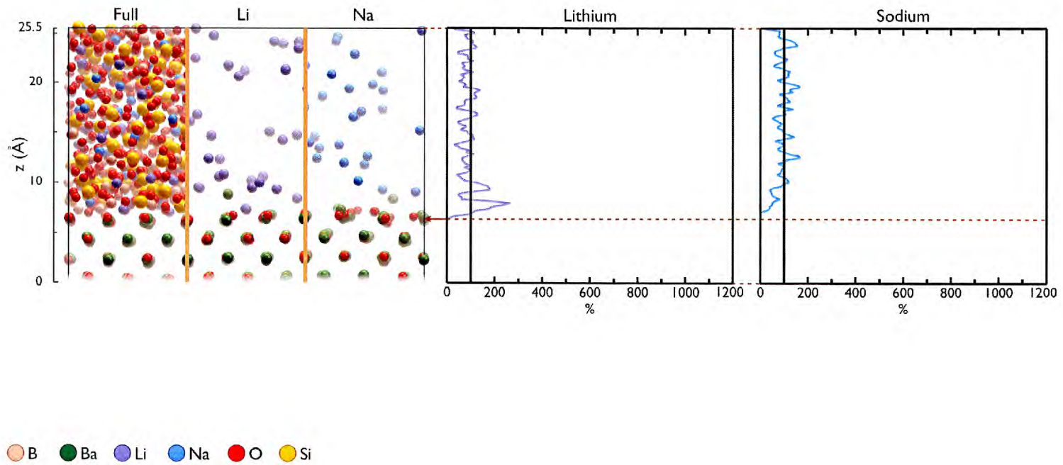
Figure 4.24: Alkali Concentration Profile: MW glass BaO-(110).
