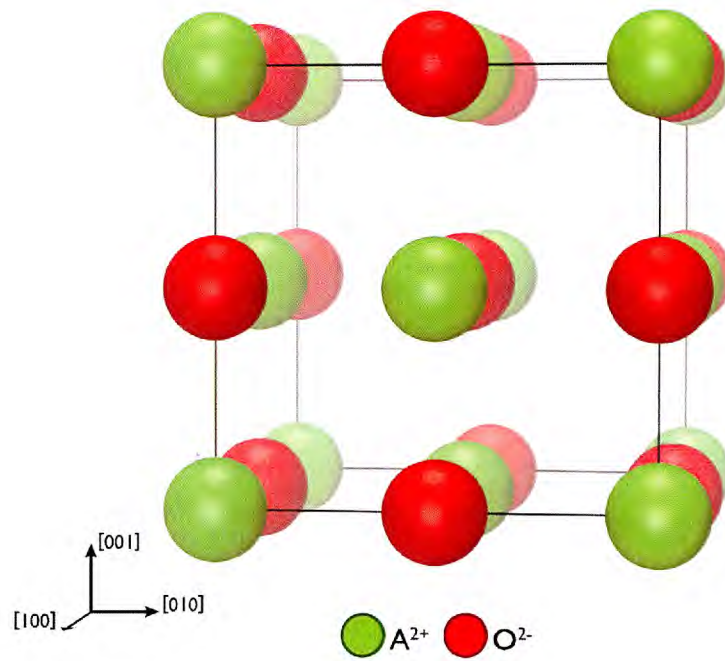
Figure 2.3: Unit cell of the A^{2+}O^{2-} rock-salt structure.
