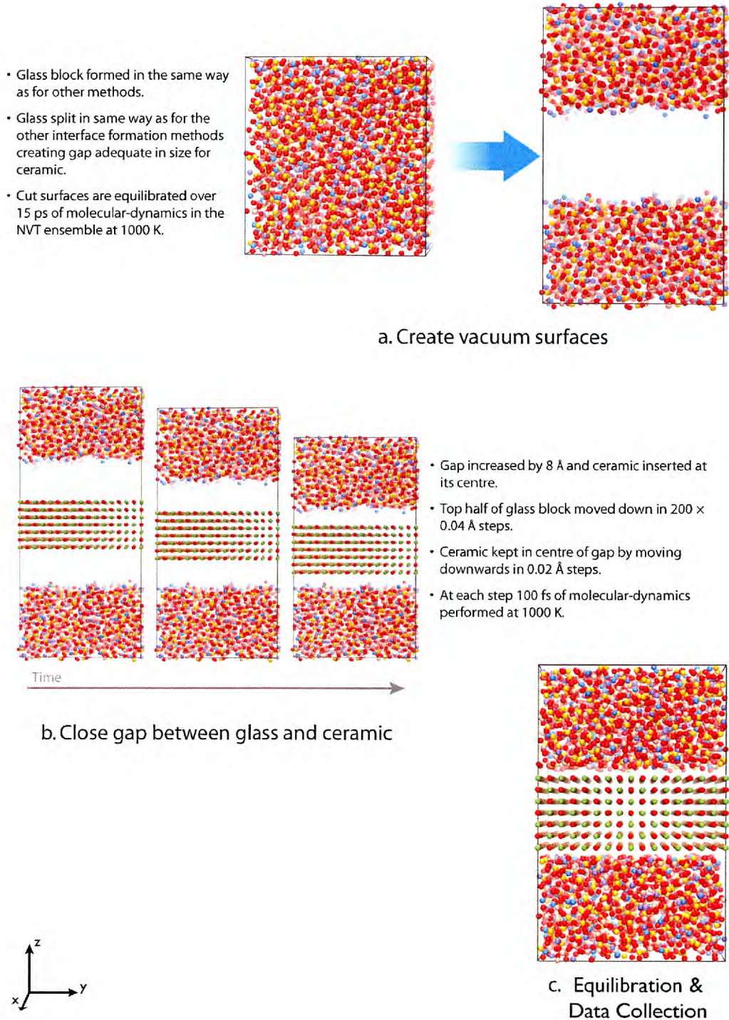
Figure 2.6: Gap close method for glass ceramic interface formation.
