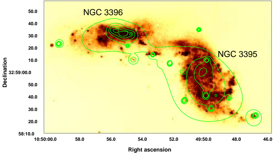
Figure 2. Contours of adaptively smoothed 0.3–8.0 keV X-ray data from Chandra ASIC-S overlaid on an optical image from the Palomar 5m telescope. Contours increase by a factor of \sqrt{2} . The nuclei of the galaxies are separated by 90 arcseconds.
