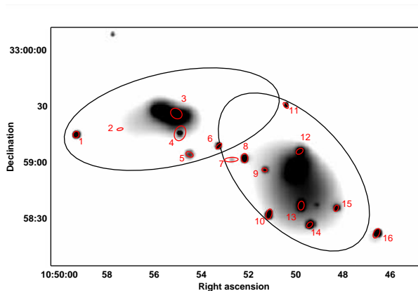
Figure 4. The sources detected by Chandra overlaid on a grey-scale image of the X-ray emission across the full band. The extent of the D 25 ellipses is also shown.
