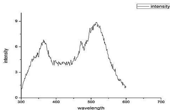
Fig. 6 – Photoluminescence spectra of CdS deposited on glass
