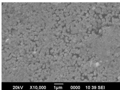
Fig. 1 – SEM image of CdS nanoparticles deposited on glass at 10,000x magnification
