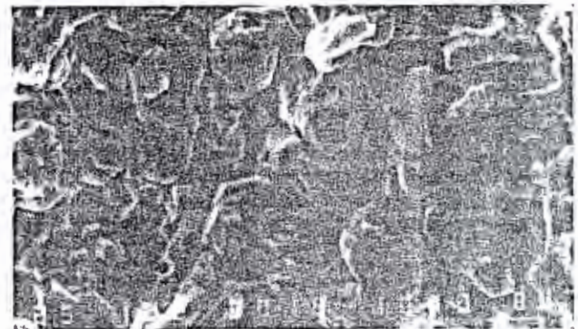
Fig.4. SEM micrograph of the steel surface after zinc electrodeposition in acid chloride solution without additive. (a) x 40 (above) (b) x 480 (above, right) (c) x 1000 (right)
