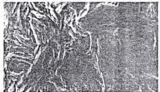
Fig.5. SEM micrographs showing the effect of thiourea and dextrin additives on the electrodeposition of zinc. (a) x 40 (above) (b) x 480 (above, right) (c) x 1000 (right)
