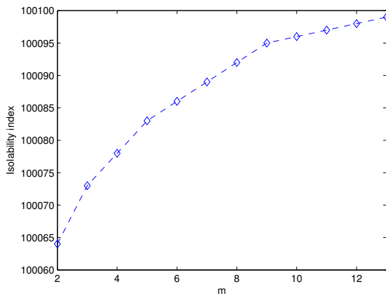
Fig. 4. Fault diagnosis performance tradeoff
