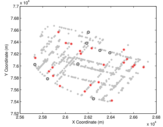
Fig. 3. DMA network with the optimal sensor location (black \circ symbol) and the remaining candidate sensors (red * symbol)
