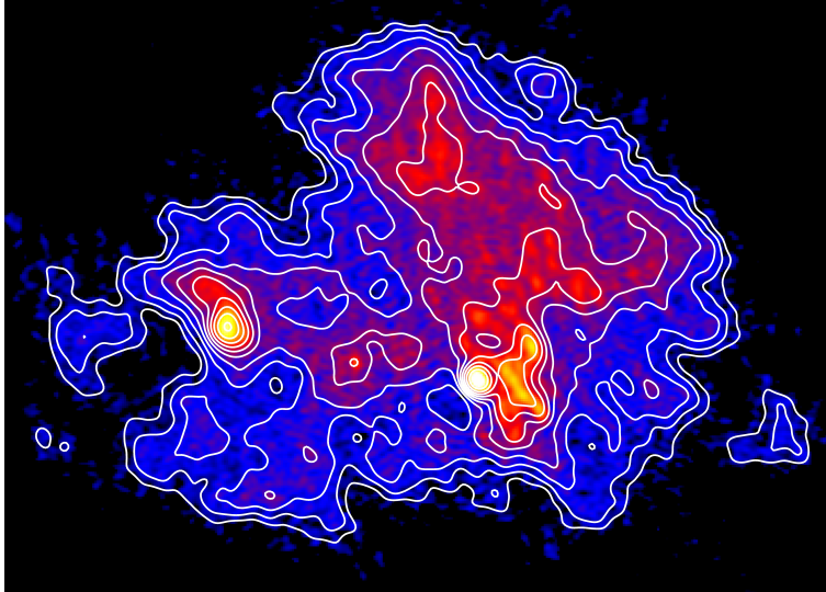
Figure 2. A 135 MHz LOFAR image of the rich X-ray cluster of galaxies A2256 at z = 0.058 . The image has been made from data that were taken with 10 core stations and 5 remote stations. Only 4 MHz bandwidth out of a total 48 MHz was used during the reduction. The resolution of the image is about 31 \times 19 arcsec and the noise is \sim 5 mJy/beam. Beside several tailed galaxies and the relic structures, the image shows for the first time a spatially resolved central halo of A2256 at low frequencies.
