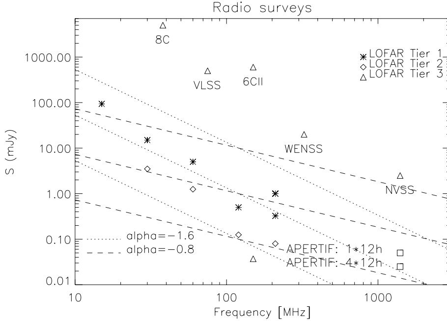
Figure 1. Flux limits (5 sigma) of the proposed LOFAR and APERTIF surveys compared to other existing radio surveys. The triangle represent existing surveys: HDF (VLA Richards et al. 2000; WSRT Garrett et al. 2000), WENSS, NVSS, 6C, VLSS and 8C. The lines represent different power-laws ( S \sim \nu^\alpha , with \alpha = -1.6 and -0.8 ) to illustrate how, depending on the spectral indices of the sources, the LOFAR surveys will compare to other surveys.
