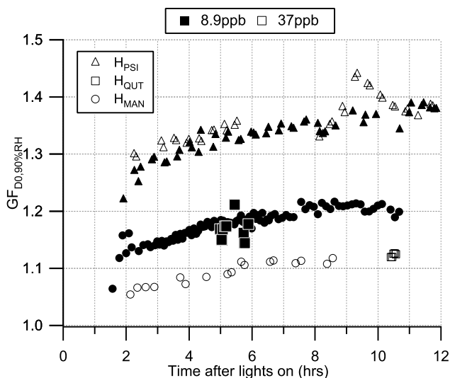
Fig. 2. Unseeded SOA growth factor measurements as a function of time.
