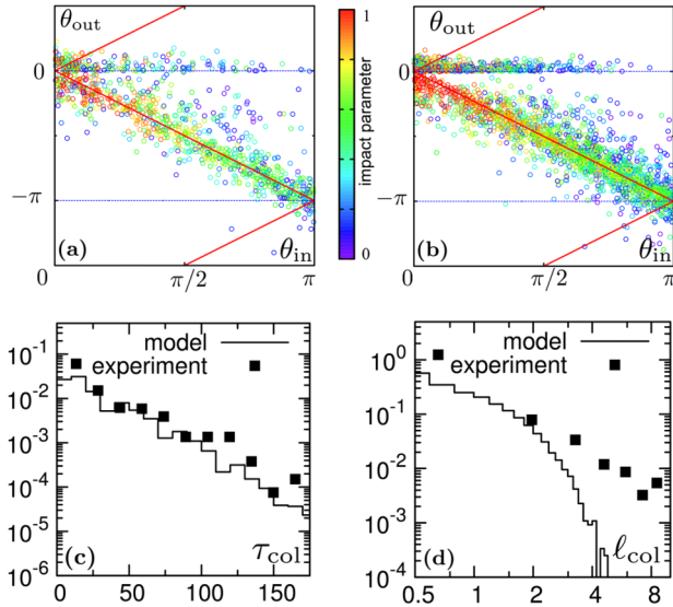
FIG. 3 (color online). Scatter graph \theta_{in} - \theta_{out} for the experiment (a) and our model (b). Values of the impact parameter b are indicated by the color bar. PDF of the duration \tau_{col} (c) [lin-log] and the extension \ell_{col} of a collision (d) [log-log].
