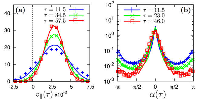
FIG. 2 (color online). (a) PDF of v_{\parallel}(\tau) and (b) PDF of the angle \alpha = \angle(\mathbf{n}(t), \Delta\mathbf{r}(t+\tau)) [lin-log] for selected values of the time increment \tau . Experimental data are indicated with symbols; model data are illustrated with lines.
