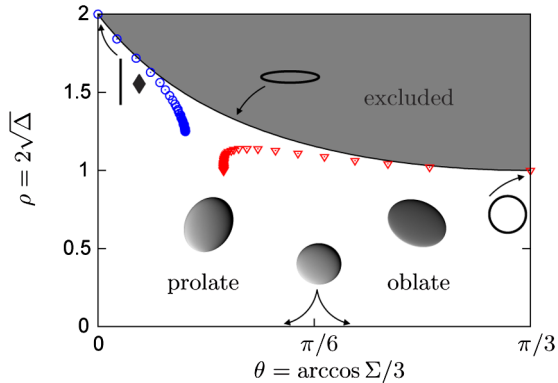
FIG. 1 (color online). The overall shape of polymer configurations depending on the asphericity \Delta and the nature of asphericity \Sigma . Along the solid line the structures are planar; configurations beyond that line are excluded as they do not correspond to real structures. The diamond indicates the peak in the distribution of flexible open polymers. The sequences of circles and triangles denote the mean shapes of open and ring polymers at integer flexibilities starting from L/l_p = 0 at (0, 2) and at (\pi/3, 1) , respectively.
