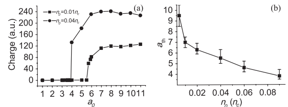
FIG. 3. (a) Charge carried by the AES versus laser amplitude a_0 . In the case of n_0 = 0.04n_c , the laser-target parameters are L_1 = 45\lambda_L and \tau_L = 10T_L , while for n_0 = 0.01n_c they are L_1 = 80\lambda_L and \tau_L = 14T_L . (b) Threshold laser amplitude a_{th} versus the plateau density n_0 .
