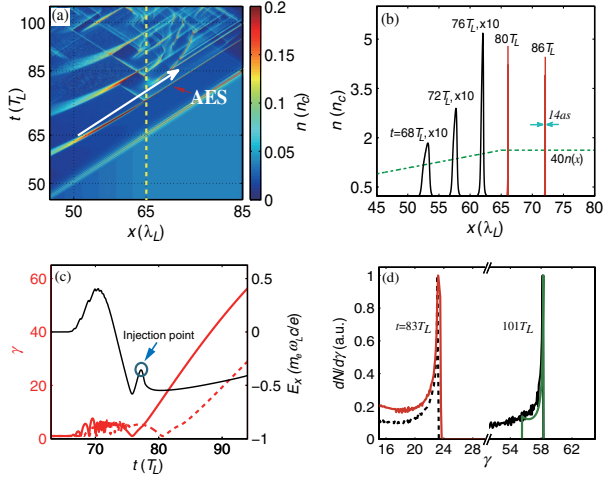
FIG. 2 (color online). Results of 1D PIC simulation. (a) Spatial-temporal plot of the electron density. The dashed line marks the UPT at x = 65\lambda_L , and the white arrow is parallel to x = t . (b) The first density wave crest before (black curve) and after (red curve) the transition. The dashed line shows the initial target profile. (c) Temporal evolution of the experienced electric field E_x (black curve) and the \gamma factor (red curve) for AES electrons. The solid curves are for n_0 = 0.04n_c and the dashed curve for n_0 = 0.02n_c . (d) Energy spectra of the trapped electrons at t = 83T_L and t = 101T_L . The black curves are 1D results, the red curve is a 2D result, and the green curve is obtained according to Eq. (2) at t = 101T_L .
