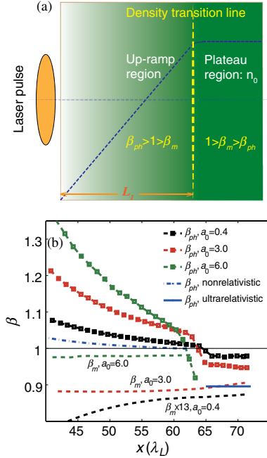
FIG. 1 (color online). (a) Schematic of AES generation. Localized electron injection occurs as \beta_{\text{ph}} , at which the apex of the first wakefield bucket is moving, undergoes a fast switch from above to well below unity near the UPT. (b) Evolution of \beta_{\text{ph}} and \beta_m from 1D PIC simulations, where the initial plasma density rises linearly from zero at x = 20\lambda_L to 0.04n_c at 65\lambda_L and then keeps constant.
