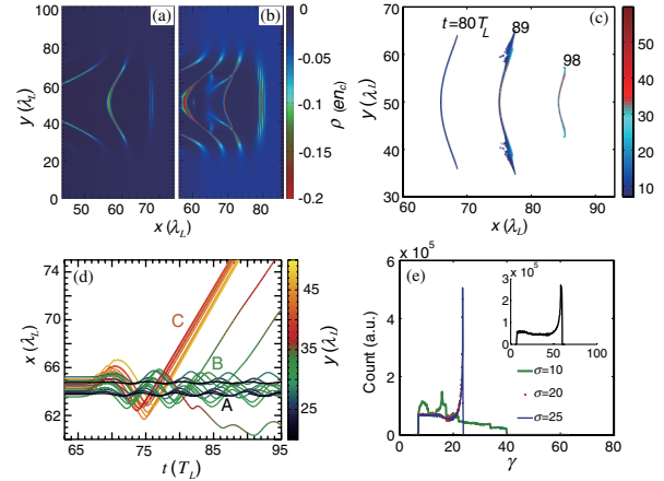
FIG. 4 (color online). Results of 2D PIC simulation. Snapshots (a) and (b) show the electron density at t = 71T_L and t = 83T_L , respectively. (c) Snapshots of the trapped electrons (colored according to \gamma - 1 ) during acceleration. (d) Particle-tracking plot. It is obtained by first tracking back AES electrons to find their initial x range and then tracking a random sample of 24 electrons within this x range. ( y = 50\lambda_L corresponds to the center axis.) (e) Energy spectra of the trapped electrons for different spot radii at t = 83T_L while keeping the other parameters fixed. The inset shows a spectrum at t = 98T_L for \sigma = 20\lambda_L .
