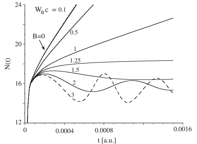
FIG. 1. The final number of created electron-positron pairs as a function of the interaction time for seven different widths of the magnetic field. Parameters used include E = 12.5c^3 , W_E = 0.1/c , and B = 0.6c^3 . B = 0 case is the upper dashed line.
