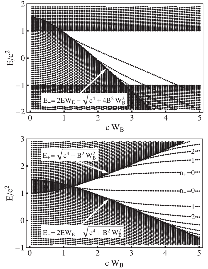
FIG. 2. The energy spectrum of the total Hamiltonian as a function of the spatial size of the magnetic field W_B . All parameters are the same as in Fig. 1 (except the numerical box length is 0.6, instead of 1.0 as used in Fig. 1). The top (bottom) figure shows the spectra for p_y = 0 ( p_y = -BW_B/c ). It is apparent that when W_B > 1.25/c the two continua begin to separate from each other. In the band gap area new discrete energy levels emerge.
