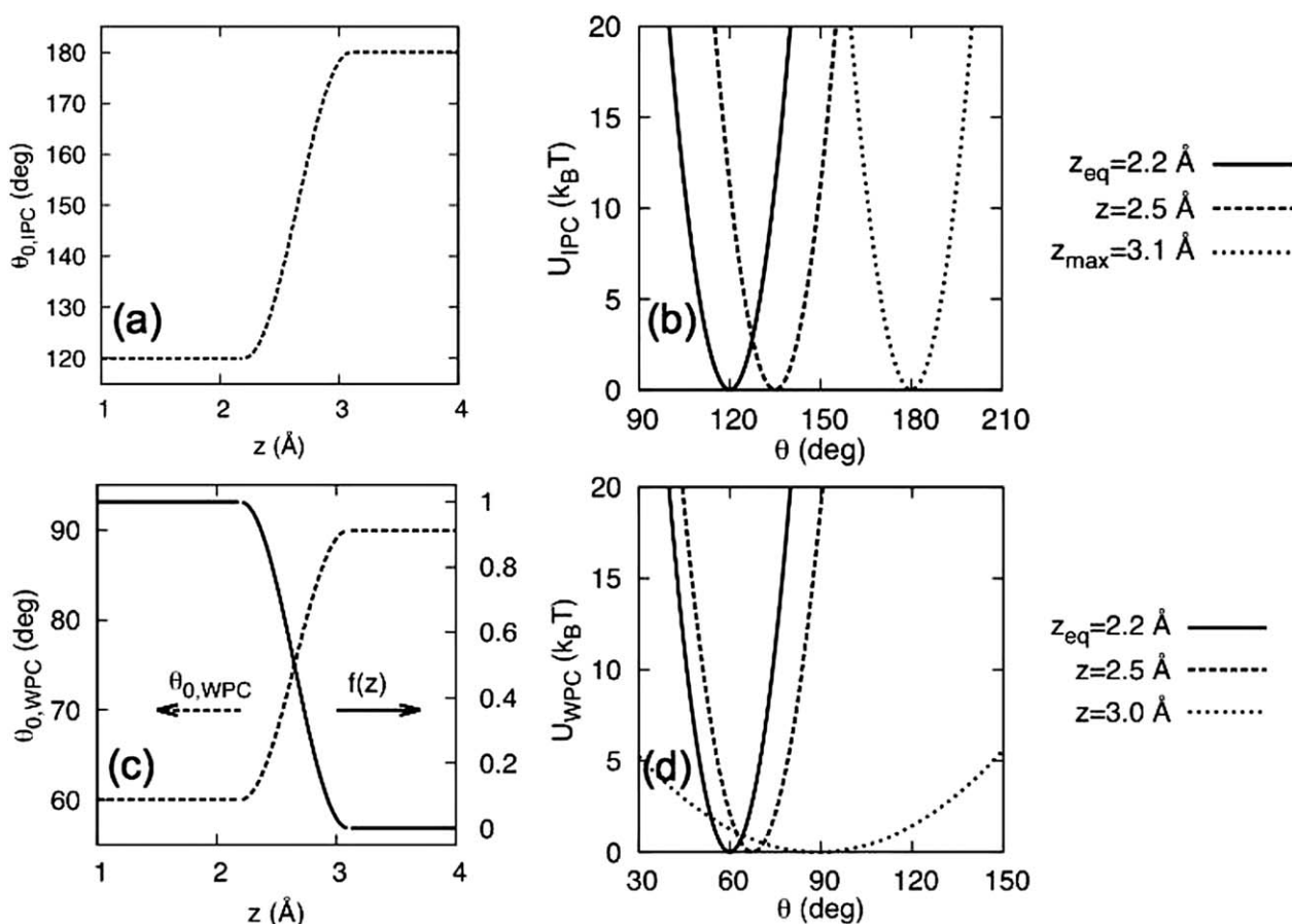
Fig. 5 Angle–distance harmonic potentials for IPC and WPC angles. (a) For the IPC angle the value of \theta_{0,IPC} changes smoothly from 180^\circ to 120^\circ as the P bead approaches the surface. (b) Although \theta_{0,IPC} changes the force constant is independent of distance. (c) For the WPC angle \theta_{0,PCW} changes and the force constant is modified by f(z) . (d) The WPC angle potential becomes flatter as z \rightarrow z_{\max} and is zero for z \geq z_{\max} .
