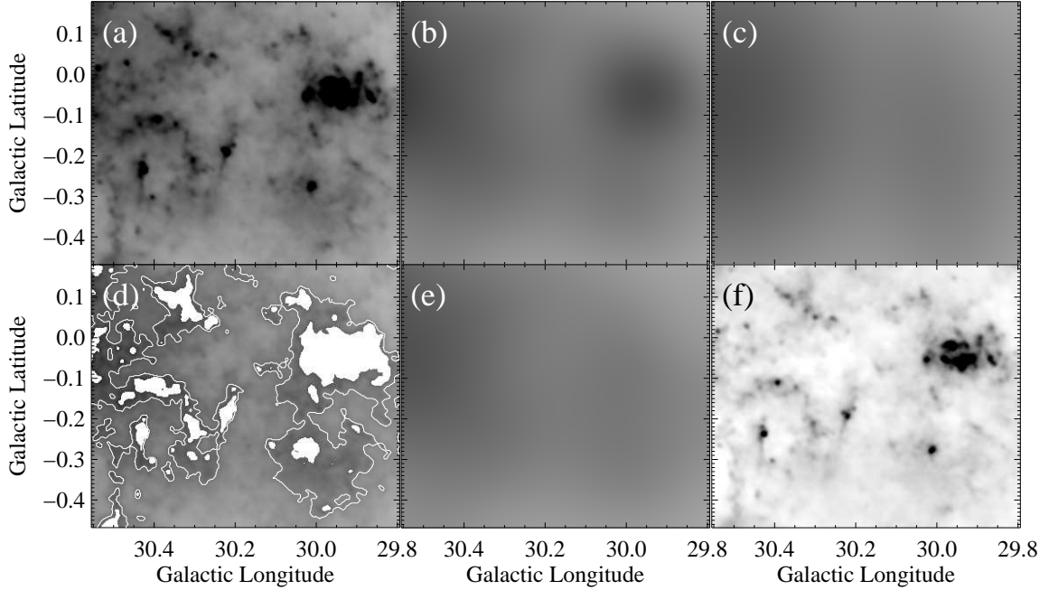
Fig. 2. A depiction of the cirrus subtraction method for the first iteration. Panel (a) is the original SPIRE 500 \mu\text{m} image (all images on the same linear reverse grayscale, from -10 to 900 MJy/sr). Panel (b) is the smoothed (FWHM Gaussian convolution kernel of 12') SPIRE 500 \mu\text{m} image that is used to fit the Gaussian shown in panel (c). Panel (c) is then subtracted from panel (a) to produce a contrast image. A 4.25\sigma cutoff is then applied to the contrast image to produce the source masks shown in panel (d). Panel (d) is the original SPIRE 500 \mu\text{m} image with the sources masked out in white. This is the first iteration source masks; the final source boundaries are shown as white contours. Panel (d) is then convolved with a Gaussian FWHM convolution kernel of 12' with the masks treated as missing data to produce panel (e). Panel (e) is considered the cirrus image for the next iteration. In the next iteration, a Gaussian will be fit to the cirrus image, as a function of latitude at each longitude, and steps b - e will repeat. Panel (f) is the difference image (original SPIRE 500 \mu\text{m} image - convolved cirrus image) that will eventually be used for greybody fitting in the final iteration.
