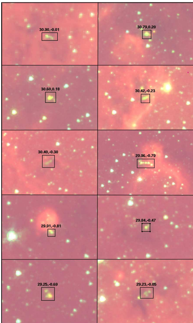
Fig. 8. GLIMPSE 3-color images (Red: 8 \mu\text{m} , Green: 4.5 \mu\text{m} , Blue: 3.6 \mu\text{m} ) of EGOs in the \ell=30^\circ field. The EGOs shown in the right column of the 3rd and 4th row were identified as “possible” EGOs by Cyganowski et al. (2008) and the others were identified by two independent viewers as EGOs as described in Section 3.3. The positions are listed in Table 1.
