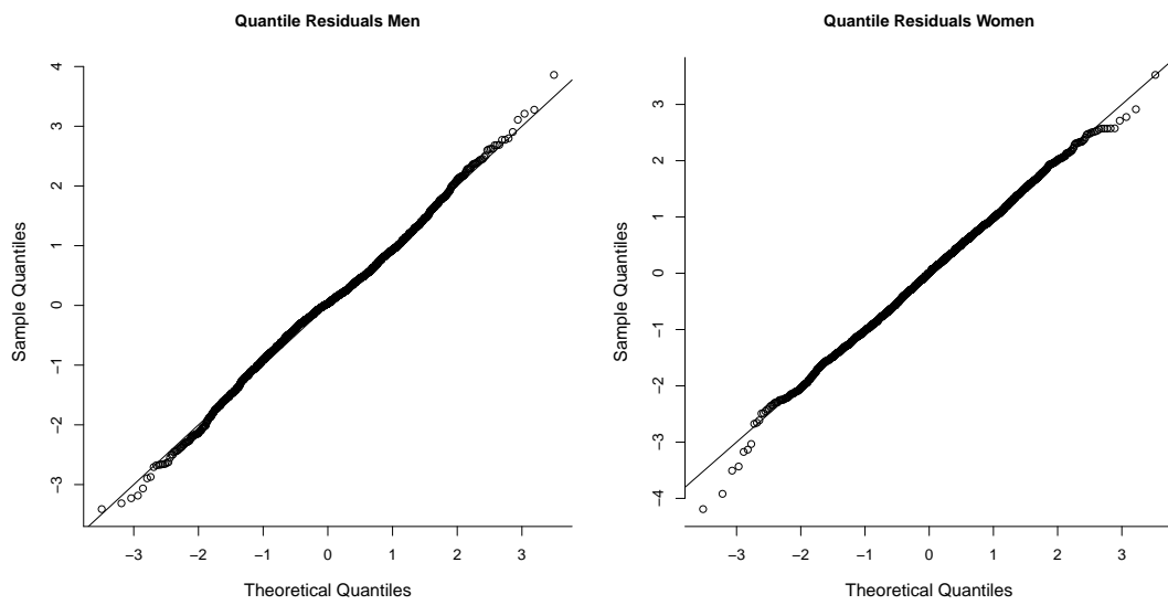
Figure 4.16: Childcare: Quantile Plots for the Poisson-Gamma Model
