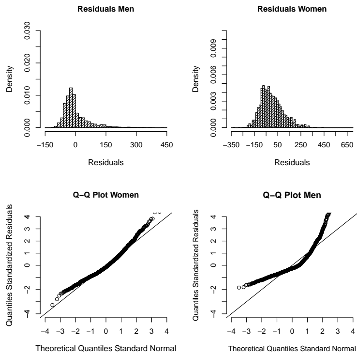
Figure 4.13: Childcare: Evaluation of the Linear Model
