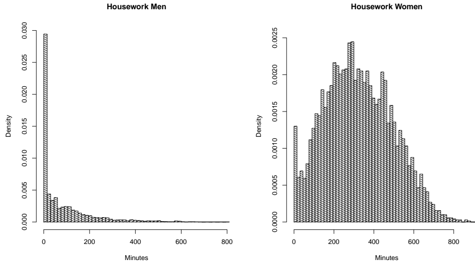
Figure 4.7: Time Devoted to Housework by Couples with Children: Empirical Density
