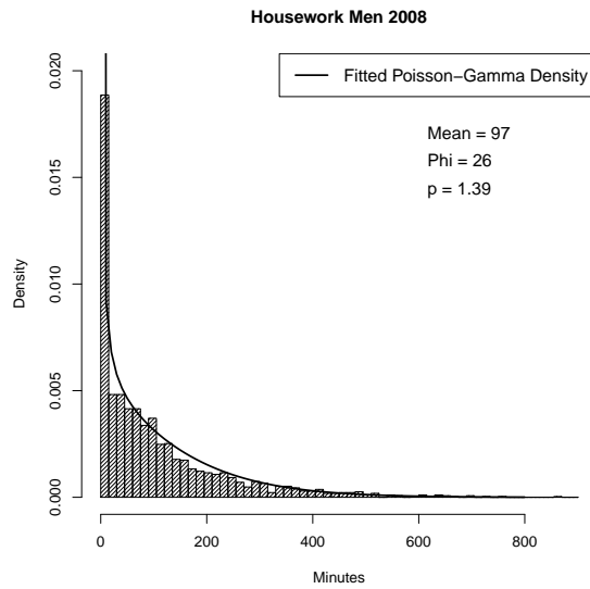
Figure 3.5: Empirical Density of Housework and Fitted Poisson-Gamma Distribution: Men 2008
