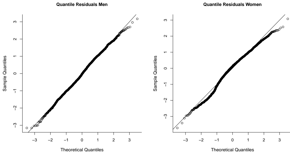
Figure 4.15: Childcare: Quantile Residuals for the Negative Binomial Model
