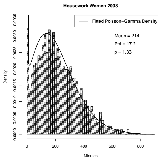
Figure 3.6: Empirical Density of Housework and Fitted Poisson-Gamma Distribution: Women 2008
