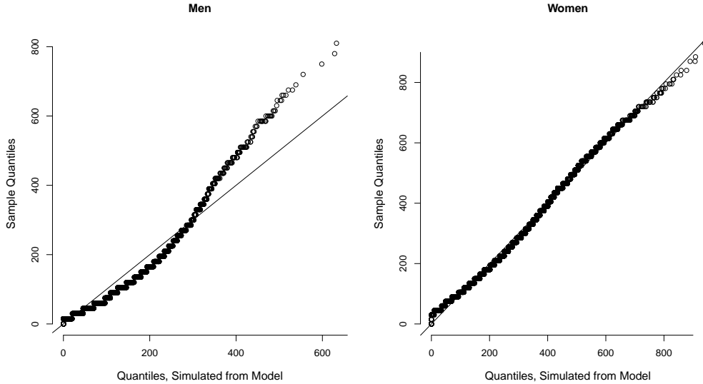
Figure 4.9: Housework: Evaluation of the Tobit Model - Comparison of Survey Data and Simulated Data from the Model
