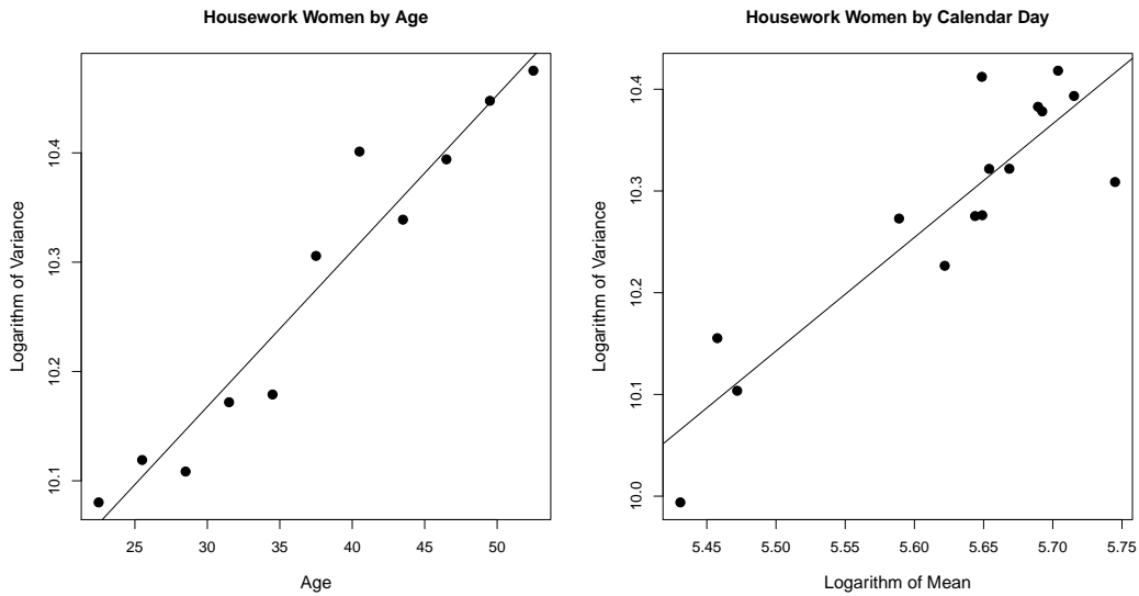
Figure 3.2: Homoscedasticity Diagnostic Plot: Logarithm of Variance vs. Logarithm of Group Means and Age
