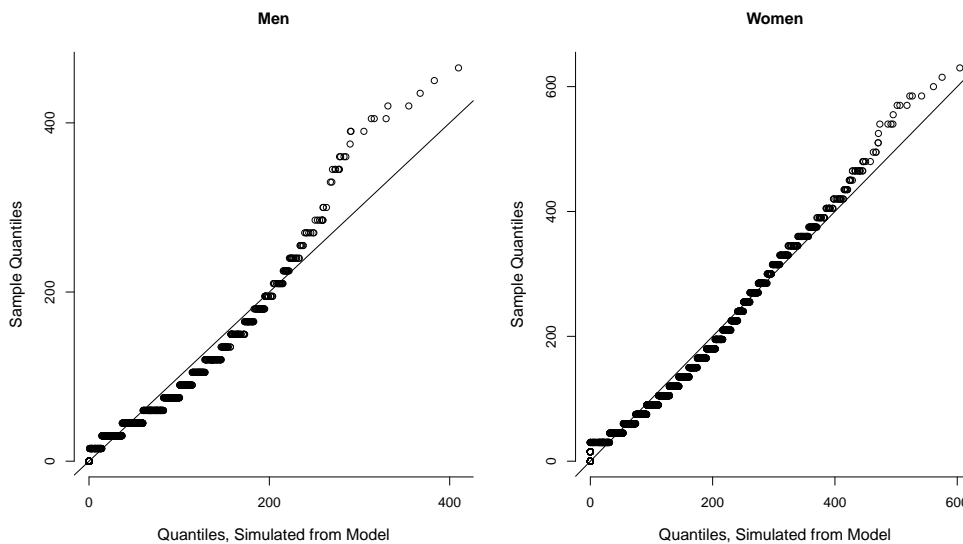
Figure 4.14: Childcare: Evaluation of the Tobit Model
