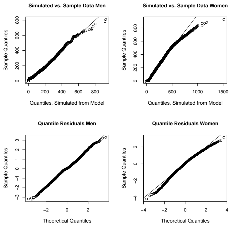
Figure 4.11: Houswork: Evaluation of the Poisson-Gamma Model
