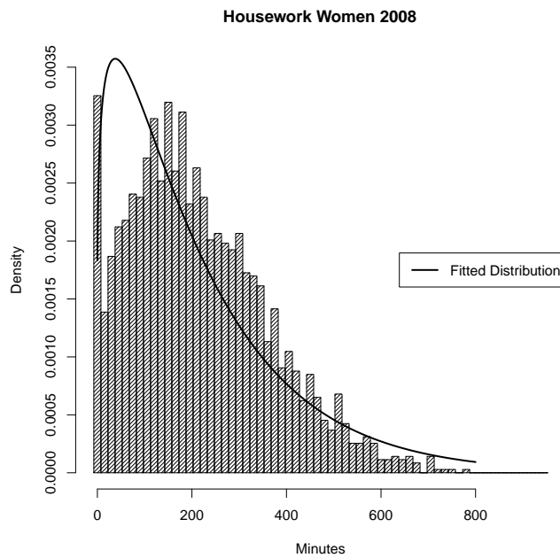
Figure 3.3: Housework of Women: Empirical Distribution and Fitted Negative Binomial Distribution
