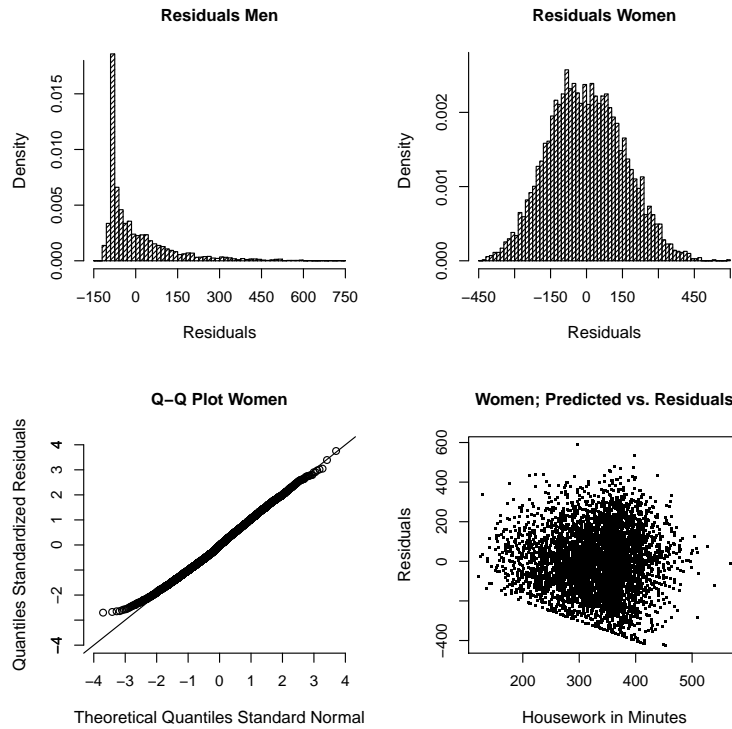
Figure 4.8: Housework: Residual Analysis of the Linear Model
