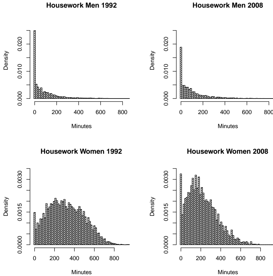
Figure 3.1: Empirical Density of Time Devoted Housework
