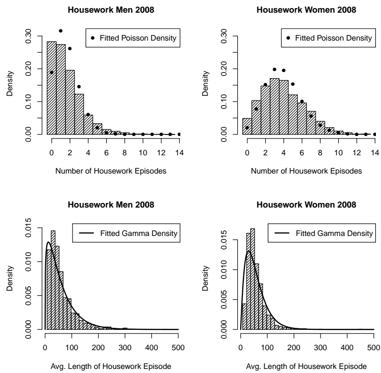
Figure 3.4: Distribution of the Number and Length of Housework Episodes: A Comparison with Fitted Poisson and Gamma Distribution
