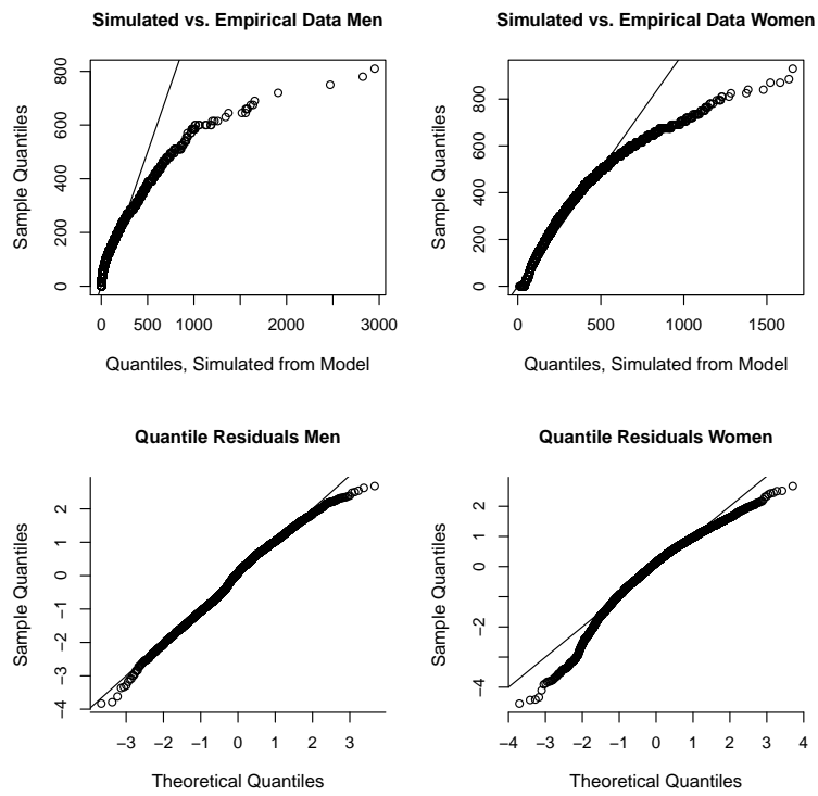
Figure 4.10: Housework: Evaluation of the Negative Binomial Model
