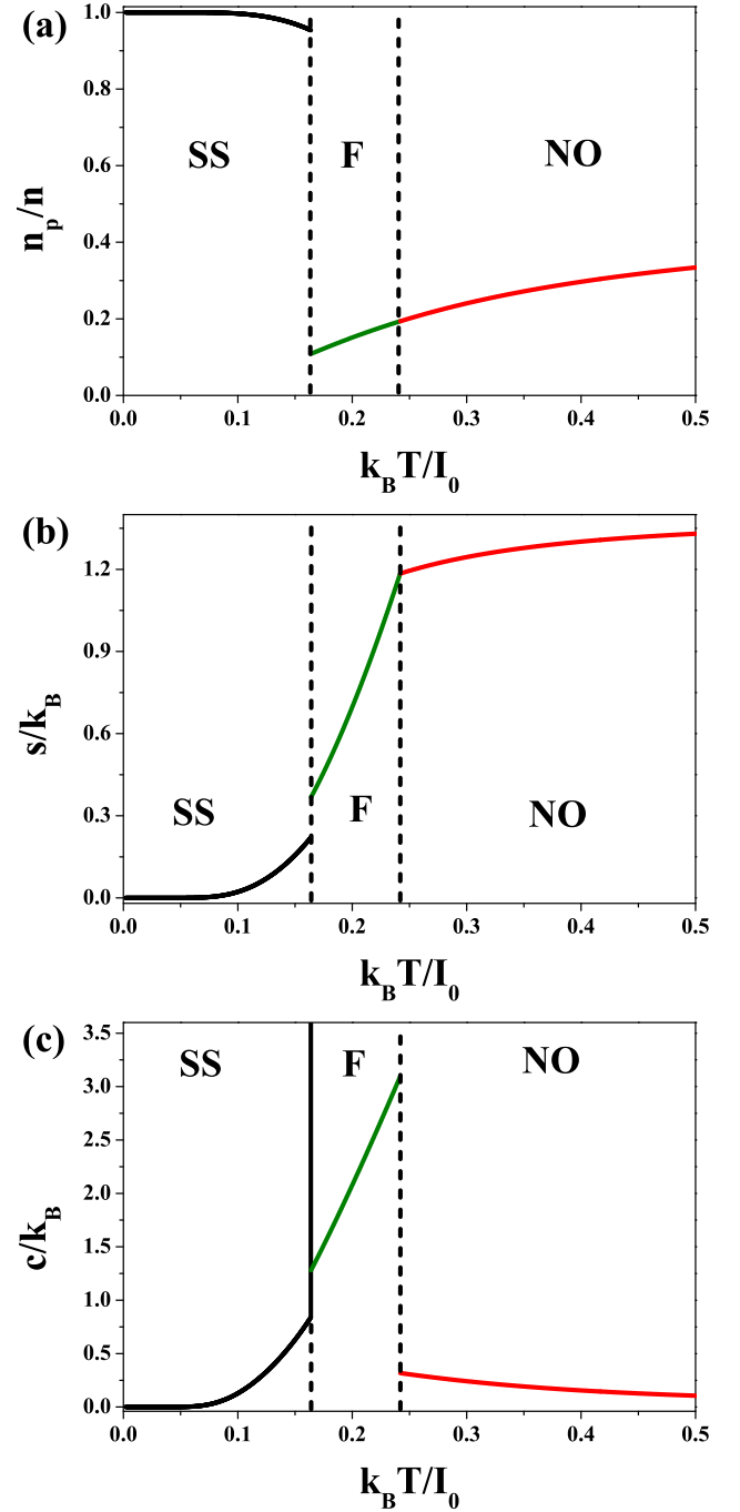
FIG. 3. (Color online) Thermodynamic parameters (a) the concentration of paired electrons n_p/n = 2D/n , (b) the entropy s and (c) the specific heat c as a function of k_B T/I_0 for J/I = 0.3 , U/I_0 = 0.69 and n = 1 .
