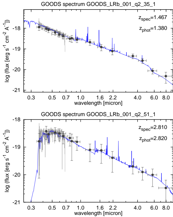
Figure 1.9: Examples of spectra for two galaxies at either side of the redshift range covered by the “redshift desert”. Observed spectra are shown as grey lines, observed photometric data-points and their respective uncertainties are shown with black circles; the blue solid line shows the best-fit spectrum obtained via the photometric redshift fitting.
