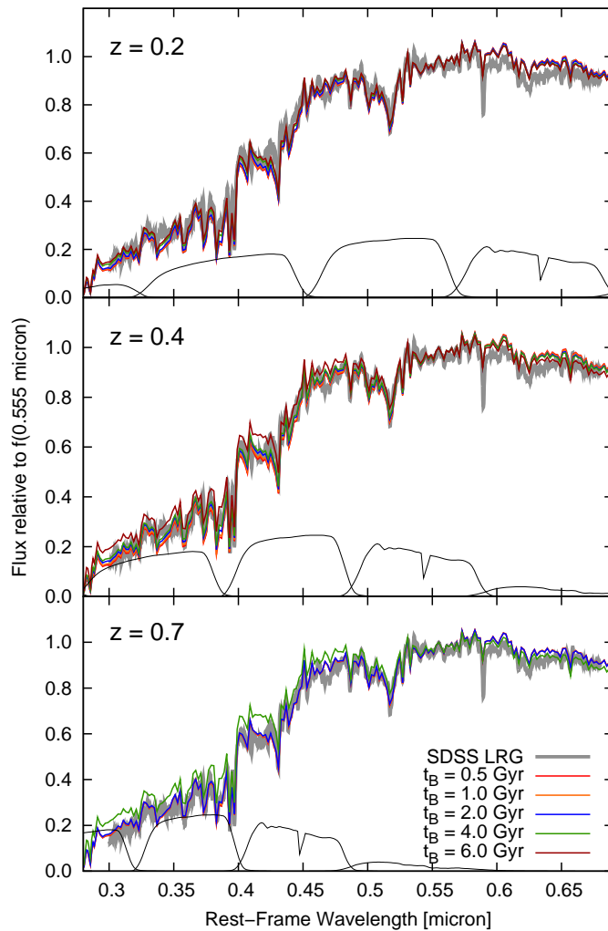
Figure 4.17: Spectra of post-starburst galaxies compared to the SDSS template spectrum for Luminous Red Galaxies (thick solid line). For reference we also show the SDSS ugriz-filters for each redshift.
