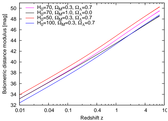
Figure C.16: Bolometric distance modulus as function of redshift for a range of cosmological parameter sets.
