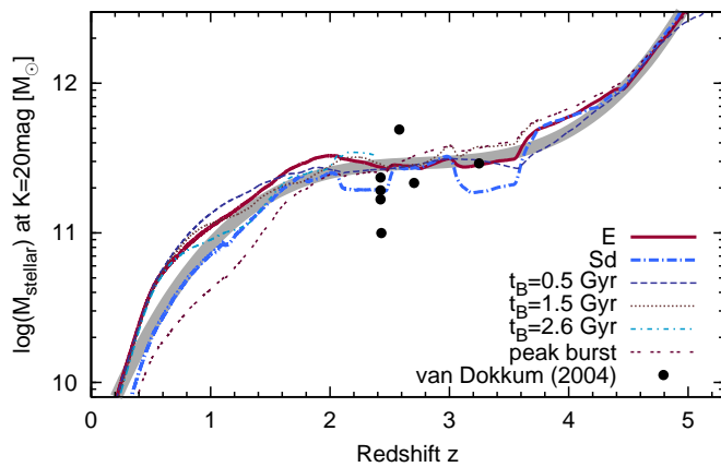
Figure 4.15: Stellar masses of galaxies with k = 20 mag and J - K = 2.3 mag for different models and, hence, star formation histories. The grey thick line shows a 3rd-order polynomial fit to the models (see text for parameters).
