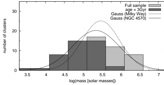
Figure A.7: Mass distribution of the GCs in NGC 4570. The light grey histogram is for all GCs from our sample, the dark one for the subsample of GCs younger than 3 Gyr. The solid line is a Gaussian fit to our unbinned GC mass distribution with a median of \log(\langle M_{GC}[M_{\odot}] \rangle) = 5.3 and \alpha(M_{GC}) = 0.6 dex, normalized to the number of GCs in our sample. The dotted line gives the Gaussian for the Milky Way GCs with \log(\langle M_{GC}[M_{\odot}] \rangle_{MW}) = 5.47 and \alpha_{MW}(M_{GC}) = 0.50 dex, normalized to the number of GCs in our sample.
