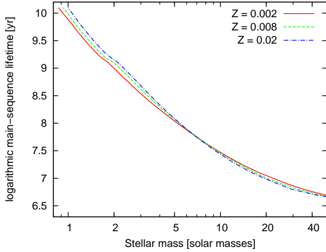
Figure 2.4: Main-sequence lifetimes as function of initial stellar mass for three different metallicities. Based on data from Bertelli et al. (1994).
