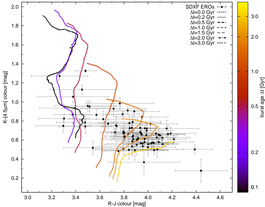
Figure 4.12: Novel two-colour diagnostic, based on R - J and K - [4.5\mu\text{m}] colours, to discriminate between dusty, actively star-forming EROs and passively evolving post-starburst EROs. Model tracks for redshifts z = 0.8 to 2.0 are shown with colours according to their respective burst age \Delta t , which is shown in the colour bar on the right-hand side of the plot. Data-points and error-bars are taken from the Subaru XMM-Newton Deep Field Survey (see text and Sect. 6.3.4 for details) and show colours of galaxies with 5.0 < R - K < 5.3 mag in the same redshift range as the models.
