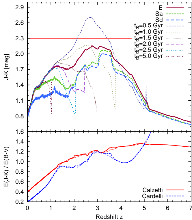
Figure 4.13: Upper part: (J - K)_{\text{Vega}} colour evolution of a representative part of our model grid. The solid horizontal marks the selection criterion for Distant Red Galaxies of J - K \geq 2.3 mag. Lower part: Extinction ratio E(J - K)/E(B - V) as function of redshift for two different choices of the extinction law.
