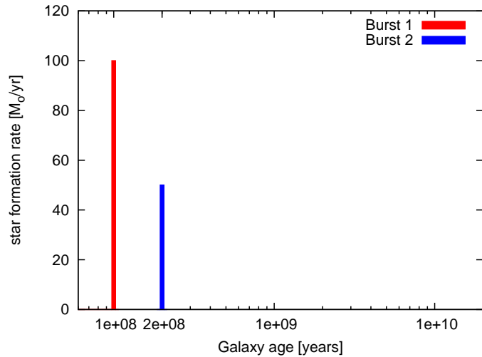
Figure C.9: For our toy-model we construct a very primitive star formation history of 2 bursts, with SFRs of 100 M_{\odot} \text{yr}^{-1} and 50 M_{\odot} \text{yr}^{-1} , each lasting 10^6 years.
