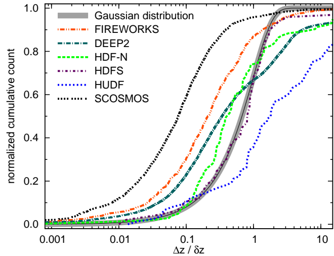
Figure 6.5: Cumulative distribution of \Delta z/\delta z (with \Delta z = |z_{\text{spec}} - z_{\text{phot}}| ; \delta z = (z_{\text{phot},+\sigma} - z_{\text{phot}}) for z_{\text{spec}} > z_{\text{phot}} and \delta z = (z_{\text{phot}} - z_{\text{phot},-\sigma}) for z_{\text{spec}} < z_{\text{phot}} ; z_{\text{phot},+\sigma} and z_{\text{phot},-\sigma} are the upper and lower 1\sigma extremities, respectively) for all galaxies in our sample with available spectroscopic redshift. For comparison we show the expected distribution in case of gaussian errors.
