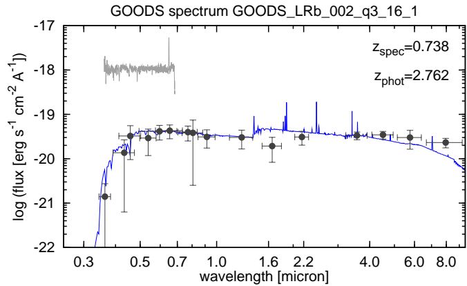
Figure 1.11: Same as Fig. 1.9, but for a case with discordant spectroscopic and photometric redshifts. For the observed spectrum, the redshift is supposedly based on the detection of the Mg II \lambda 2798 and [O II] \lambda 3727 lines.
