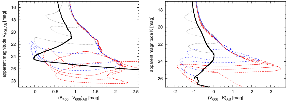
Figure 3.15: B-V (upper panel) and V-K (lower panel) colour evolution of all galaxy models in our model grid. The thick solid line gives the colour of the S b -type progenitors for comparison. All magnitudes are given in the AB system. Red lines show early bursts with t_B = (0.5, 1.0, 1.5) Gyr, blue are bursts at intermediate ages ( t_B = (2.0, 3.0, 4.5) ) and shown in grey are late bursts with t_B = (6.0, 9.0, 11.0) Gyr.
