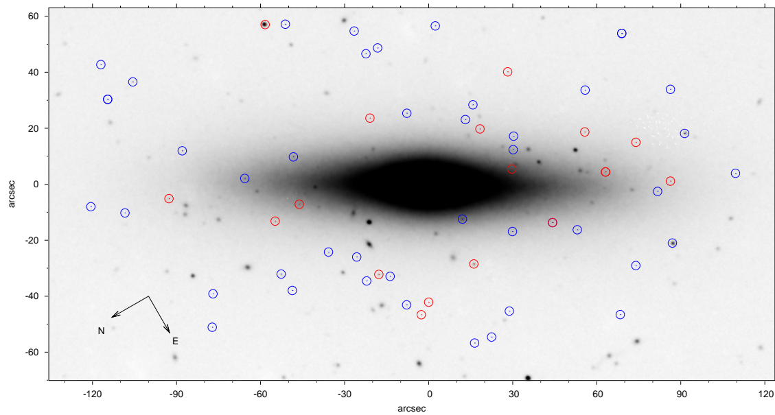
Figure A.5: Spatial distribution of our Globular Cluster sample, overlaid over our K-band image obtained with NTT/SOFI. Blue circles mark GCs with best-fit ages < 3 Gyr, while red circles mark GCs older than 3 Gyr. Most of the bright sources are either stars or (in most cases) background galaxies, that are resolved on the HST images.
