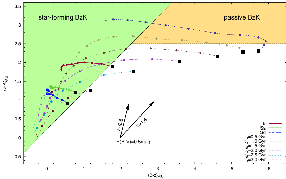
Figure 4.3: Colour selection scheme for BzK galaxies over-plotted with the part of our model grid that the BzK selection scheme aims at - galaxies with redshifts 1.4 \leq z \leq 2.5 . In the bottom middle of the plot we show reddening vectors for E(B - V) = 0.5 \text{ mag} for both extreme redshifts z = 1.4 and z = 2.5 . Large black squares mark the low-redshift end of the targeted redshift range at z = 1.4 . Thin lines mark the colour evolution of several models of Sb-progenitors undergoing a starburst with bs = 0.75 at a galaxy age of t_B .
