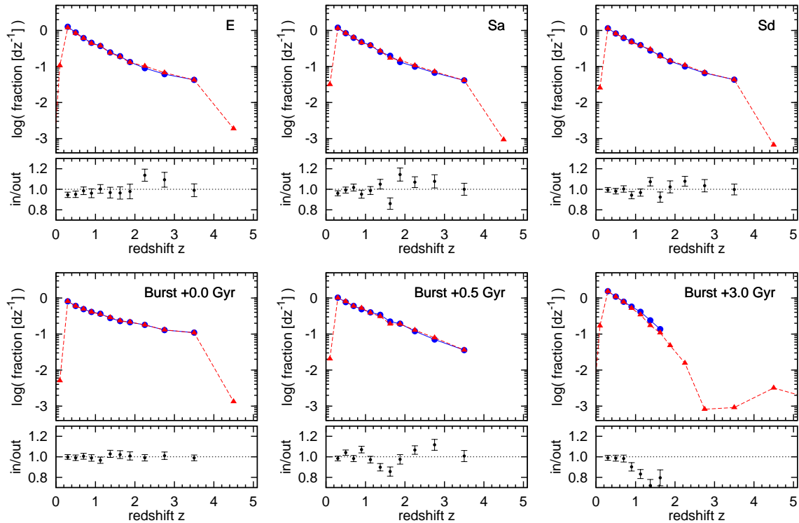
Figure 6.11: Results from our Monte-Carlo runs trying to explain the relative absence of galaxies in the redshift range z = 1.5 - 2 for six representative galaxy types (star formation histories) from our model grid. The top panels show, for each type, the input (blue circles) and the resulting redshift distribution after the photo- z fitting to the simulated photometry (red triangles). In the bottom panels we show the ratio between the number of galaxies in the output bin relative to the number of galaxies in the input catalog as a function of redshift. Error bars assume poissonian noise.
