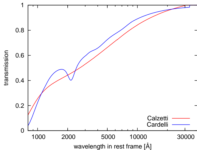
Figure C.12: Extinction curves from Calzetti and Cardelli. Both show very little transmission at short wavelengths indicating that most of the light gets absorbed.
