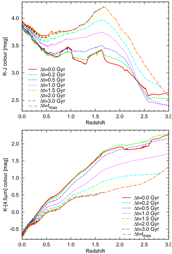
Figure 4.11: Colour evolution with redshift for several models with varying burst ages, ranging from the peak of star formation \Delta t = 0 Gyr to late post-starburst phases \Delta t = 3.0 Gyr. We also show the colour evolution of a maximally old post-starburst galaxy \Delta t = t_{\max} , encountering a burst with subsequent termination of star formation only 0.12 Gyr after its formation.
