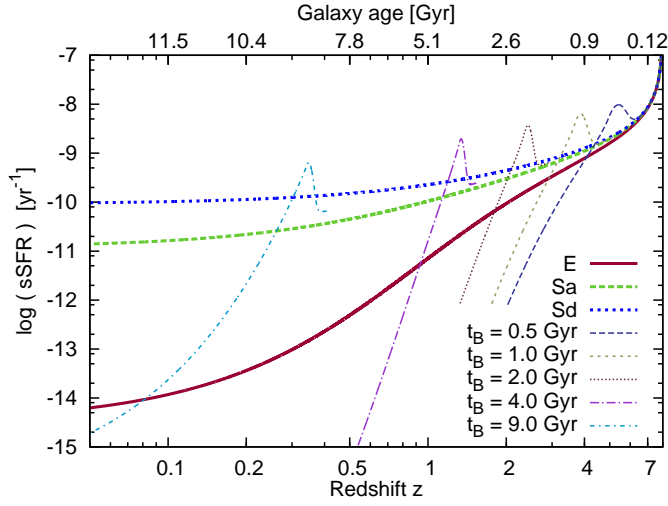
Figure 3.8: Specific star formation rates (sSFRs, = SFRM_{\text{stellar}}^{-1} ) for a range of undisturbed models (thick lines) and starburst models (thinner lines). Starburst models are only shown for ages after the onset of the burst. The top axis gives the corresponding galaxy age.
