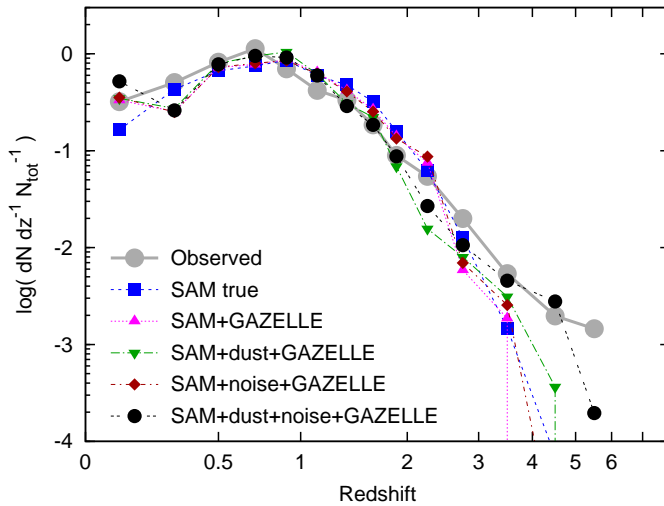
Figure 6.12: Comparison between the observed (thick grey line) projected density of galaxies per unit redshift, normalised by total number with the results from the artificial light-cones from Kitzbichler & White (2007) that are based on the Millennium simulation. The different lines represent results from different simulations also accounting for dust-extinction of photometric noise.
