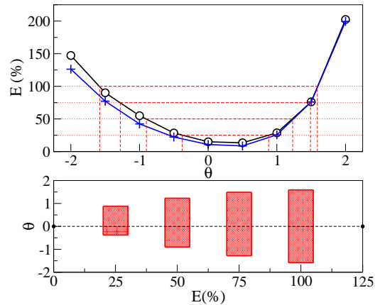
FIG. 2: (Color Online) Top: Average error as a function of \theta in quenched WN of size N = 10^4 and \gamma = 2.5 for the simple HMF estimate (circles), Eq. (23), and a more refined approximation (crosses), Eq. (27). Bottom: Range of \theta values yielding an average error E smaller than a given value for the HMF estimate.
