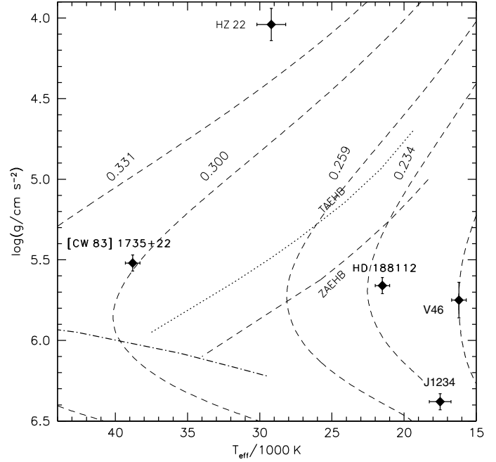
Fig. 20. T_{\text{eff}} - \log g -diagram similar to Fig. 2. The black filled diamonds mark the known post-RGB binaries HD 188112 (Heber et al. 2003), NGC 6121–V46 (V46 for short, O’Toole et al. 2006), HZ 22 (Schönberner 1978; Saffer et al. 1997) and SDSS J123410.37–022802.9 (J1234 for short, Liebert et al. 2004). The candidate post-RGB system [CW83] 1735+22 is included as well. The helium main sequence and the EHB-band are superimposed with post-RGB evolutionary tracks from Driebe et al. (1998) labelled by their masses.
