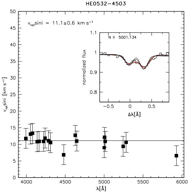
Fig. 6. Rotational broadening fit result for HE0532–4503 (see Fig. 4).
