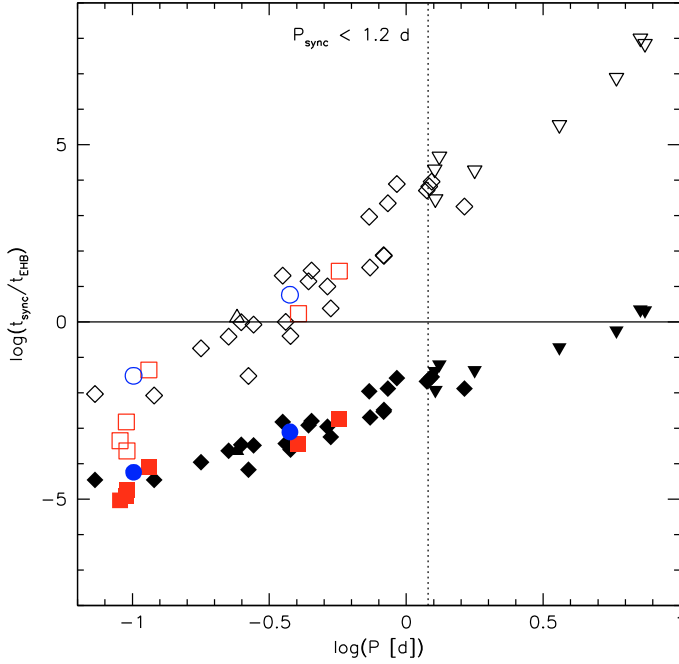
Fig. 19. Observed orbital period is plotted against the synchronization times of Zahn (1977, open symbols) and Tassoul & Tassoul (1992, filled symbols) both in units of the average lifetime on the EHB ( 10^8 yr, Dorman et al. 1993). The solid horizontal line marks the border between synchronization within the EHB lifetime and synchronization times longer than the EHB lifetime. The squares mark sdB binaries, where the primaries have been proven to be synchronized by light curve analysis of eclipsing or ellipsoidal variable systems. The circles mark binaries where synchronization could be shown by asteroseismology. The systems marked with diamonds could be solved consistently under the assumption of synchronization, while the systems marked with downward triangles rotate faster than synchronized. PG 2345+318 is the only sdB in our sample that rotates slower than synchronized. It is marked with an upward triangle.
