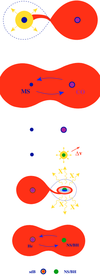
Fig. 17. Schematic diagram of formation scenarios leading to hot subdwarf binaries with neutron-star (left hand panel) or black-hole (right hand panel) companions.
