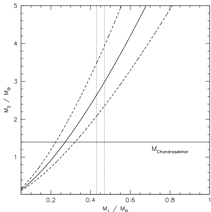
Fig. 11. Mass of the sdB primary HE 0532–4503 plotted against the mass of the unseen companion. The companion mass error is indicated by the dashed lines. The mass range of the CE ejection channel (Han et al. 2002) is marked with dotted vertical lines. The Chandrasekhar mass limit is plotted as solid horizontal line.
