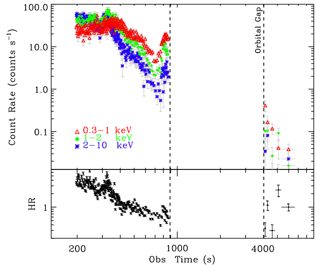
Figure 4. Upper panel: steep decay portion of GRB 081028 X-ray afterglow. The XRT signal has been split into 3 energy bands so that the different temporal behaviour can be fully appreciated. Lower panel: (0.3 - 1 \text{ keV}) / (1 - 10 \text{ keV}) hardness ratio evolution with time. The signal clearly softens with time. In both panels, the vertical black dashed lines mark the orbital data gap.
