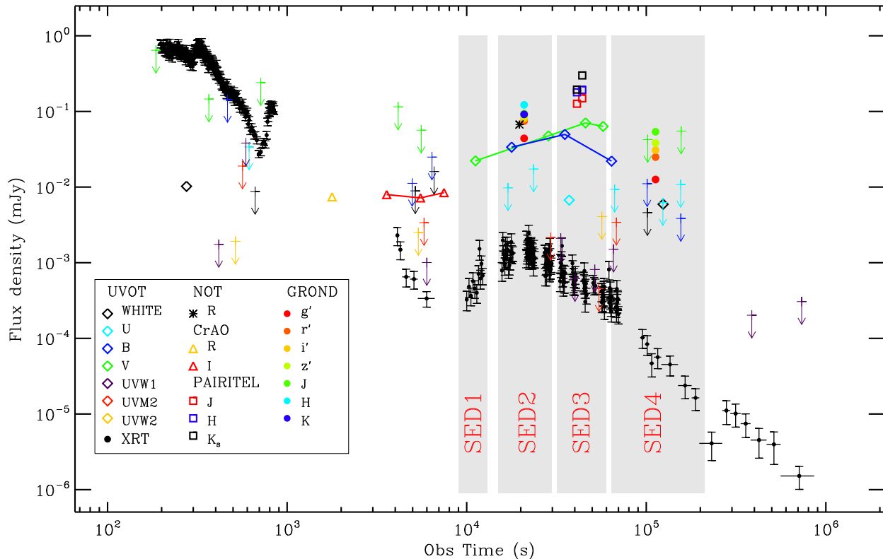
Figure 2. Complete data set for GRB081028 starting 200 s after the trigger including X-ray (XRT, flux density estimated at 1 keV), UV/visible/NIR (UVOT, GROND, PAIRITEL, CrAO, NOT) observations. The arrows indicate 3\text{-}\sigma upper limits of UVOT observations. The shaded regions indicate the time intervals of extraction of the SEDs.
