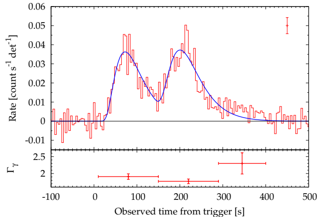
Figure 1. Top panel: BAT 15-150 keV mask weighted light-curve (binning time of 4.096 s). Solid blue line: 15 – 150 keV light-curve best fit using Norris et al. (2005) profiles. The typical 1 \sigma error size is also shown. Bottom panel: best fit photon index \Gamma_\gamma as a function of time (errors are provided at the 90% c.l.).
