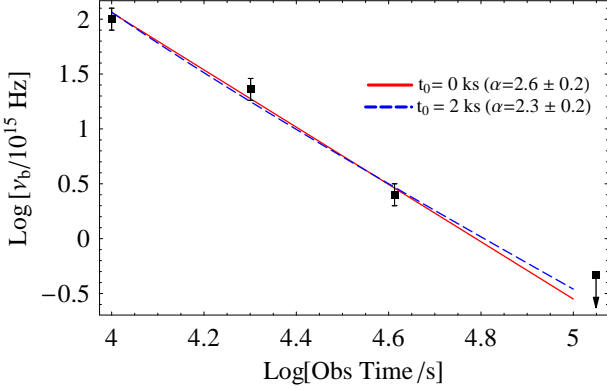
Figure 8. Spectral break frequency (See Eq. 3) evolution with time as found from a simultaneous fit of SED1, SED2, SED3 and SED4 with best fit models superimposed. Red solid line (blue dashed line): simple power-law with zero time t_0=0 ks (2 ks) and best power-law index \alpha = 2.6 (2.3). The satisfactory fit of SED4 with a simple power-law provides the upper limit shown.
