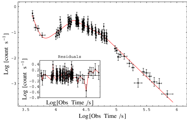
Figure 5. XRT 0.3-10 keV count-rate light-curve of GRB 081028 starting from 3 ks with best fit model superimposed (Eq. 2, Table 3). Inset: residuals with respect to the best-fit model.
