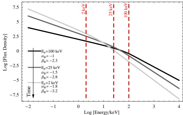
Figure 10. Qualitative description of the spectral evolution with time detected in GRB 081028 from the prompt to the steep decay phase: the peak energy ( E_p ) moves to lower energies while both the high and low energy components soften with time. Arbitrary flux density units are used.
