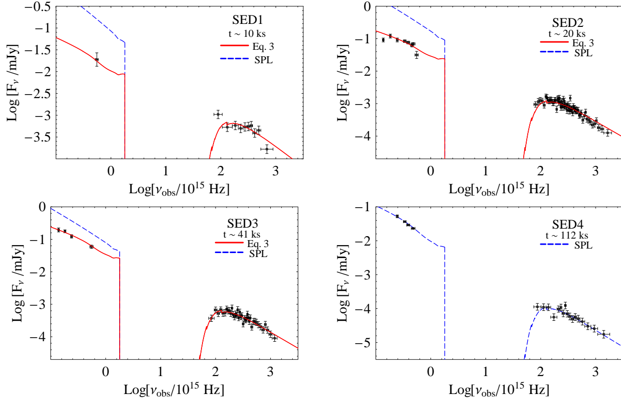
Figure 7. Observer-frame SED1, SED2, SED3 and SED4 from optical to X-ray extracted at t \sim 10 ks, t \sim 20 ks, t \sim 41 ks and t \sim 112 ks, respectively. Red solid line: photo-electrically absorbed model corresponding to Eq. 3. This proved to be the best fit model for SED1, SED2 and SED3. Blue dashed line: photo-electrically absorbed simple power law. This is the best fit model for SED4. For all SEDs an SMC extinction curve at the redshift of the source is assumed. The best fit parameters are reported in Table 4.
