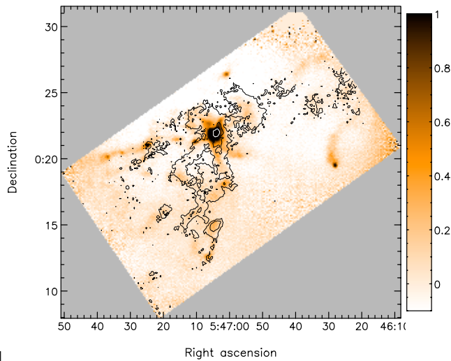
Figure 15. NGC 2071 SCUBA 850 \mu\text{m} map (Di Francesco et al. 2008), overlaid with \text{C}^{18}\text{O} integrated intensity contours. Contour levels are as in Fig. 6.
