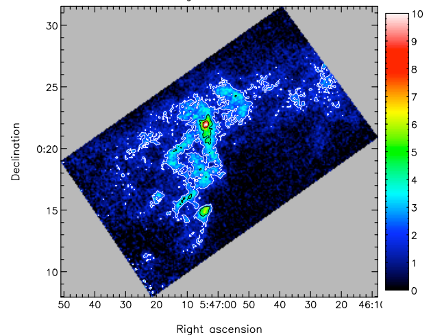
Figure 6. Integrated intensity images of ^{12}\text{CO} (top), ^{13}\text{CO} (middle) and \text{C}^{18}\text{O} (bottom) towards NGC 2071. Contours are ^{12}\text{CO} : 30,35 (white) and 45,65,105,185,345 (black) \text{K km s}^{-1} ; ^{13}\text{CO} 7,9 (white) and 11,15,21,29,39 (black) \text{K km s}^{-1} ; \text{C}^{18}\text{O} : 2 (white) and 4,7 (black) \text{K km s}^{-1} . The first \text{C}^{18}\text{O} contour is at 5\sigma .
