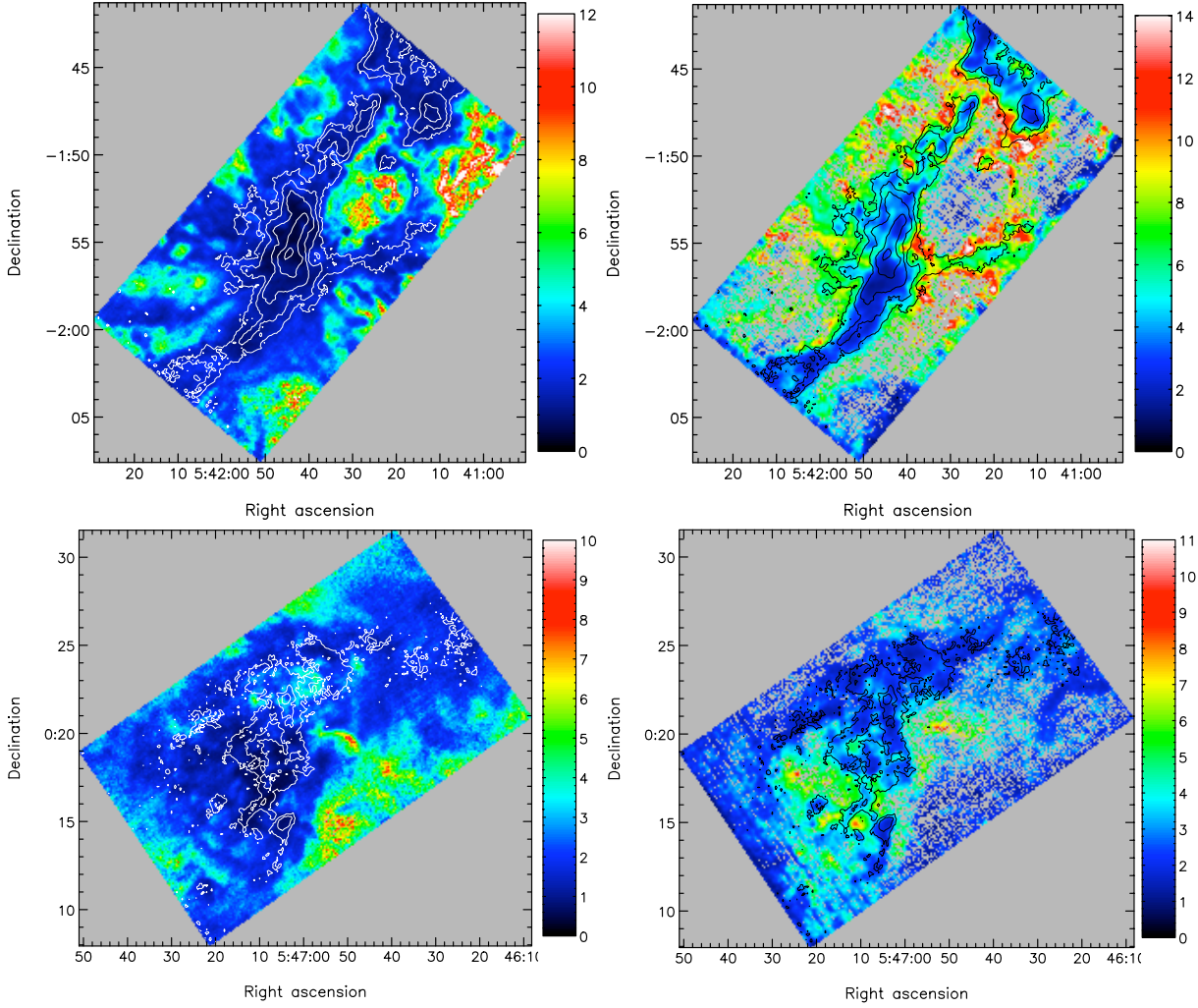
Figure 16. The ^{12}\text{CO}/^{13}\text{CO} (left) and ^{13}\text{CO}/\text{C}^{18}\text{O} (right) peak intensity ratios for regions with detections <3\sigma towards NGC 2024 (top) and NGC 2071 (bottom), overlaid with \text{C}^{18}\text{O} integrated intensity contours. The ^{13}\text{CO}/\text{C}^{18}\text{O} ratio data has been smoothed by a Gaussian with 12 arcsec FWHM to make the features more visible in these images.
