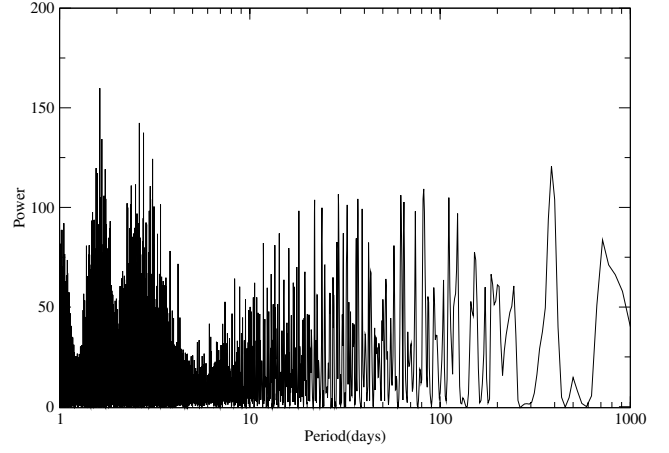
Fig. 8. Periodogram for H\alpha index.
