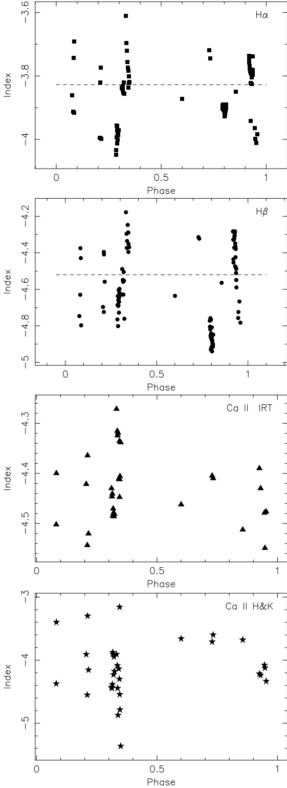
Fig. 7. Spectroscopic index for chromospheric activity indicators, phased folded orbital period. From top to bottom: H\alpha (squares), H\beta (circles), Ca II IRT (triangles) and Ca II H & K (stars). The dashed line is indicating the quiescent state. Error bars for indices are about 0.001.
