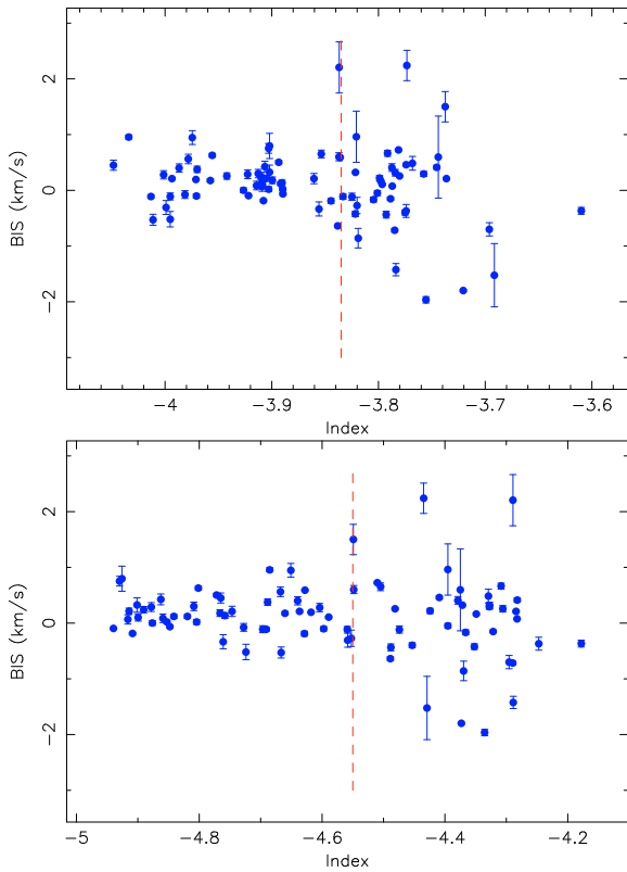
Fig. 12. Up: H\alpha index vs. BIS. The dashed line indicates the quiescent state. Down: H\beta index vs. BIS. Error bars for the indices are about of 0.001.
