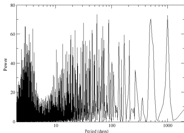
Fig. 6. Periodogram for bisectors of all runs.
