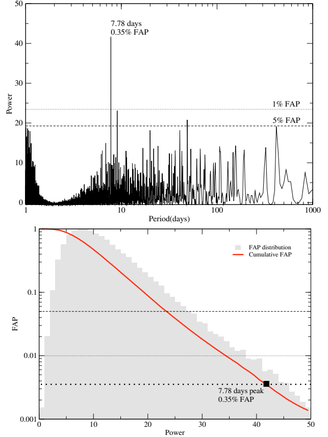
Fig. 4. Up: Least-squares periodogram of the nightly averaged radial velocity measurements. The 7.78 days peak has a FAP of 0.35%. The dotted horizontal line illustrates a FAP lower than 1% and the dashed horizontal line a FAP lower than 5%. Down: Empirical FAP as a function of the power (red line). The grey bars illustrate the distribution of false alarms with an arbitrary normalization used to derive the empirical FAP. The Y axis is on a logarithmic scale.
