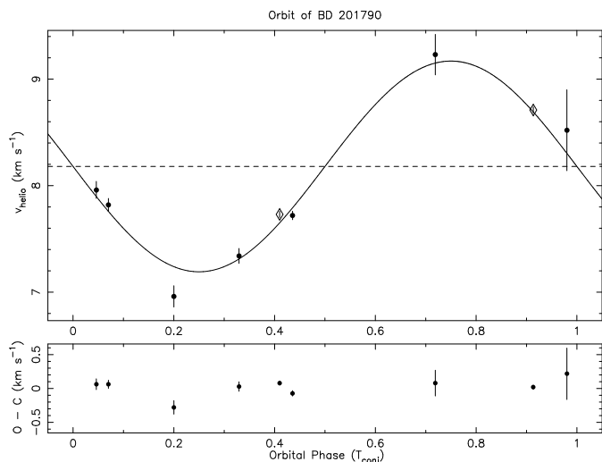
Fig. 14. Radial velocity variation of BD+20 1790 computed considering only the data that are not affected by flares. Circle symbols represent FOCES runs except that stars represent DDT FOCES 08B run. Diamond symbols are for SARG runs.
