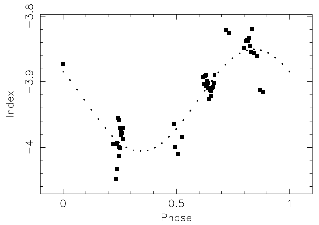
Fig. 9. H\alpha index for the data without flare events, including a modulation with a period of about 2.77 days, similar to the photometric period.
