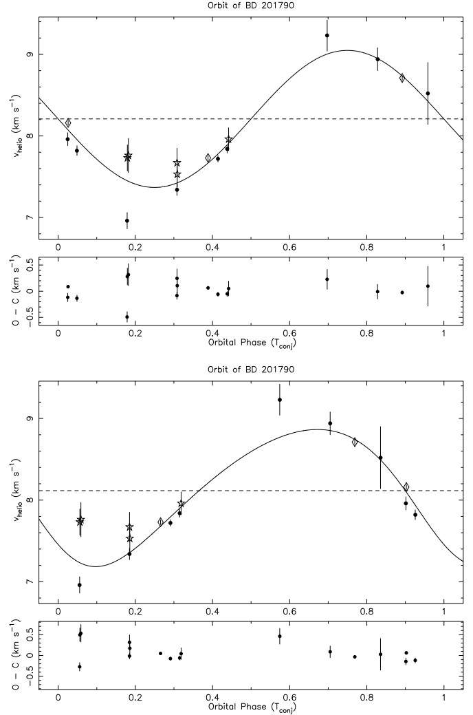
Fig. 13. Radial velocity variability of BD+20 1790. Up: Circular orbit. Down: Eccentric orbit. Values marked with circle symbol represent FOCES runs except stars that represent DDT FOCES 08B run. Diamond symbols are for SARG runs.
