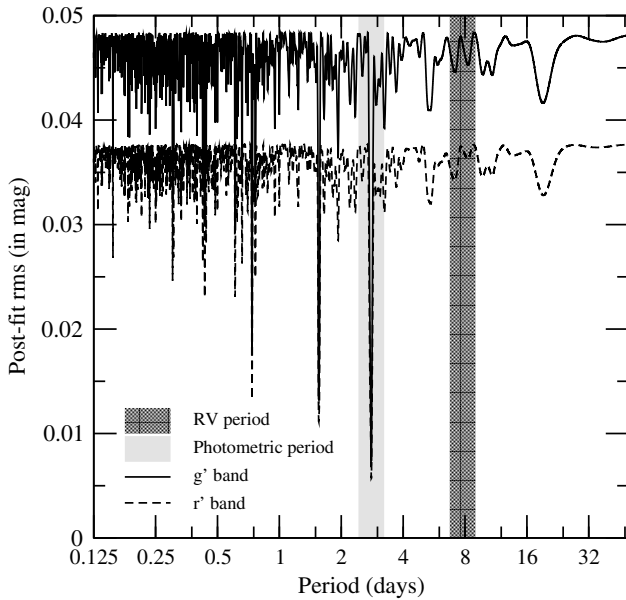
Fig. 3. Postfit residuals to the photometry as a function of the period. The sharper minima correspond to the 2.801 day period in both bands. The RVs period is marked in grey to illustrate the absence of related photometric signals.
