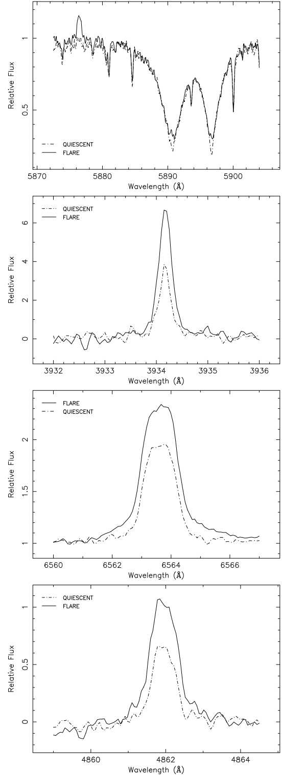
Fig. 1. Chromospheric activity indicators. The dashed line indicates quiescent state, while solid line indicates flare state. From top to bottom: He I D 3 region, Ca II K, H \alpha , and H \beta
