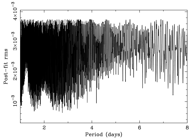
Fig. 10. Postfit residuals to H\alpha index for no-flare data as a function of the period.
