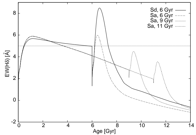
Figure 5. Time evolution of EW(H\delta) in galaxies with different burst scenarios (Sa, burst of 70% at 6 Gyr, decline time 0.1 Gyr; Sd, burst of 70% at 6 Gyr, decline time 0.1 Gyr; Sa, burst of 70% at 11 Gyr, decline time 0.1 Gyr).
