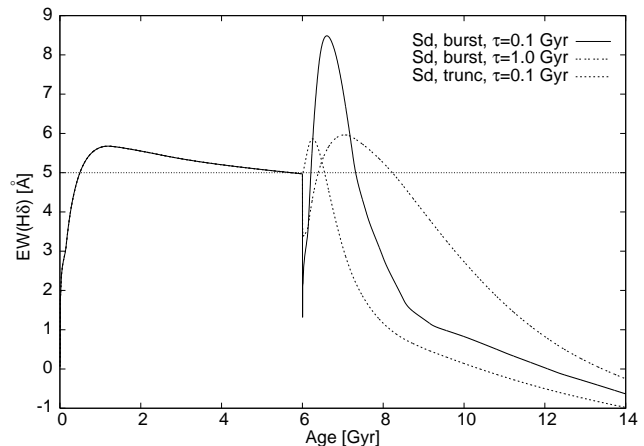
Figure 6. Time evolution of EW(H\delta) in galaxies with different burst scenarios (Sd, burst of 70% at 6 Gyr, decline time 0.1 Gyr; Sd, burst of 70% at 6 Gyr, decline time 1.0 Gyr; Sd, truncation at 6 Gyr, decline time 0.1 Gyr).
