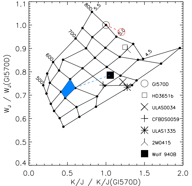
Figure 9. W_J versus K/J indices for a grid of solar metallicity BT-Settl model spectra. The grid is normalised such that the model values for the T_{\text{eff}} and \log g of G1 570D lie at coordinates (1,1). All observed values of W_J and K/J are shown as a proportion of those of G1 570D. We have indicated, with a red dotted line and open circle, the relative shift in position on the grid associated with increasing metallicity by +0.1 dex. Uncertainties are of similar size to the symbols. The blue dotted line highlights the difference between the true properties of Wolf 940B, and those expected from the model grid.
