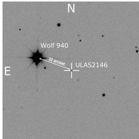
Figure 1. A 2'x2' J -band finding chart for ULAS 2146 taken from the UKIDSS database.
